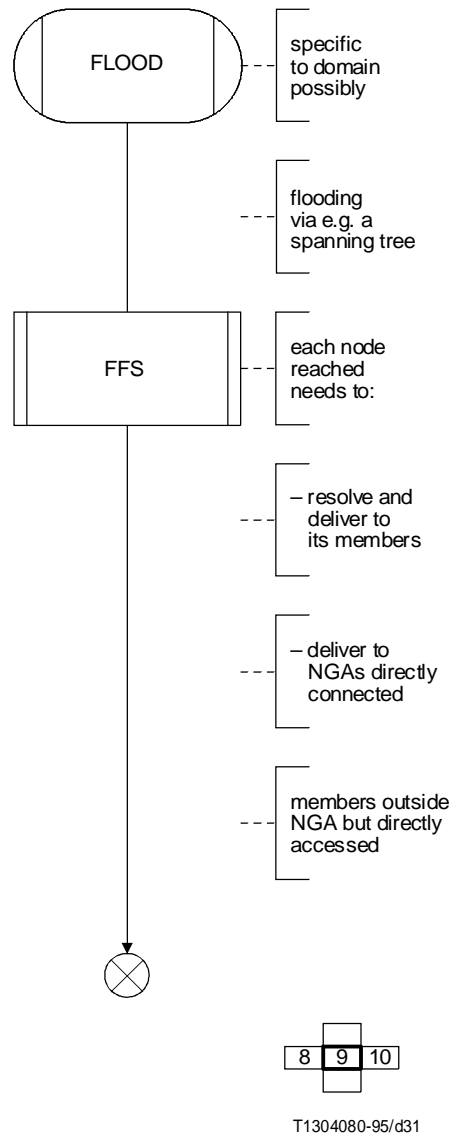
FIGURE II.4/I.364 (sheet 9 of 15)
