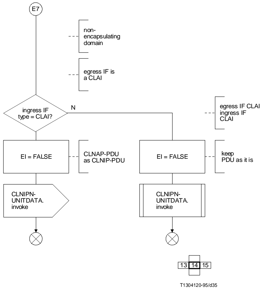
FIGURE II.4/I.364 (sheet 13 of 15)
