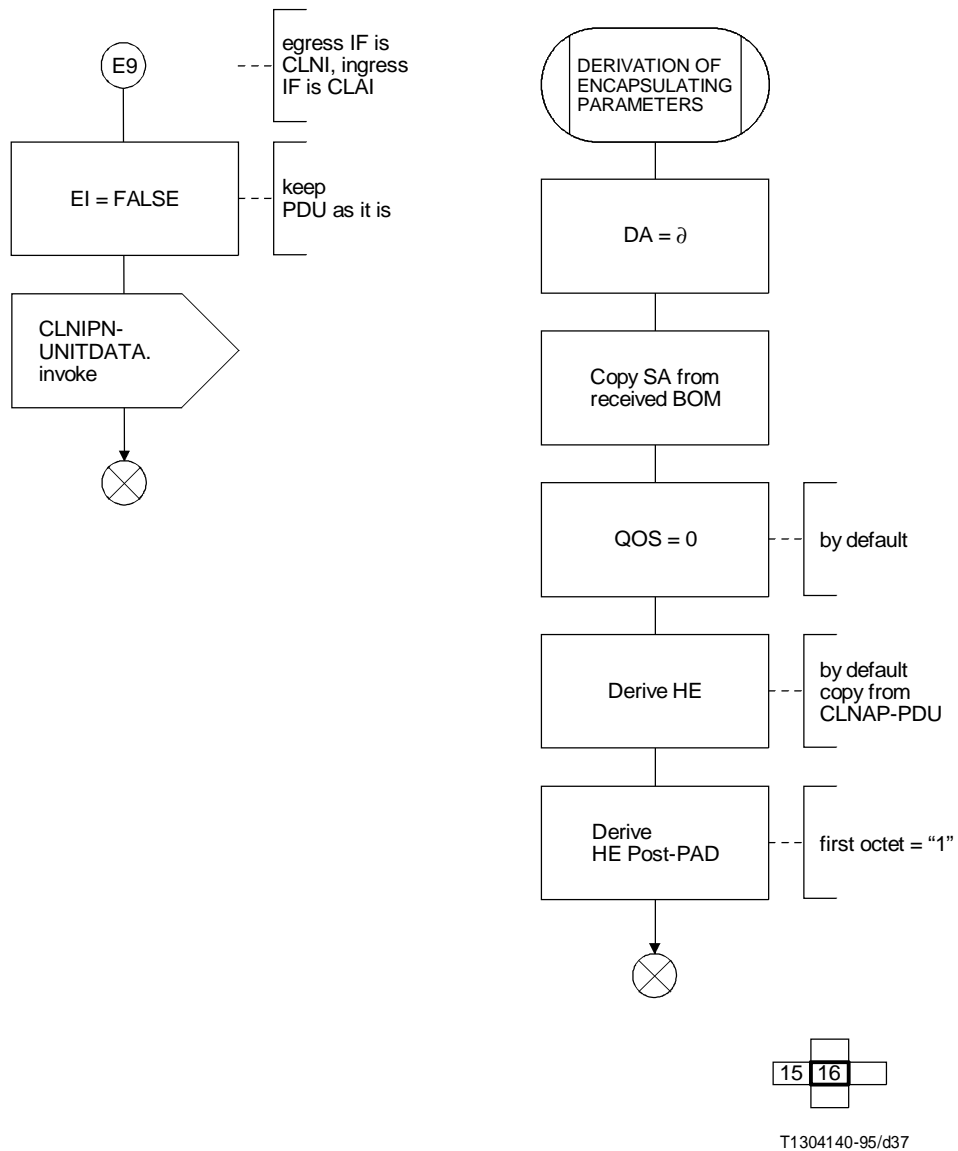
FIGURE II.4/I.364 (sheet 15 of 15)
