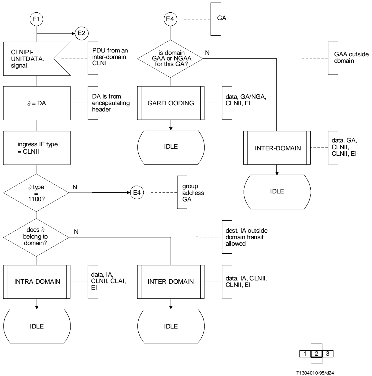
FIGURE II.4/I.364 (sheet 2 of 15)
