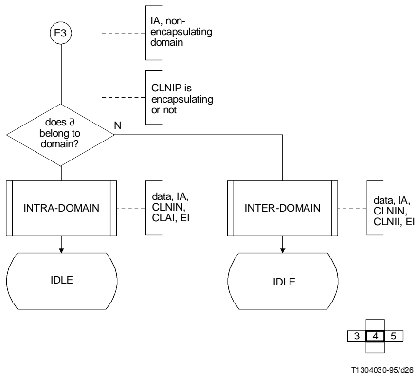
FIGURE II.4/I.364 (sheet 4 of 15)
