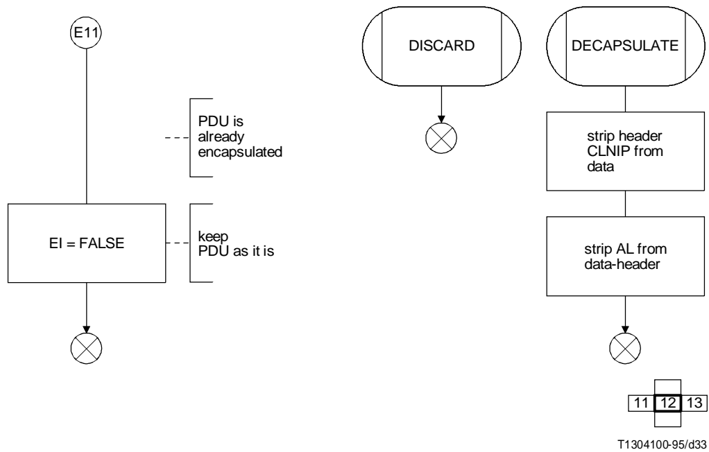
FIGURE II.4/I.364 (sheet 11 of 15)
