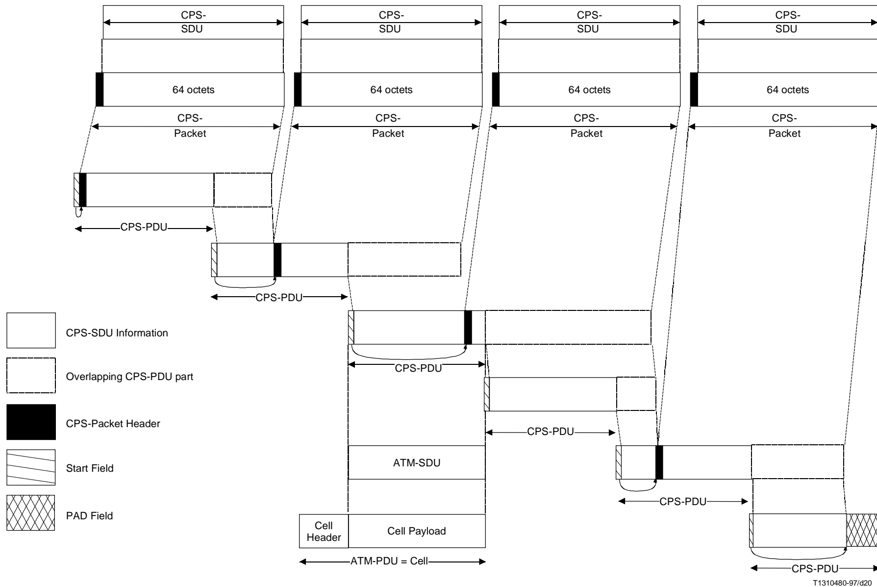
Figure I.3/I.363.2 – Multiplexing and packing of maximum size CPS-Packets into CPS-PDUs (ATM cells)
