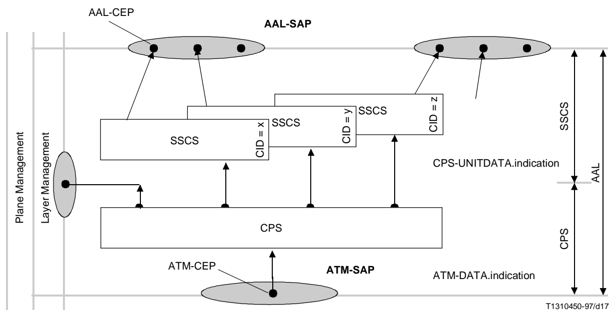
Figure B.2/I.363.2 – Functional model for the receiver of the AAL type 2
