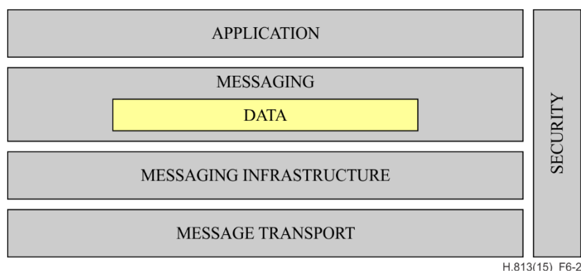
Figure 6-2 – Architecture
