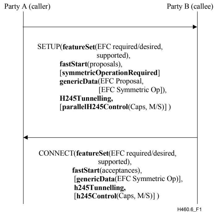
Figure 1/H.460.6 – Initial Extended Fast Connect exchange
