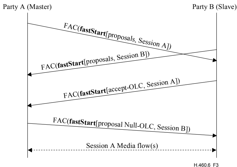
Figure 3/H.460.6 – Conflict resolution
