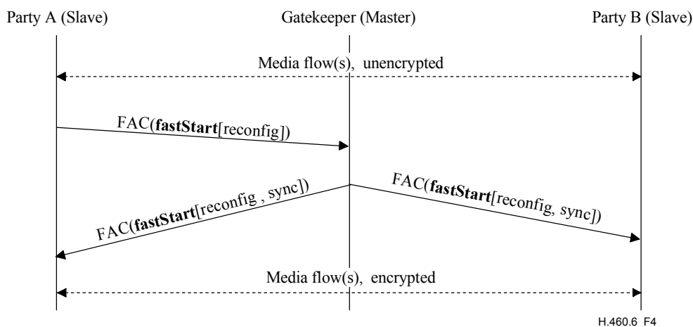
Figure 4/H.460.6 – Rekeying by the master
