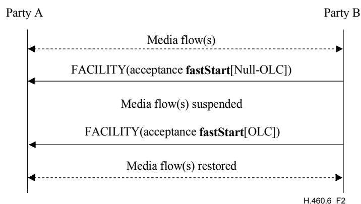
Figure 2/H.460.6 – Media stream idle and restore
