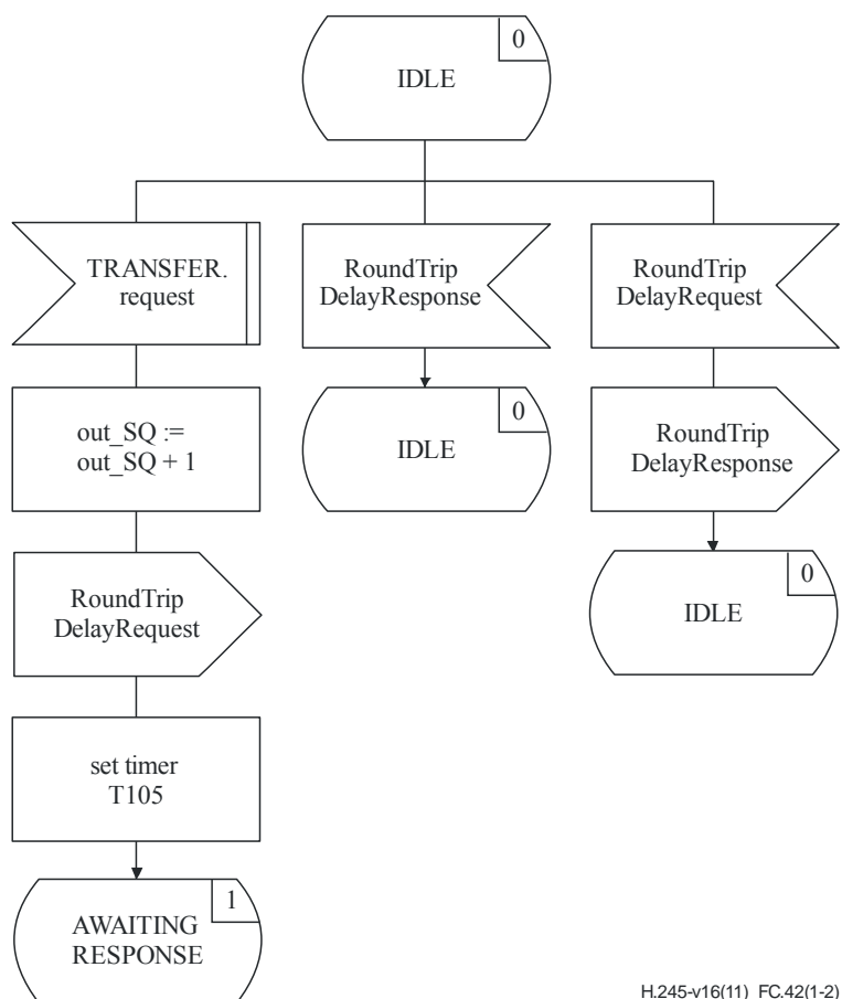
Figure C.42 – RTDSE SDL (sheet 1 of 2)
