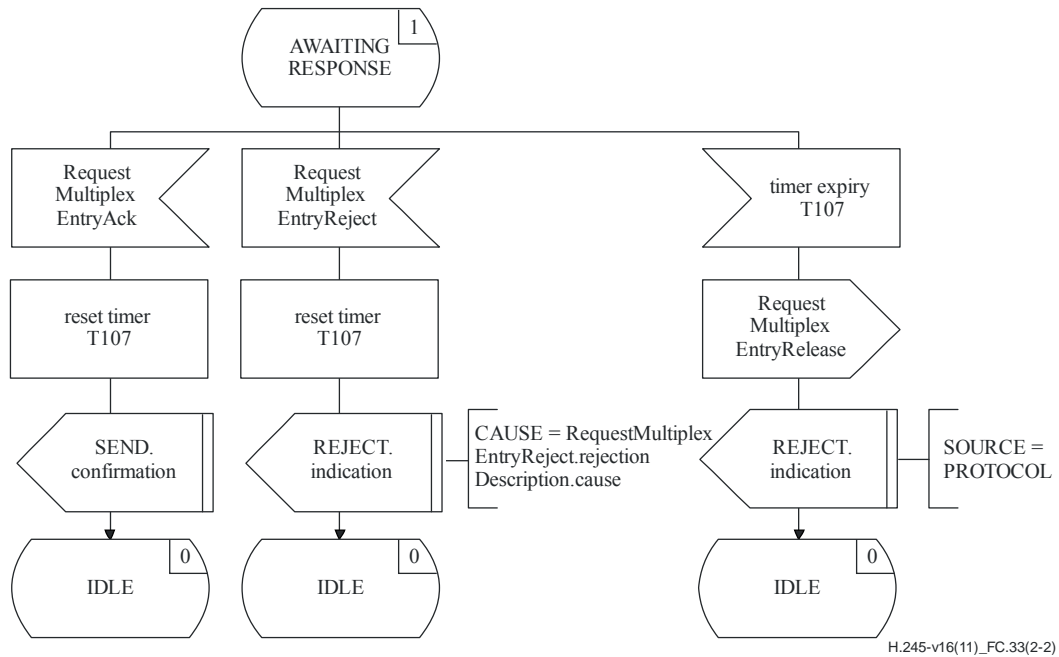
Figure C.33 – Outgoing RMESE SDL (sheet 2 of 2)
