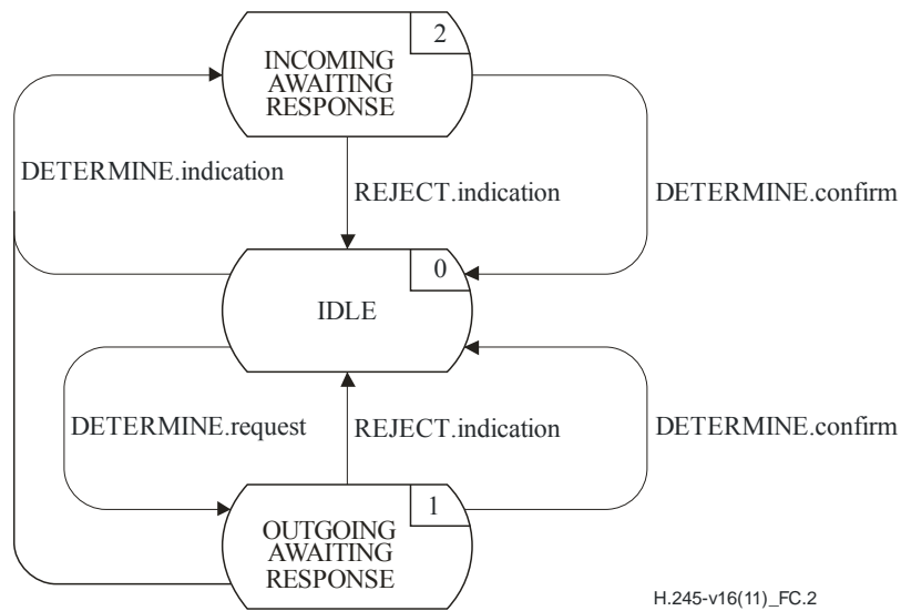
Figure C.2 – State transition diagram for sequence of primitives at MSDSE
