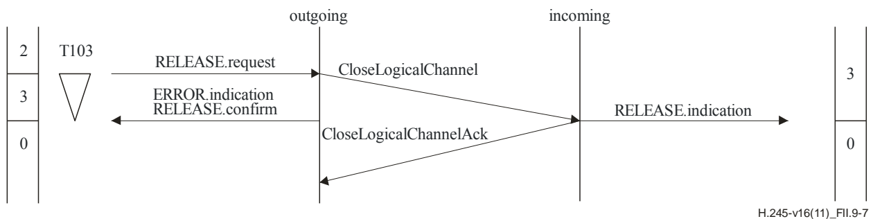
Figure II.9-7 – Bidirectional logical channel release request with expiry of timer T103 at the outgoing side
