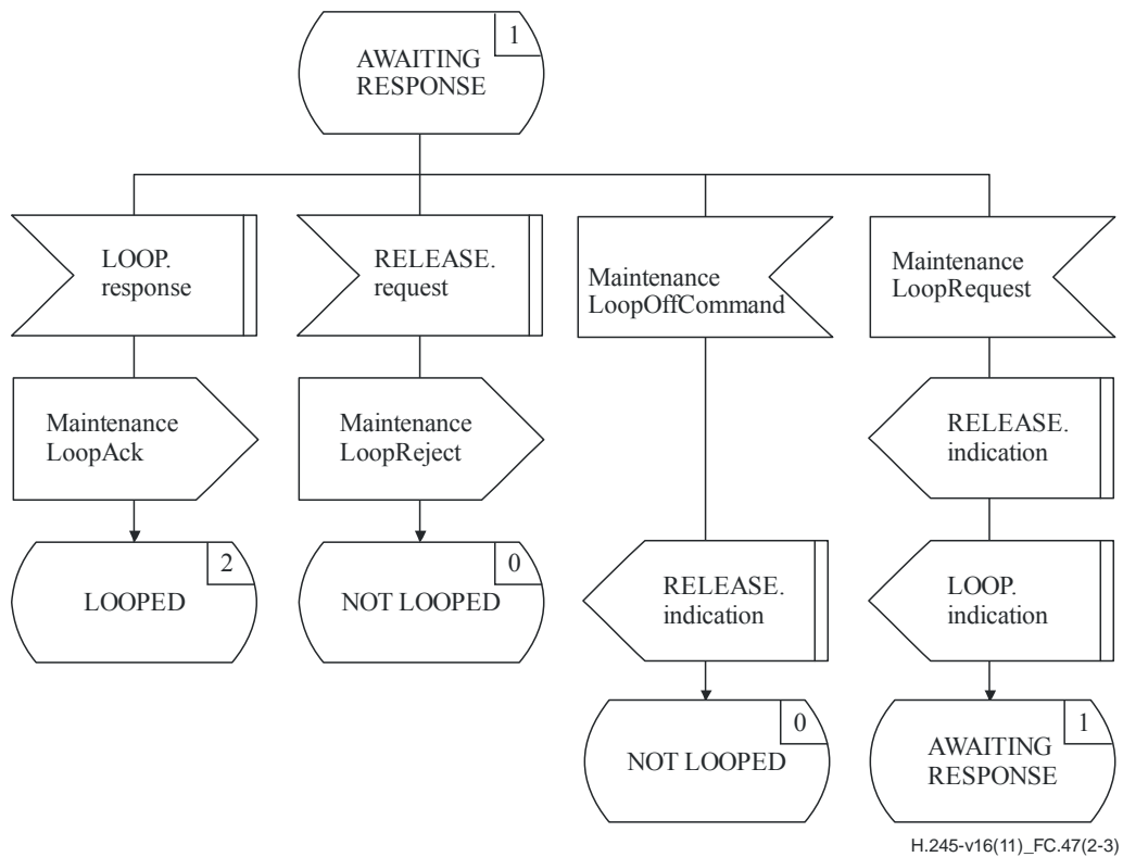
Figure C.47 – Incoming MLSE SDL (sheet 2 of 3)
