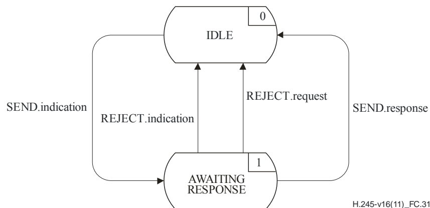
Figure C.31 – State transition diagram for sequence of primitives at incoming RMESE
