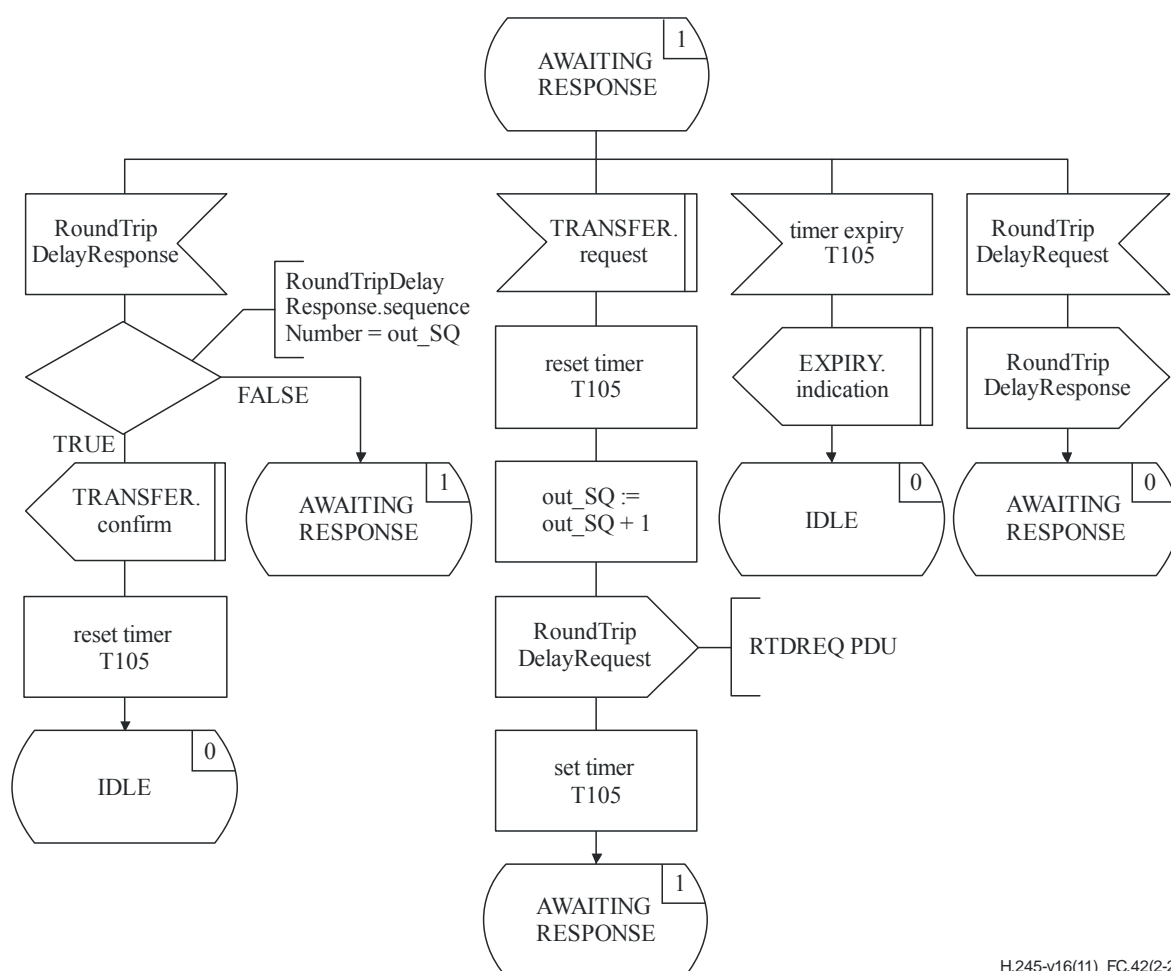
Figure C.42 – RTDSE SDL (sheet 2 of 2)
