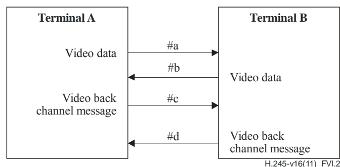
Figure VI.2 – Logical Channels for Separate Logical Channel Mode
