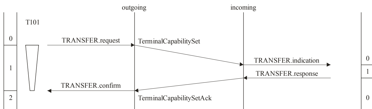
Figure II.3-1 – Capability exchange with acceptance from the peer incoming CESE user
