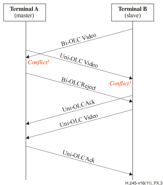
Figure X.3 – Master proposes unidirectional OLC and slave proposes bidirectional OLC
