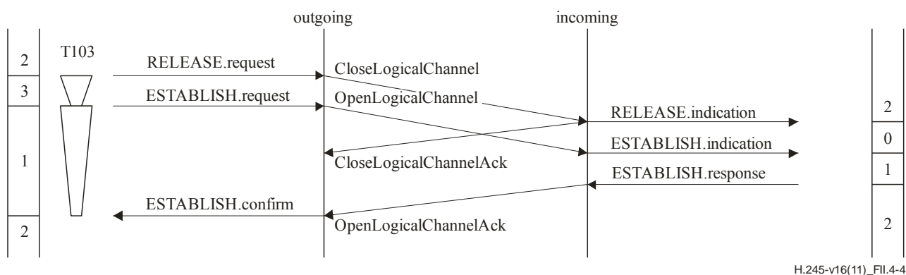
Figure II.4-4 – Logical channel release followed by immediate re-establishment
