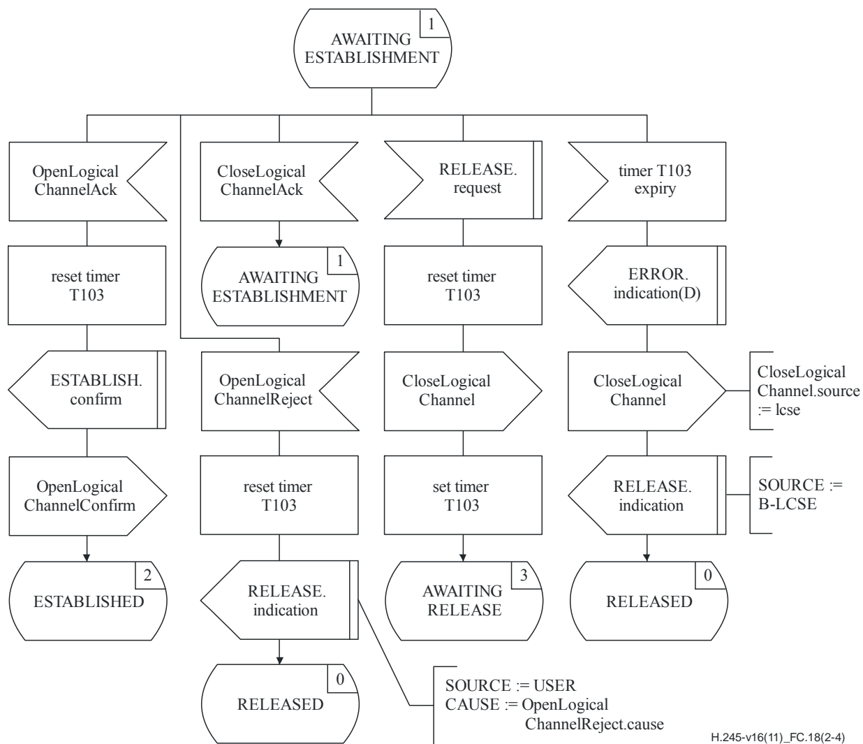
Figure C.18 – Outgoing B-LCSE SDL (sheet 2 of 4)
