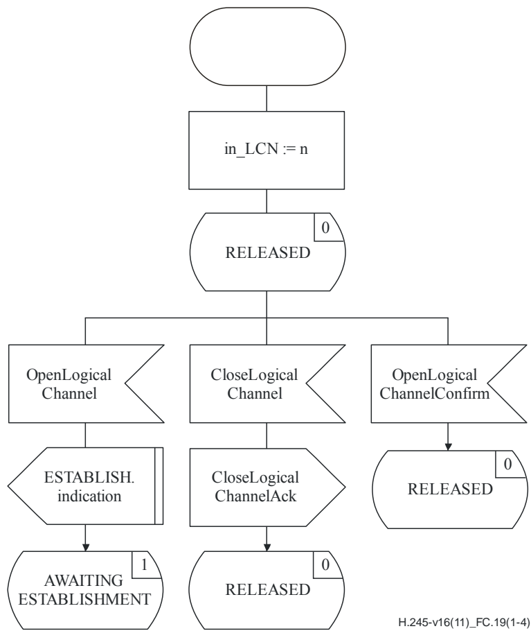
Figure C.19 – Incoming B-LCSE SDL (sheet 1 of 4)
