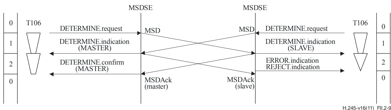
Figure II.2-9 – Master-slave determination – Simultaneous determination procedures with timer T106 expiry during INCOMING AWAITING ACKNOWLEDGEMENT
