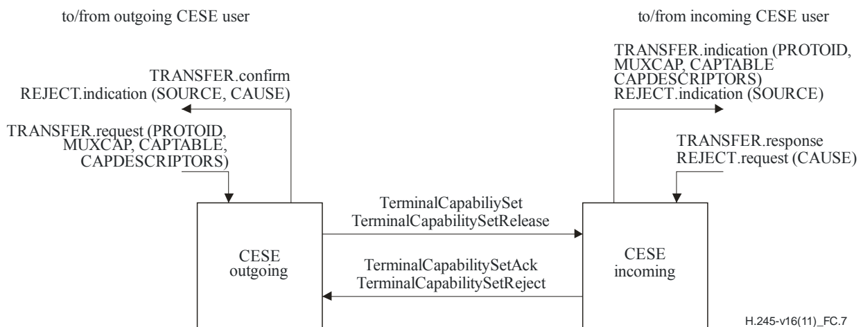
Figure C.7 – Primitives and messages in the Capability Exchange Signalling Entity
