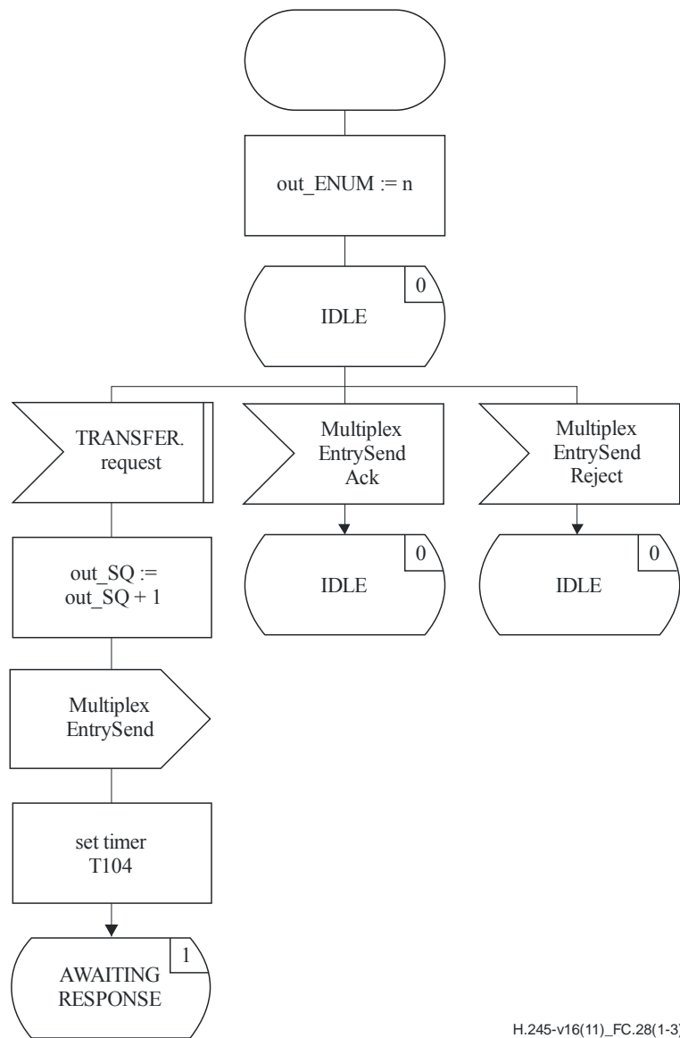
Figure C.28 – Outgoing MTSE SDL (sheet 1 of 3)
