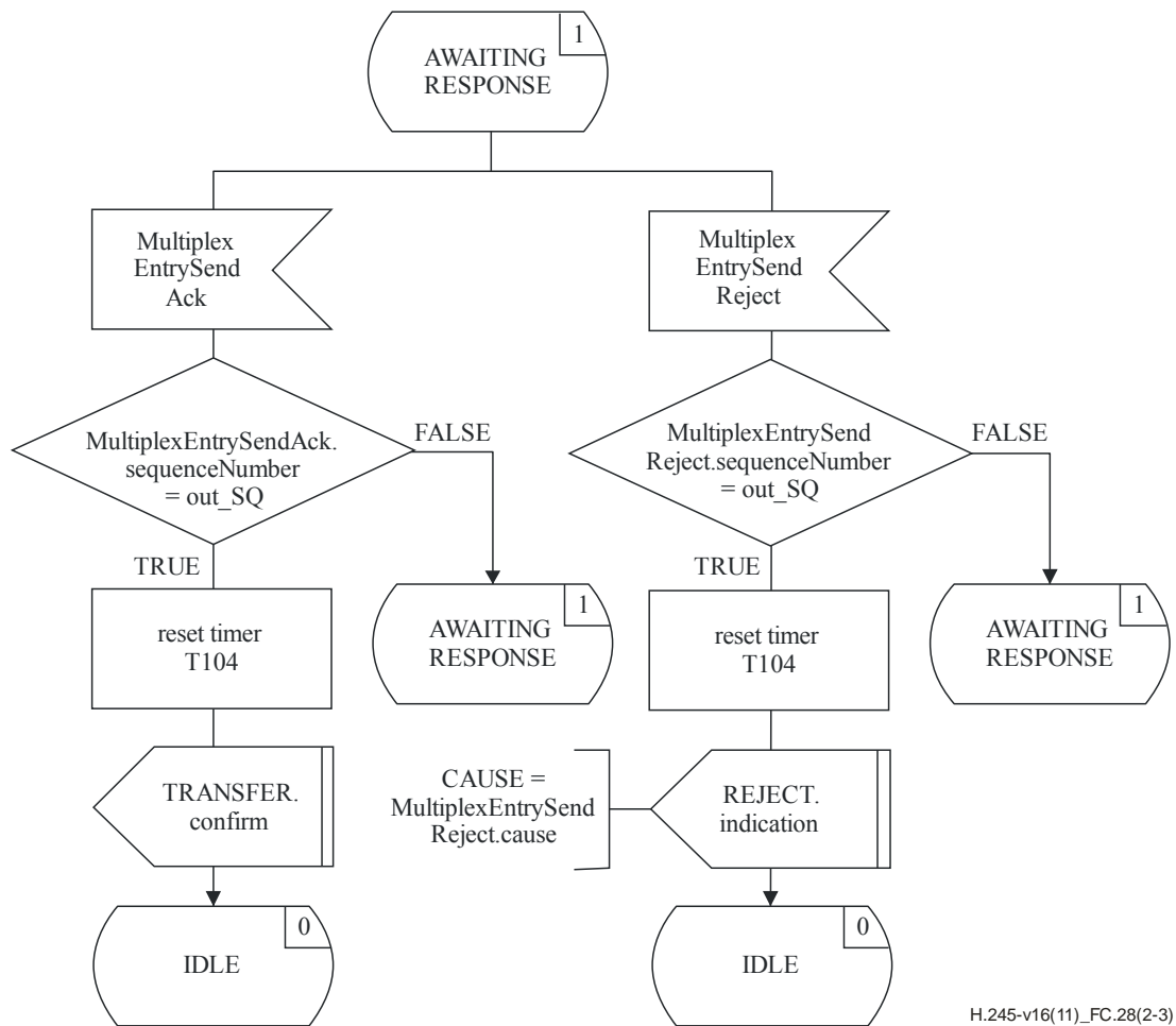
Figure C.28 – Outgoing MTSE SDL (sheet 2 of 3)
