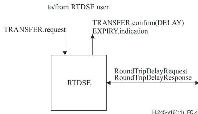
Figure C.41 – Primitives and messages in the RTDSE
