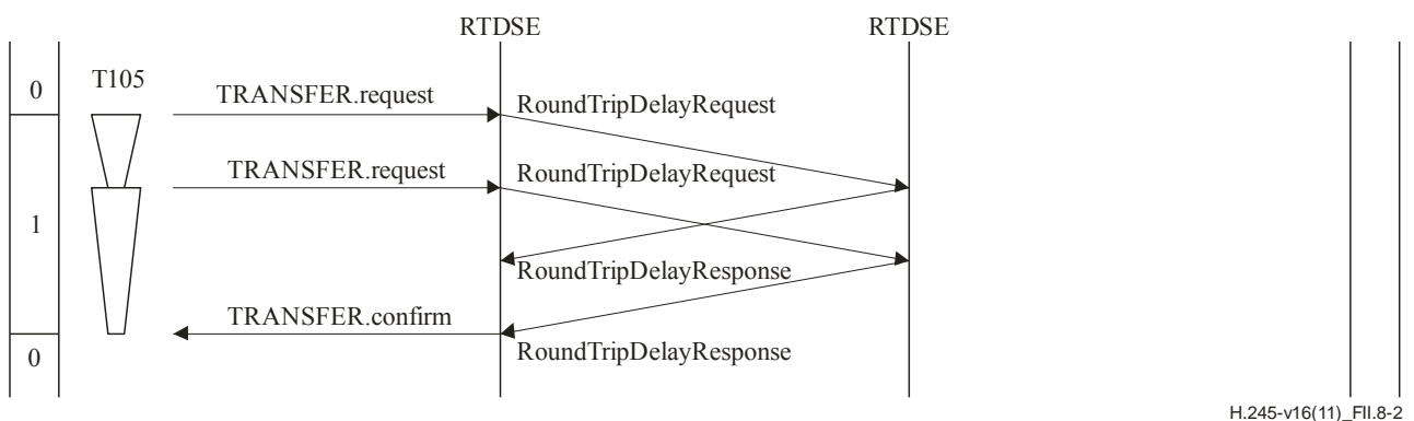
Figure II.8-2 – Round-trip delay determination procedure with an earlier unacknowledged round-trip delay procedure outstanding
