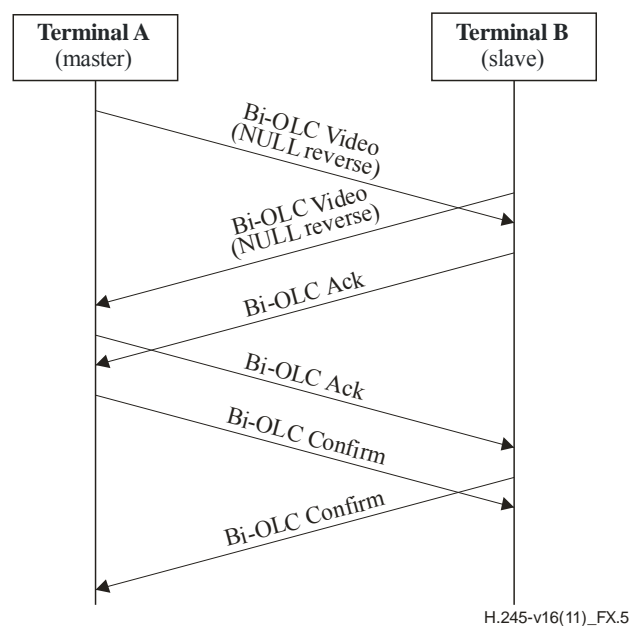
Figure X.5 – Both terminals propose bidirectional OLC with nullData
