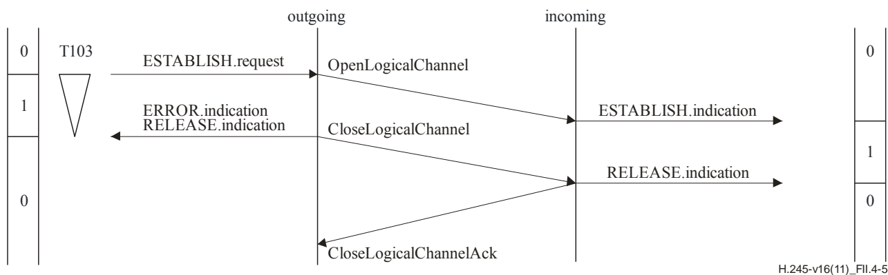
Figure II.4-5 – Logical channel establishment request with expiry of timer T103 due to slow response from peer incoming LCSE user
