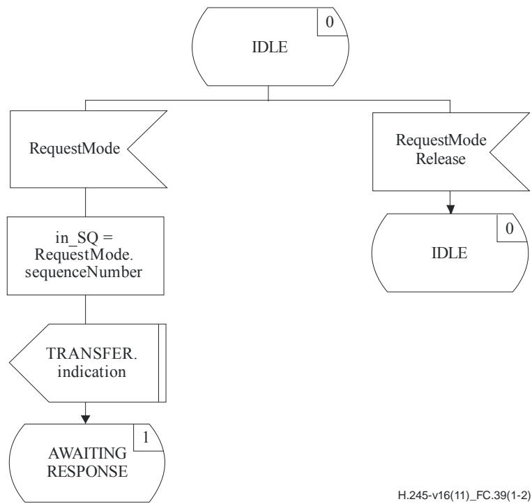
Figure C.39 – Incoming MRSE SDL (sheet 1 of 2)
