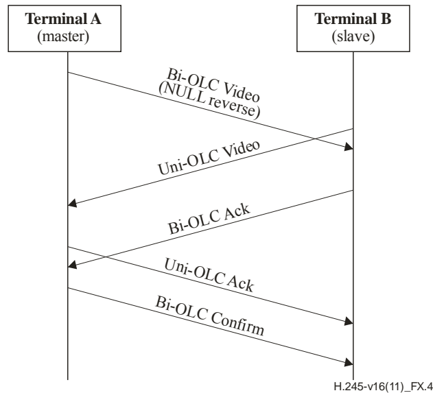
Figure X.4 – Master proposes bidirectional OLC with nullData and slave proposes unidirectional OLC
