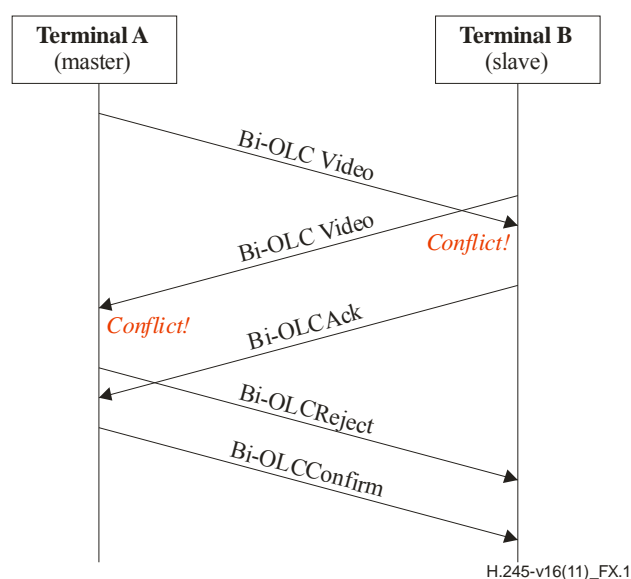
Figure X.1 – Both terminals use bidirectional OLC
