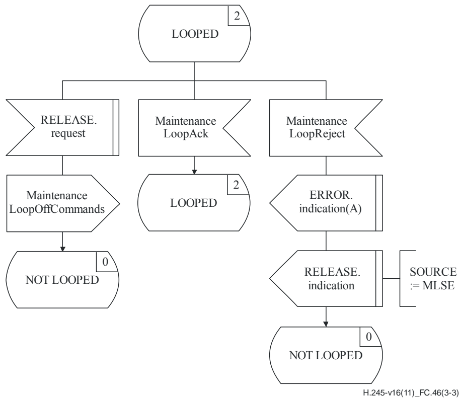
Figure C.46 – Outgoing MLSE SDL (sheet 3 of 3)
