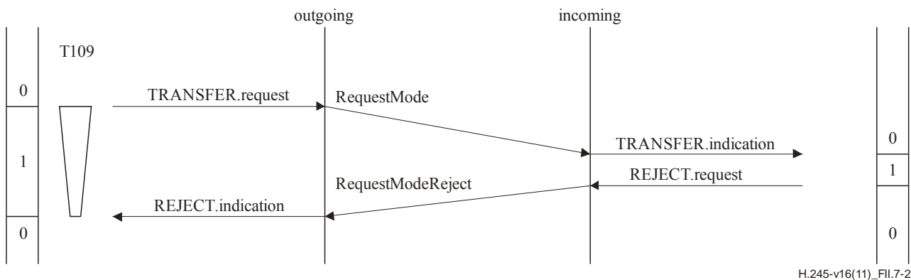
Figure II.7-2 – Mode request with rejection from the peer MRSE user
