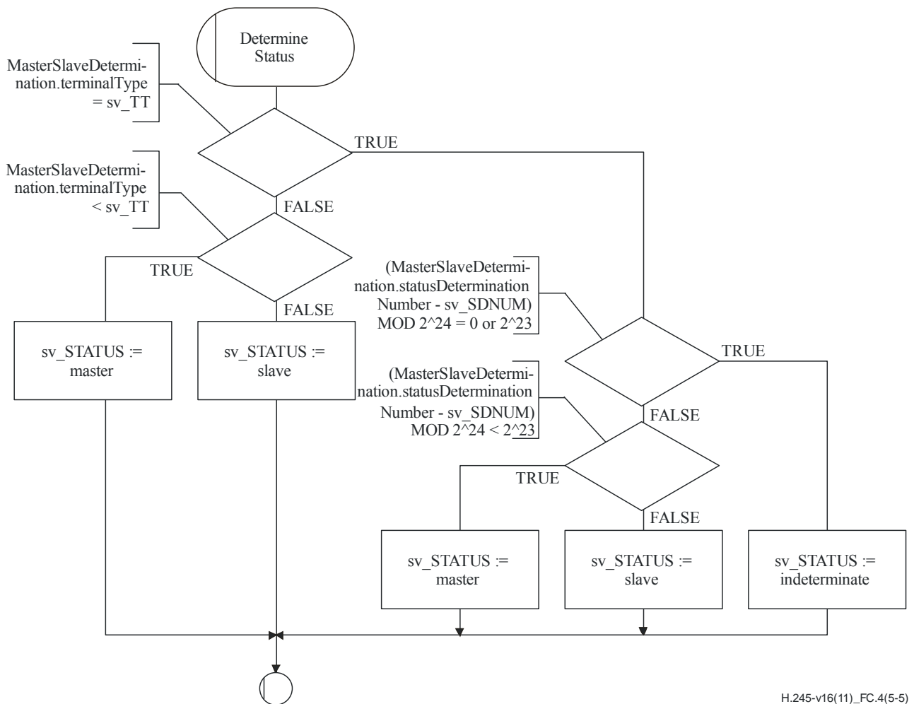
Figure C.4 – MSDSE SDL (sheet 5 of 5)
