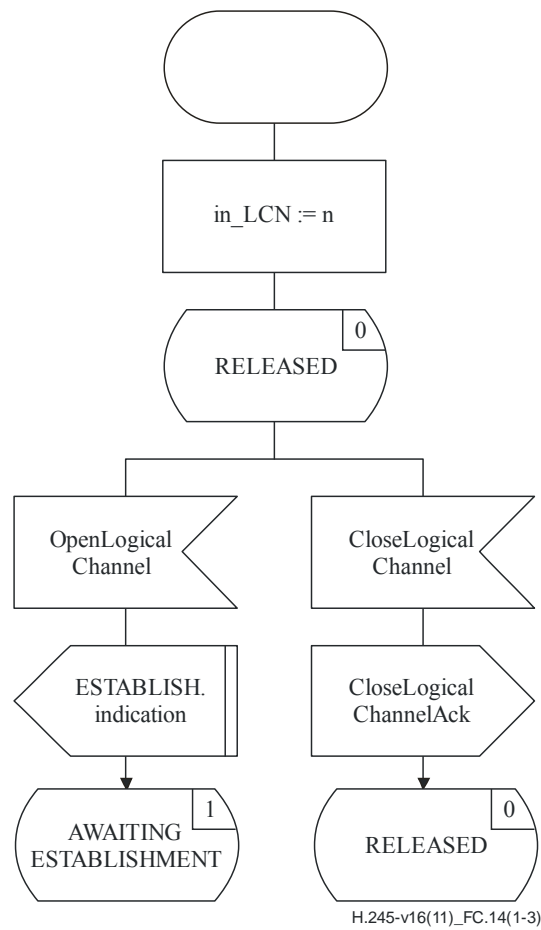
Figure C.14 – Incoming LCSE SDL (sheet 1 of 3)
