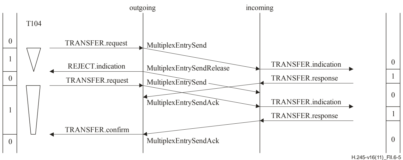
Figure II.6-5 – Multiplex table send request with timer T104 expiry followed by a second multiplex table send request
