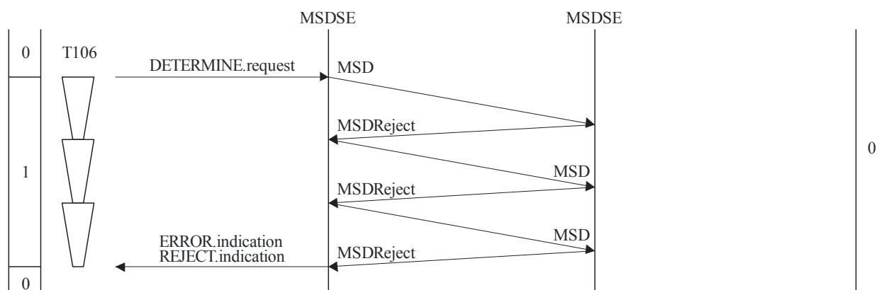
Figure II.2-10 – Master-slave determination – Indeterminate result with N100 = 3
