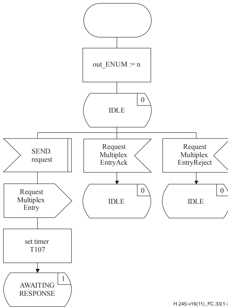
Figure C.33 – Outgoing RMESE SDL (sheet 1 of 2)
