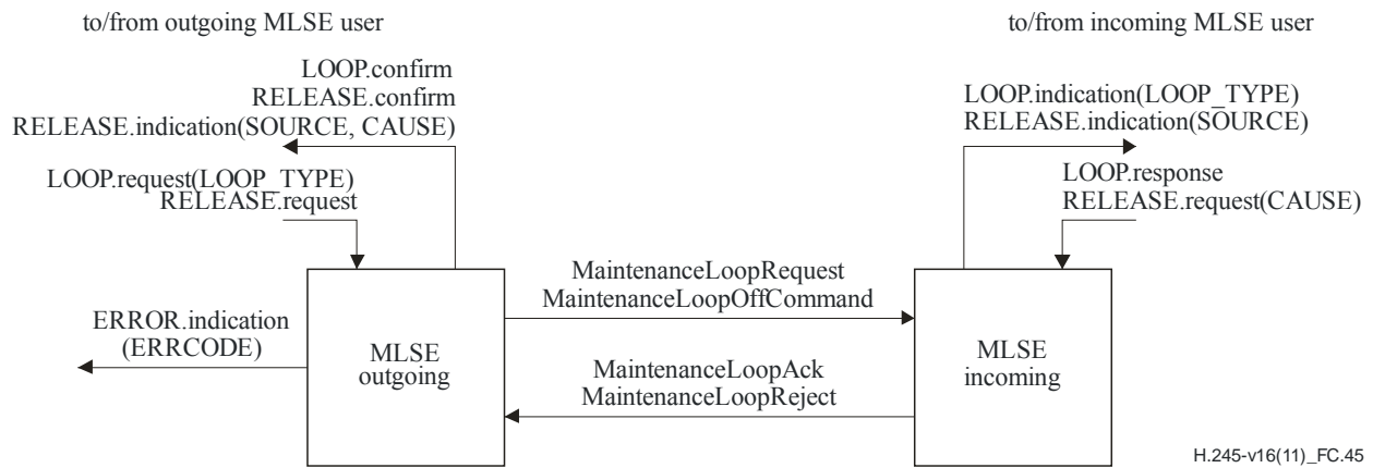
Figure C.45 – Primitives and messages in the Maintenance Loop Signalling Entity
