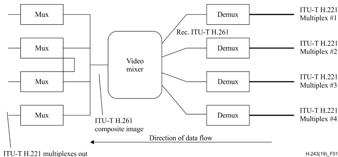
Figure 1 – Video mixing example: Quadrature
