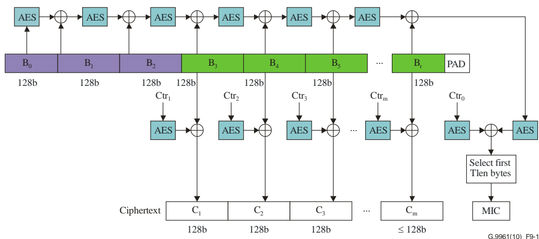
Figure 9-1 – Functional diagram of CCM encryption and message-authentication
