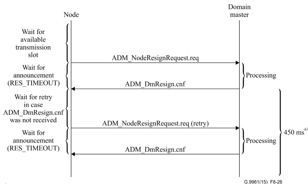
Figure 8-26 – Protocol diagram describing node resignation
