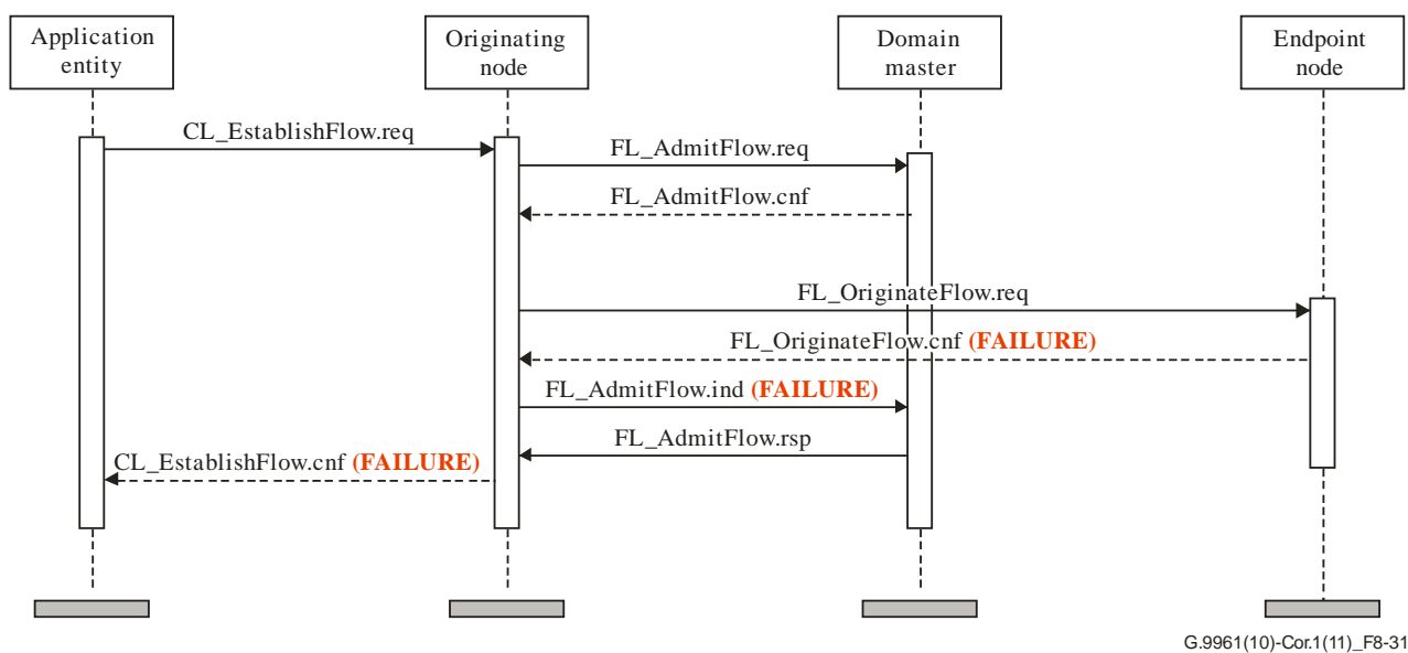
Figure 8-31 – Failure in flow establishment due to rejection by endpoint node
