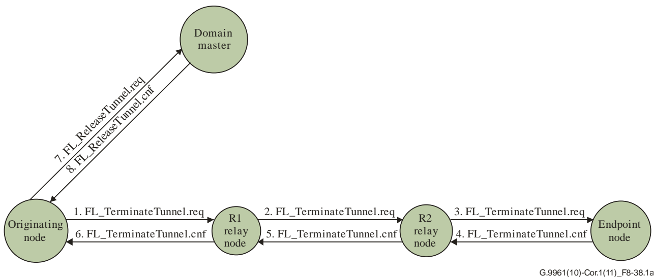
Figure 8-38.1a – Normal tunnel termination
