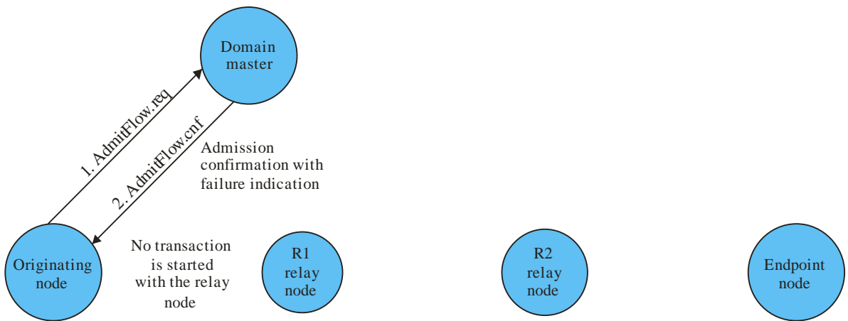
Figure 8-35 – Example of a tunnel establishment failure scenario due to the domain master rejecting the admission request
