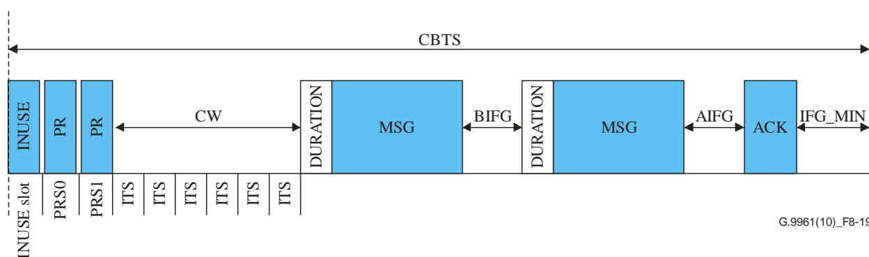
Figure 8-19 – Example of duration-based CBTS closure
