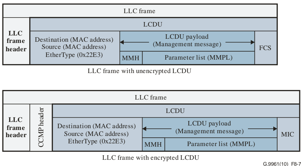
Figure 8-7 – Encapsulation of an LCDU into an LLC frame
