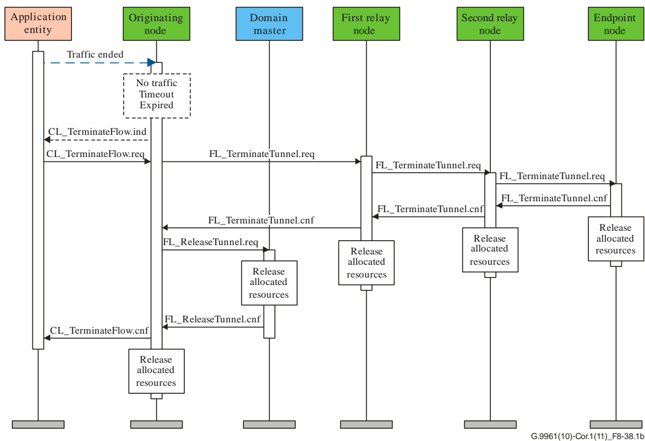
Figure 8-38.1b – MSC of normal termination of a tunnel
