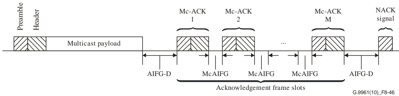
Figure 8-46 – Multicast acknowledgment with NACK signalling
