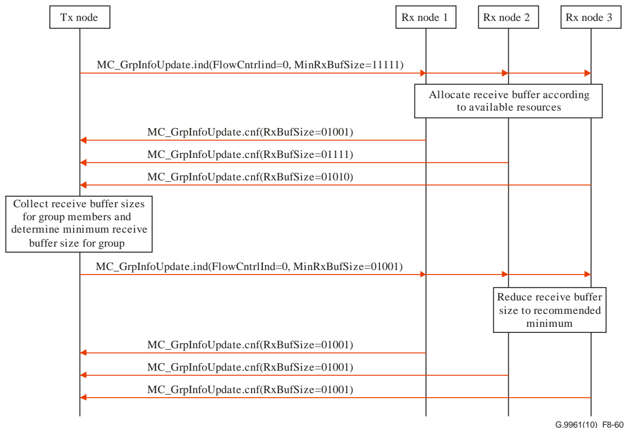
Figure 8-60 – Example of establishment of a PHY multicast group with flow-control disabled
