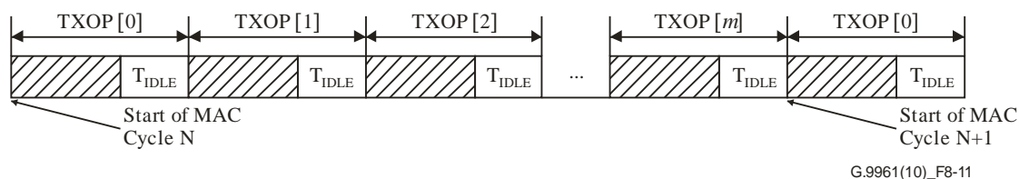
Figure 8-11 – IFG placement in the MAC cycle
