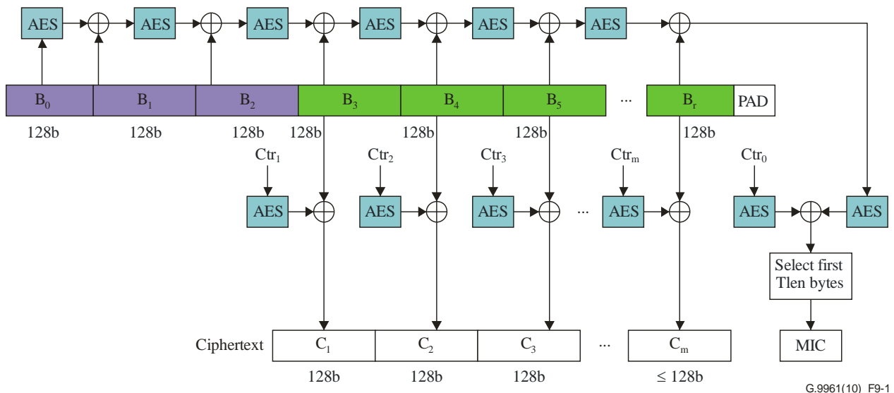
Figure 9-1 – Functional diagram of CCM encryption and message-authentication
