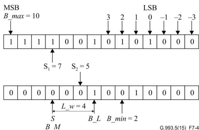
Figure 7-4 – Example of two registers, each representing a clipped error sample component
