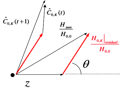
Figure III.6 – Detail of constellation point with pre-coding
