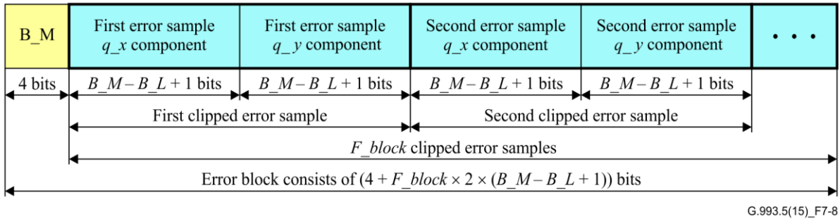
Figure 7-8 – Format of an error block
