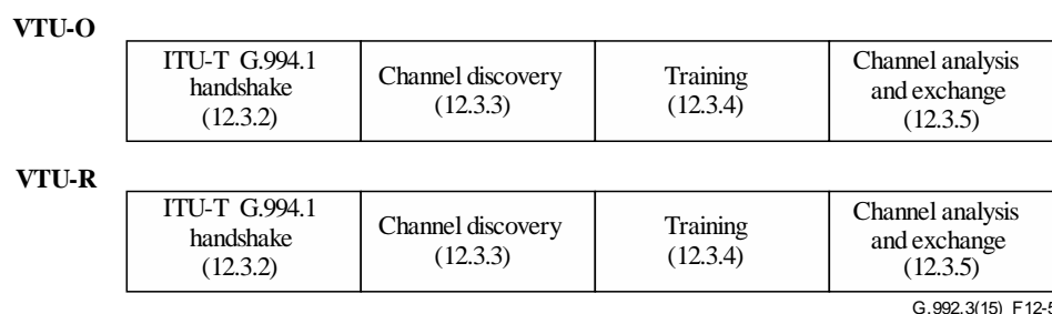
Figure 12-5 – Overview of initialization procedure
