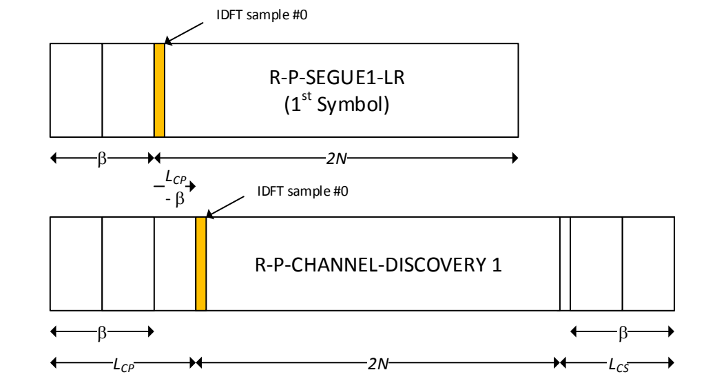
Figure D.3 – Reference samples for alignment of upstream symbols between the VDSL2-LR TRAINING stage and ITU-T G.993.2 channel discovery phase
