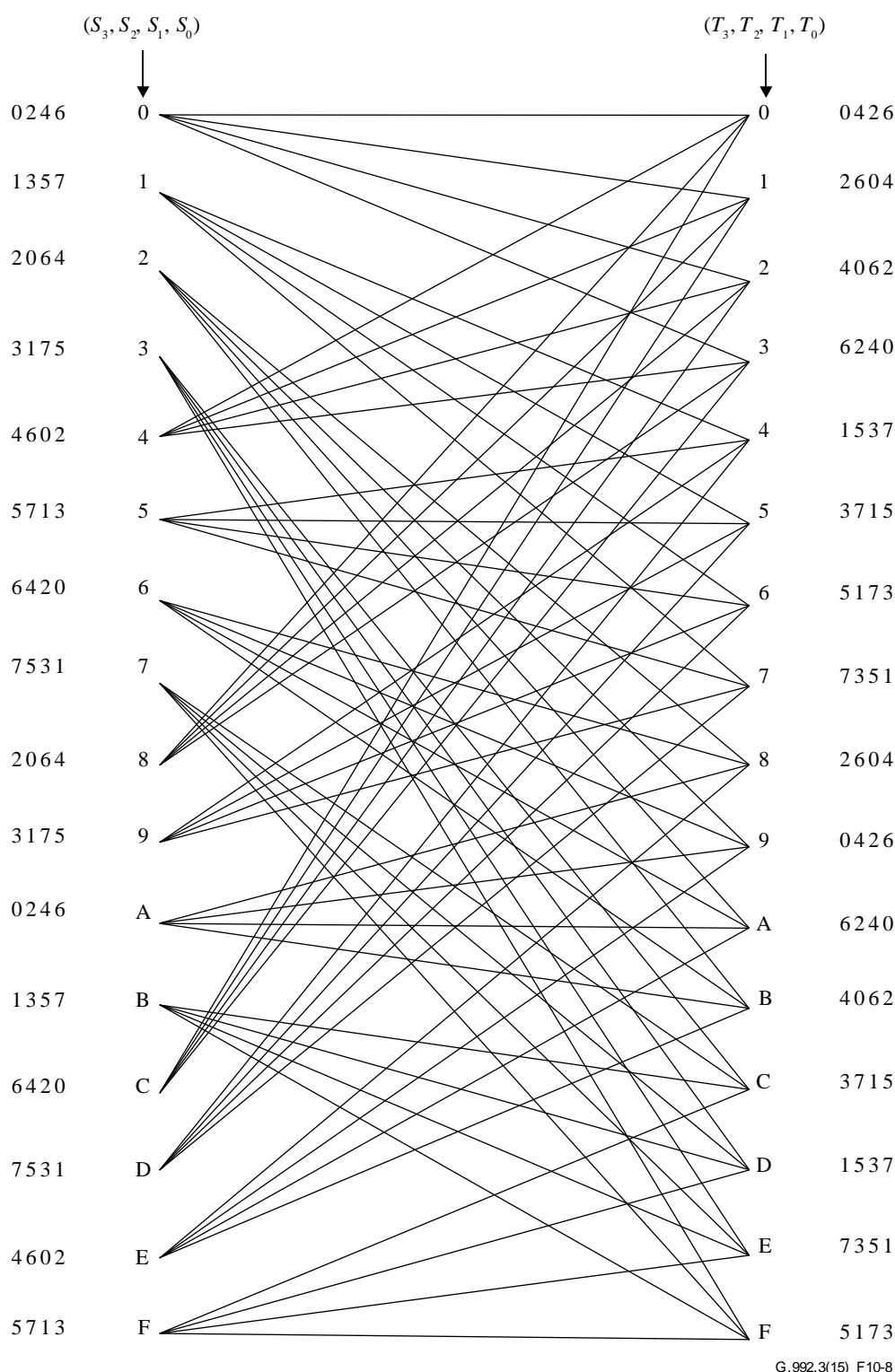
Figure 10-8 – Trellis diagram
