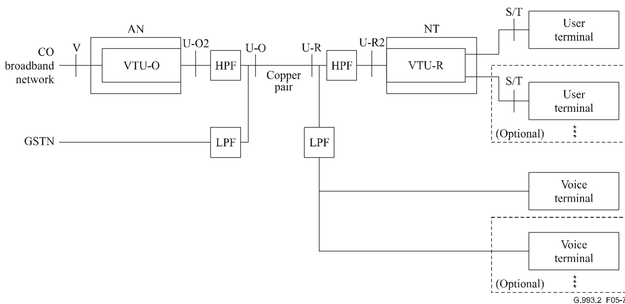
Figure 5-7 – Data with POTS service application model for remote deployment with splitter
