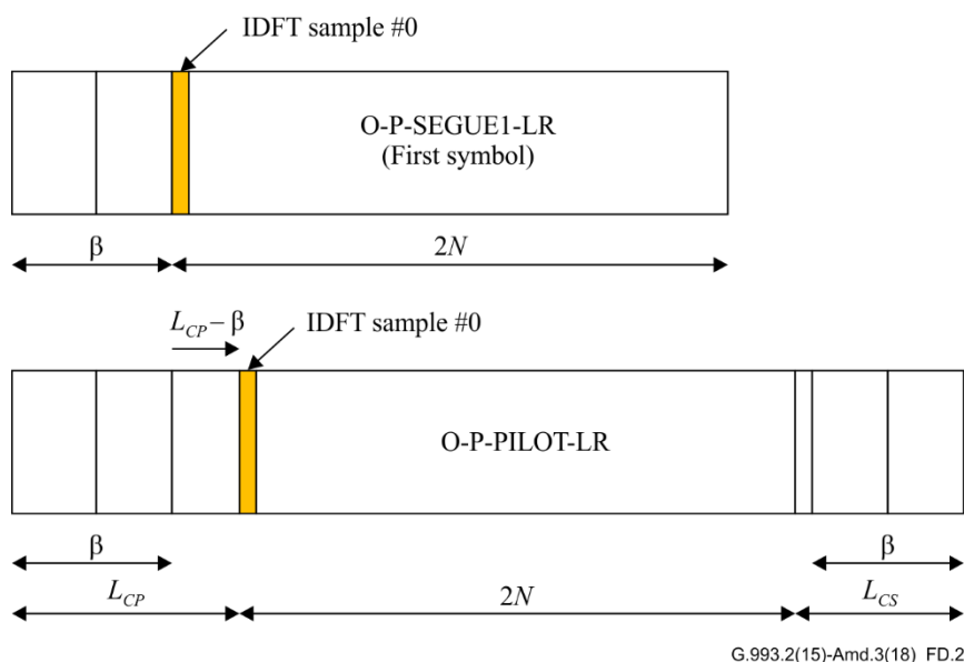
Figure D.2 – Reference samples for alignment of downstream symbols between the O-SEGUE 1-LR state and O-P-PILOT-LR state
