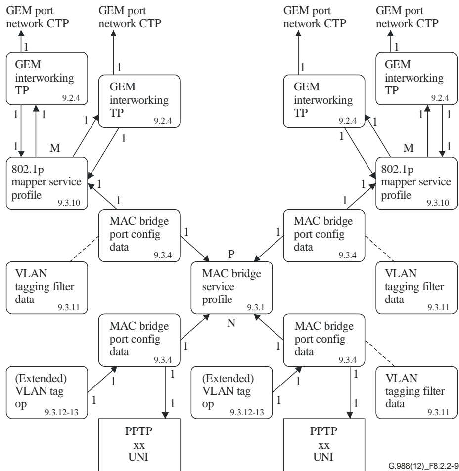
Figure 8.2.2-9 – Illustration of N:MP bridge-map-filtering
