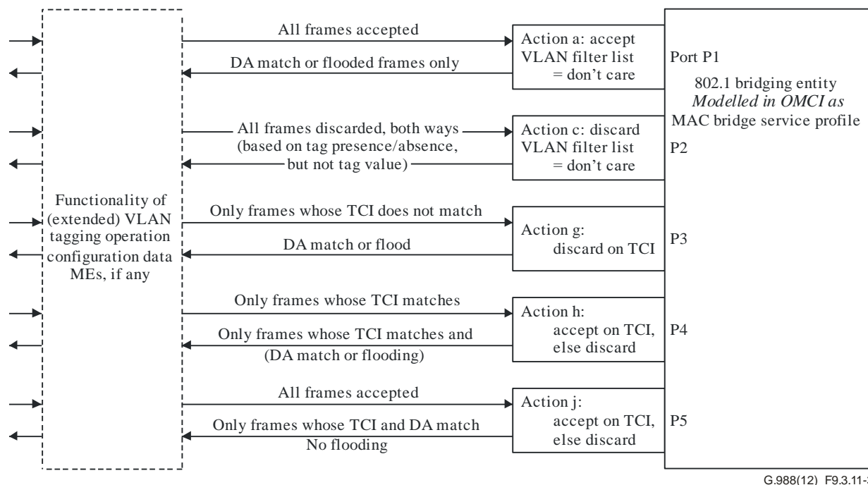
Figure 9.3.11-3 – Forwarding behaviour
