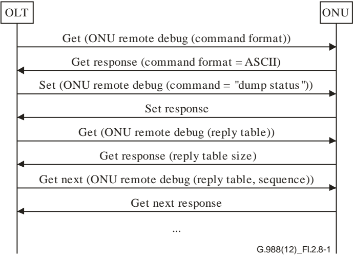
Figure I.2.8-1 – Success example
