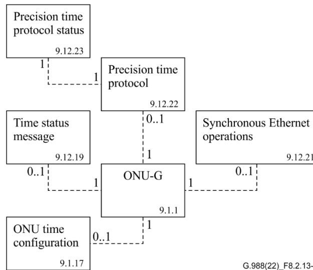
Figure 8.2.13-1 – ONU packet-based Time Synchronization
