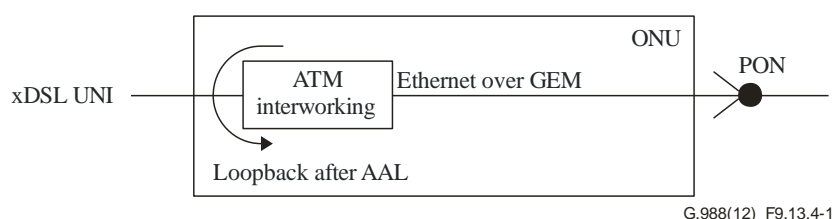
Figure 9.13.4-1 – AAL loopback configuration
