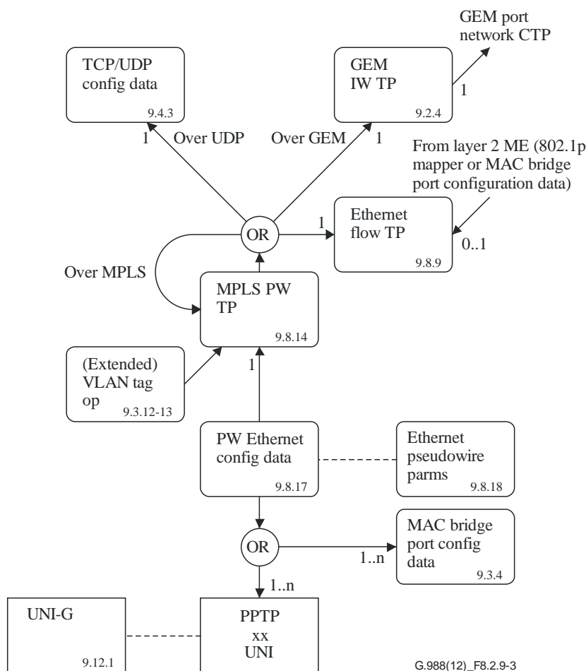
Figure 8.2.9-3 – Ethernet pseudowire
