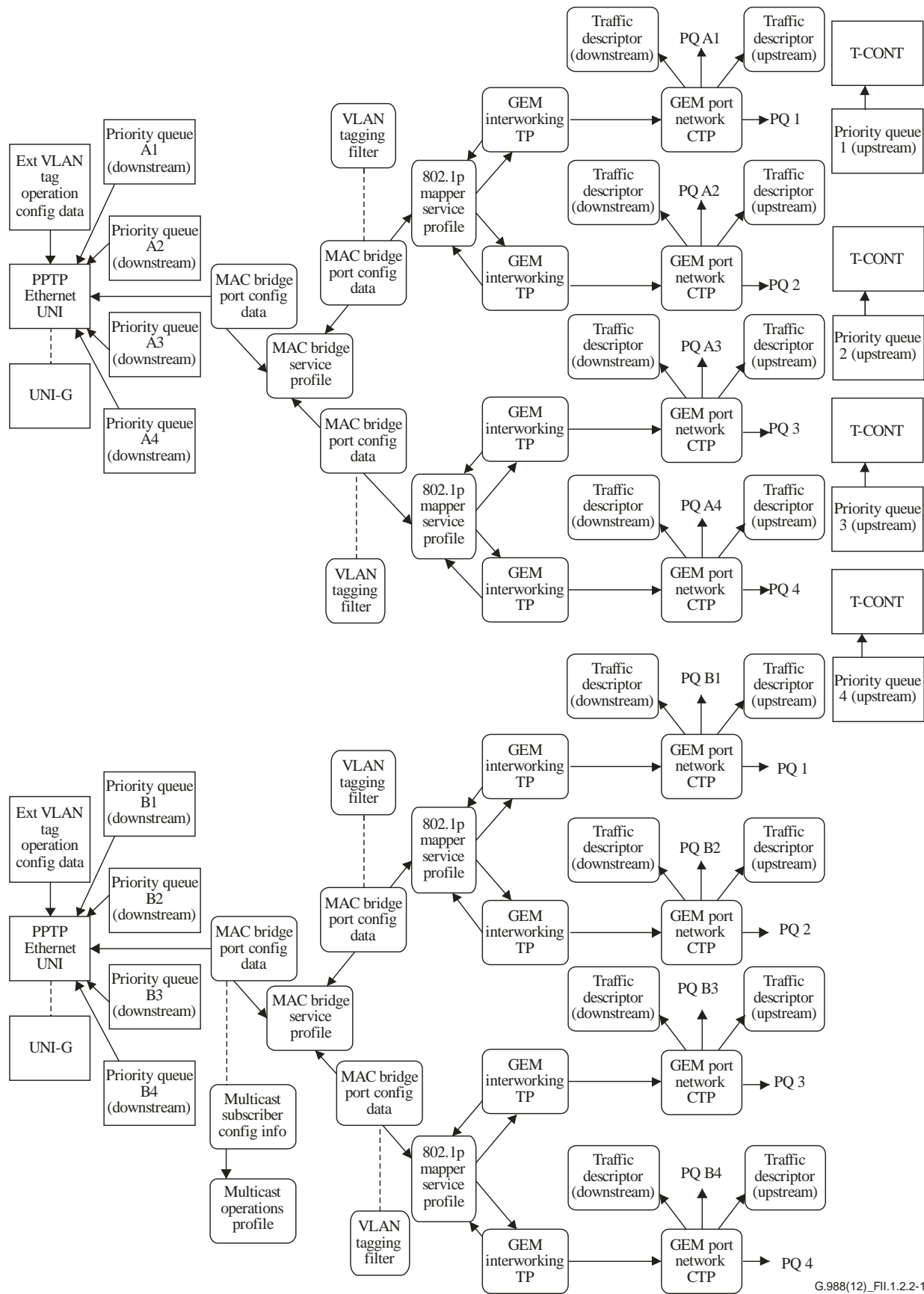
Figure II.1.2.2-1 – Multi-UNI L2-OCM
