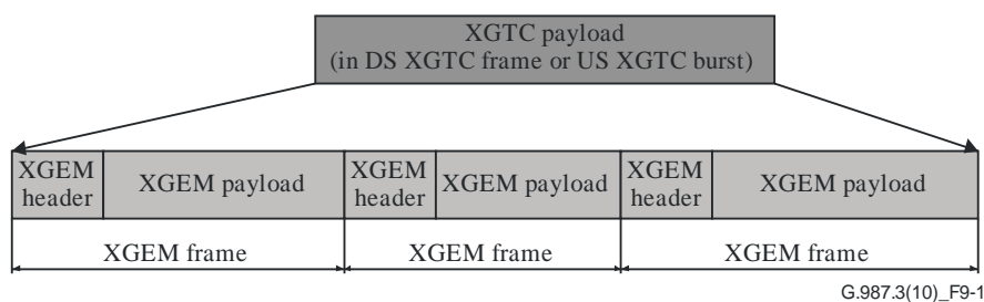
Figure 9-1 – Structure of XGTC payload
