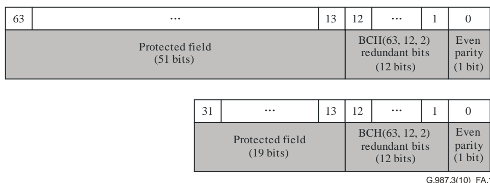
Figure A.1 – Hybrid error correction structure, showing details of the 13-bit header error control field
