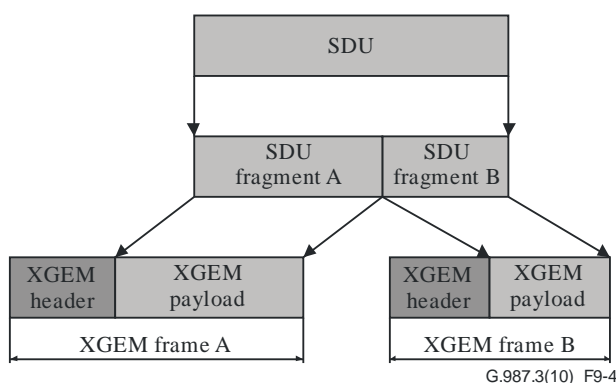
Figure 9-4 – SDU fragmentation
