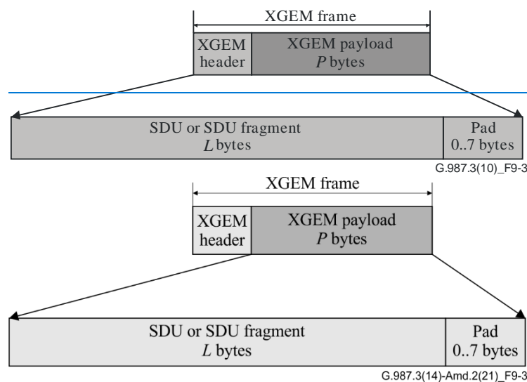
Figure 9-3 – XGEM payload format
