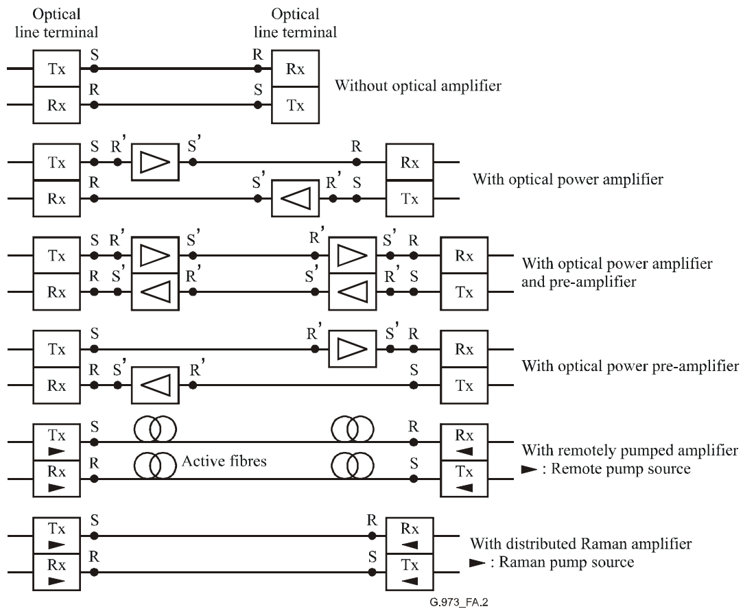
Figure A.2 – Possible system configurations
