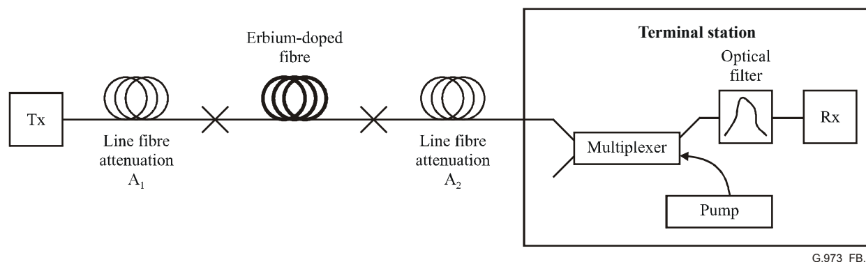
Figure B.1 – Example of system configuration with ROPA from the receiver end
