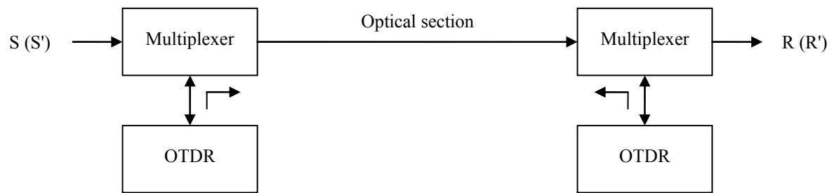
Figure B.2 – Example of line monitoring using OTDR
