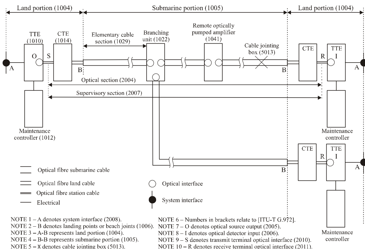
Figure A.1 – Example of repeaterless optical fibre submarine cable system
