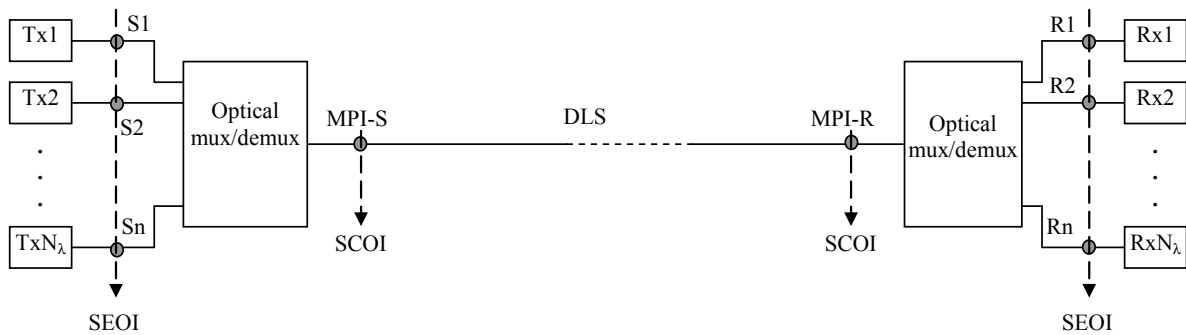
Figure 1 – Representation of optical line system interfaces (multichannel system)
