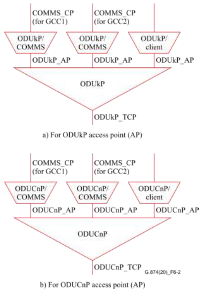
Figure 6-2 – COMMS (GCC1 and GCC2) access at ODU k P access point
