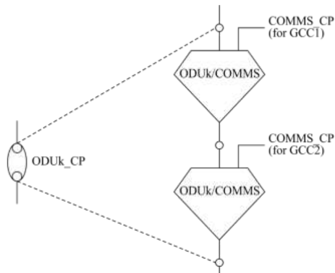
a) ODUk_CP expansion for COMMS access
