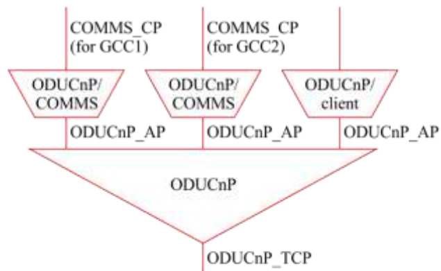
b) ODUCn_CP expansion for COMMS access
