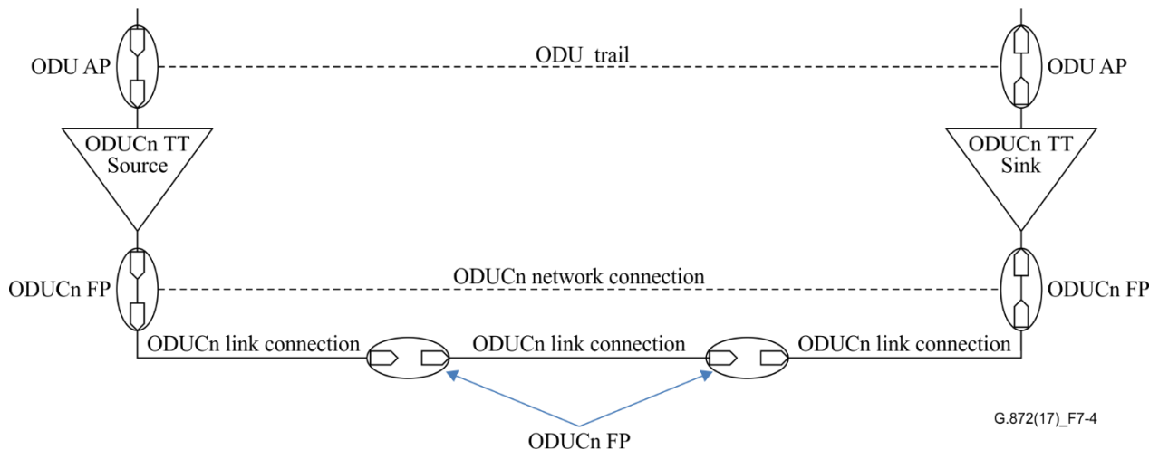
Figure 7-4 – ODUCn layer network example
