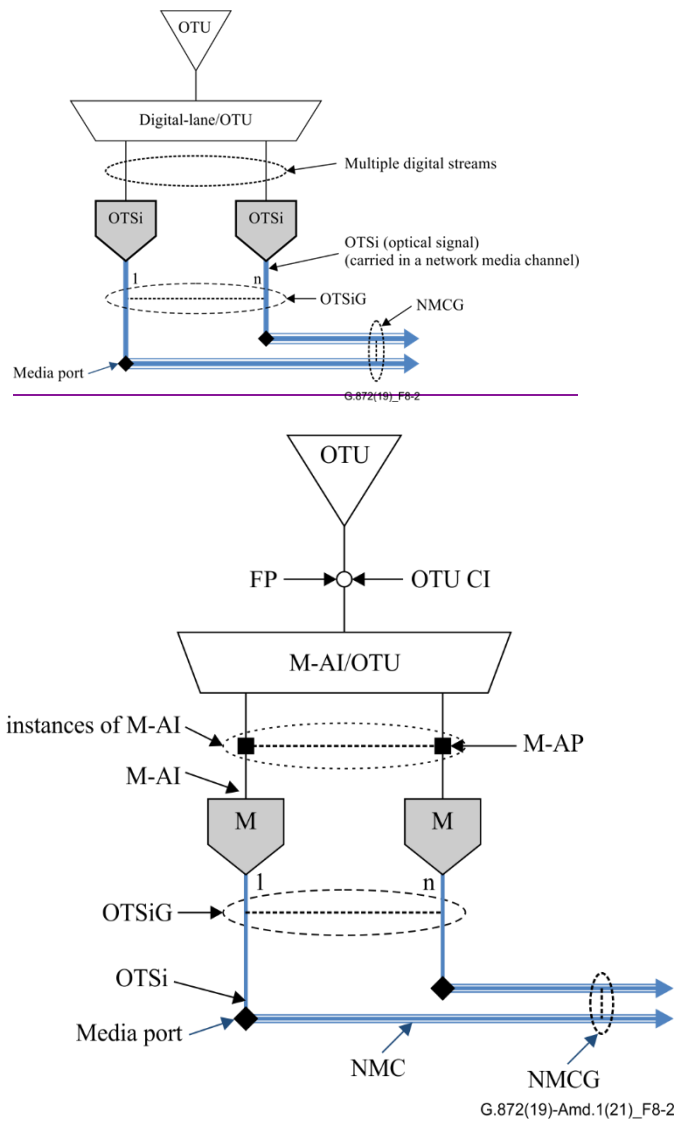
Figure 8-2 – Mapping an OTU to an OTSiG that contains more than one OTSi
