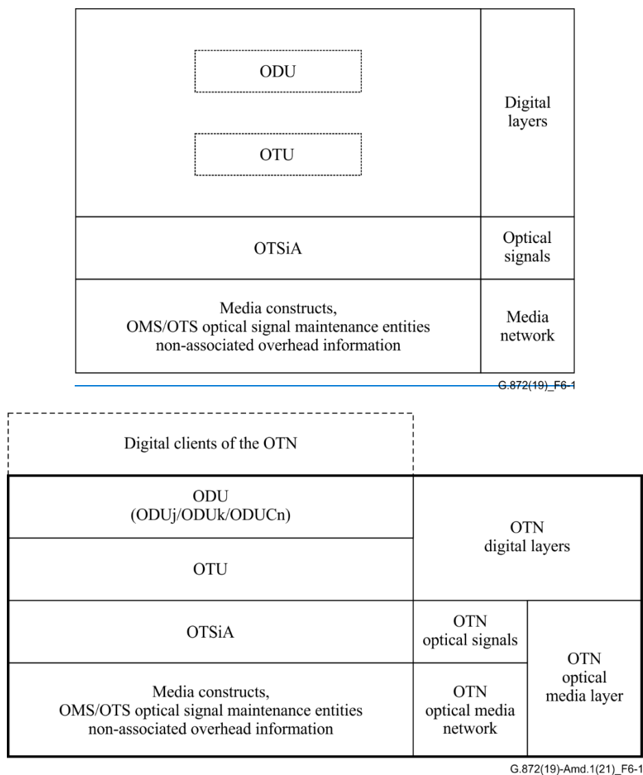
Figure 6-1 – Overview of the OTN
