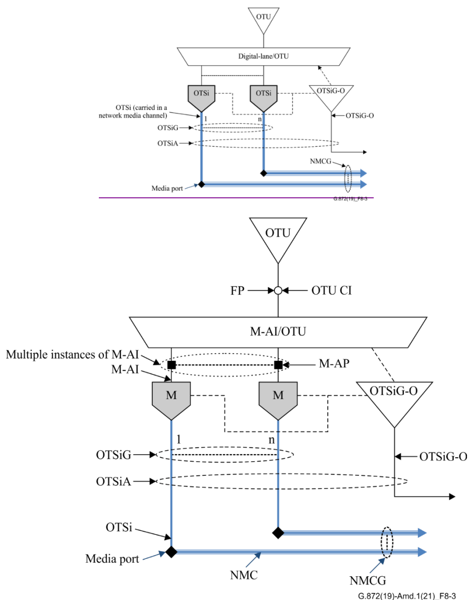
Figure 8-3 – Mapping an OTU to an OTSiA with non-associated overhead (OTSiG-O)
