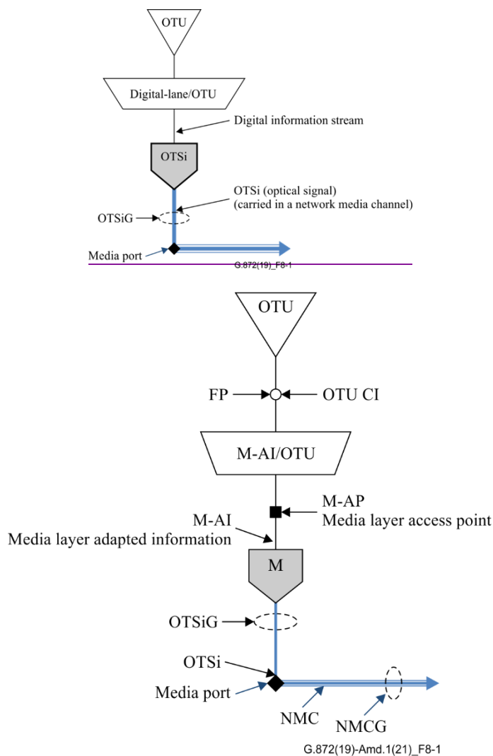
Figure 8-1 – Mapping an OTU to an OTSiG that contains one OTSi
