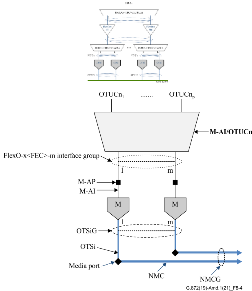
Figure 8-4 – Mapping an OTUCn to FlexO group where each FlexO-x-<FEC> interface is carried by one OTSi
