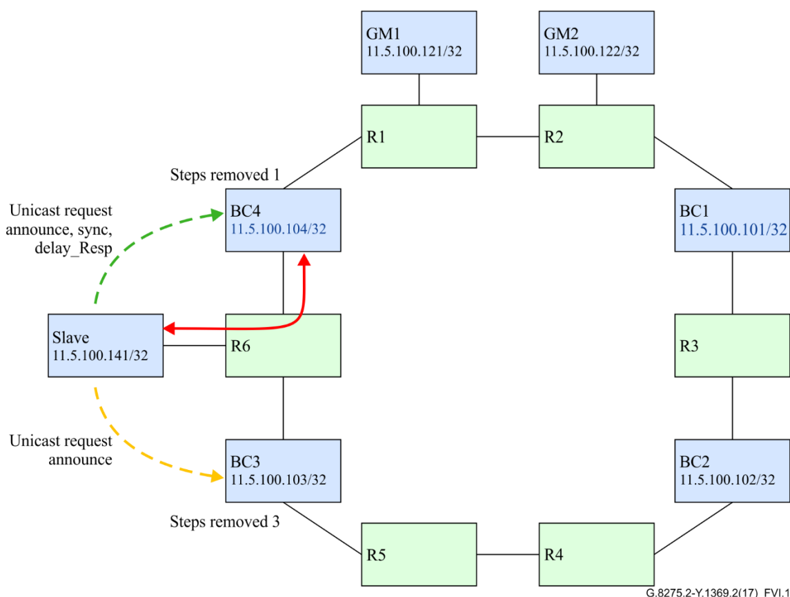
Figure VI.1 – Normal operation
