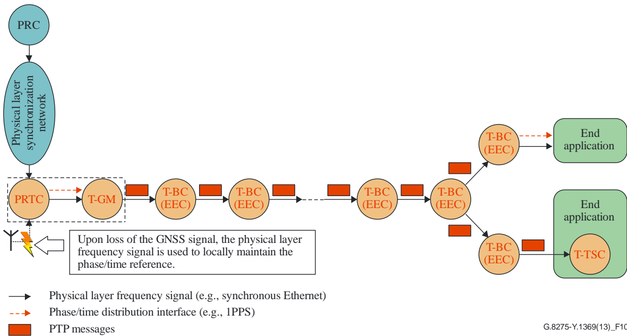
Figure 10 – Illustration of protection scenario 1.2 at the PRTC/GM, (phase/time long-term holdover at the PRTC/GM, with the PRTC/GM not collocated with the end application)
