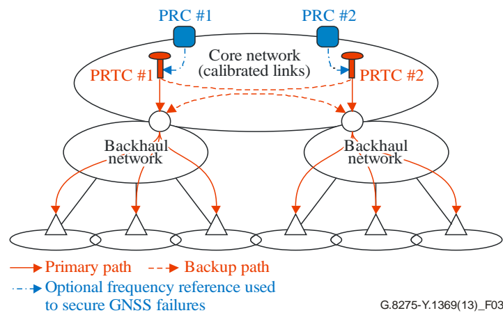
Case B: centralized PRTC not collocated with PRC
