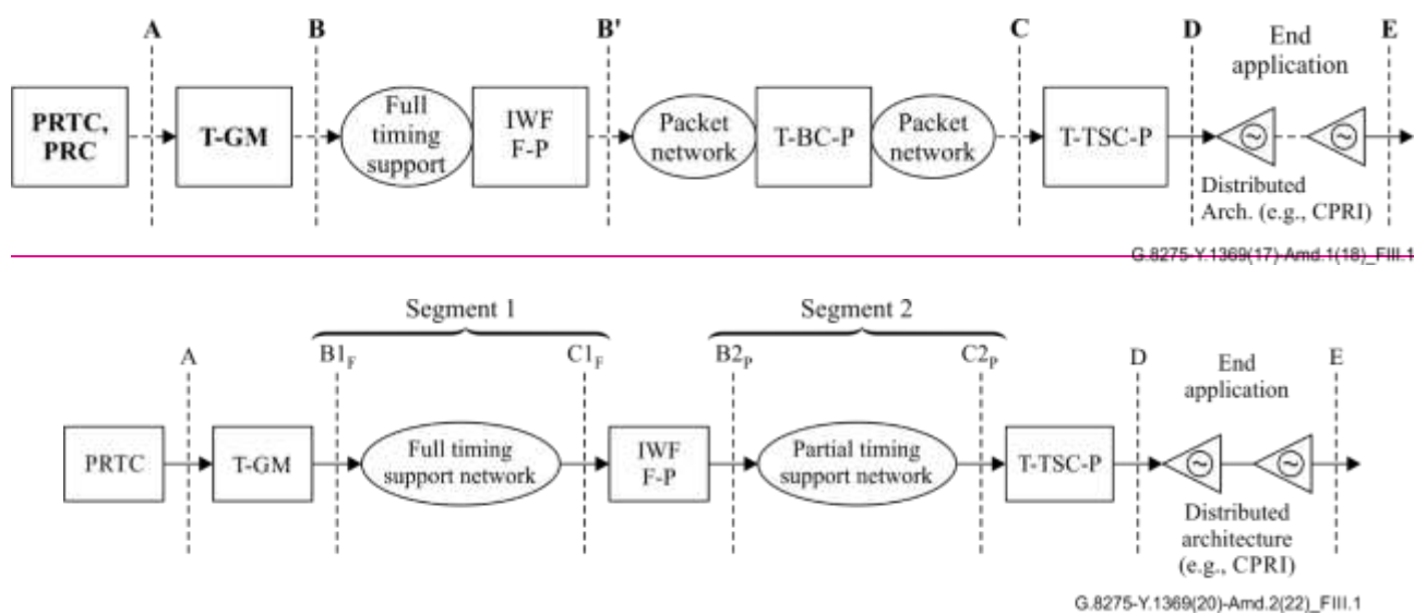
Figure III.1 – Deployment case requiring IWF node
