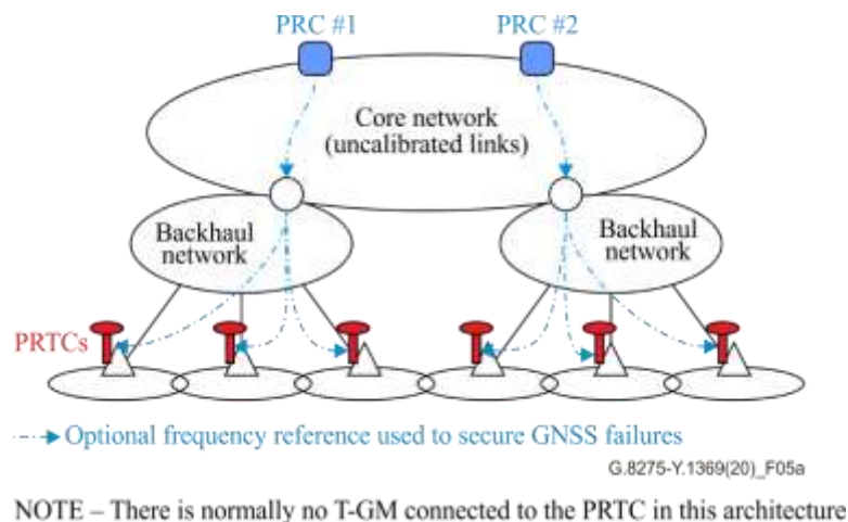
Figure 5a – Architecture with PRTC functions distributed at cell sites
