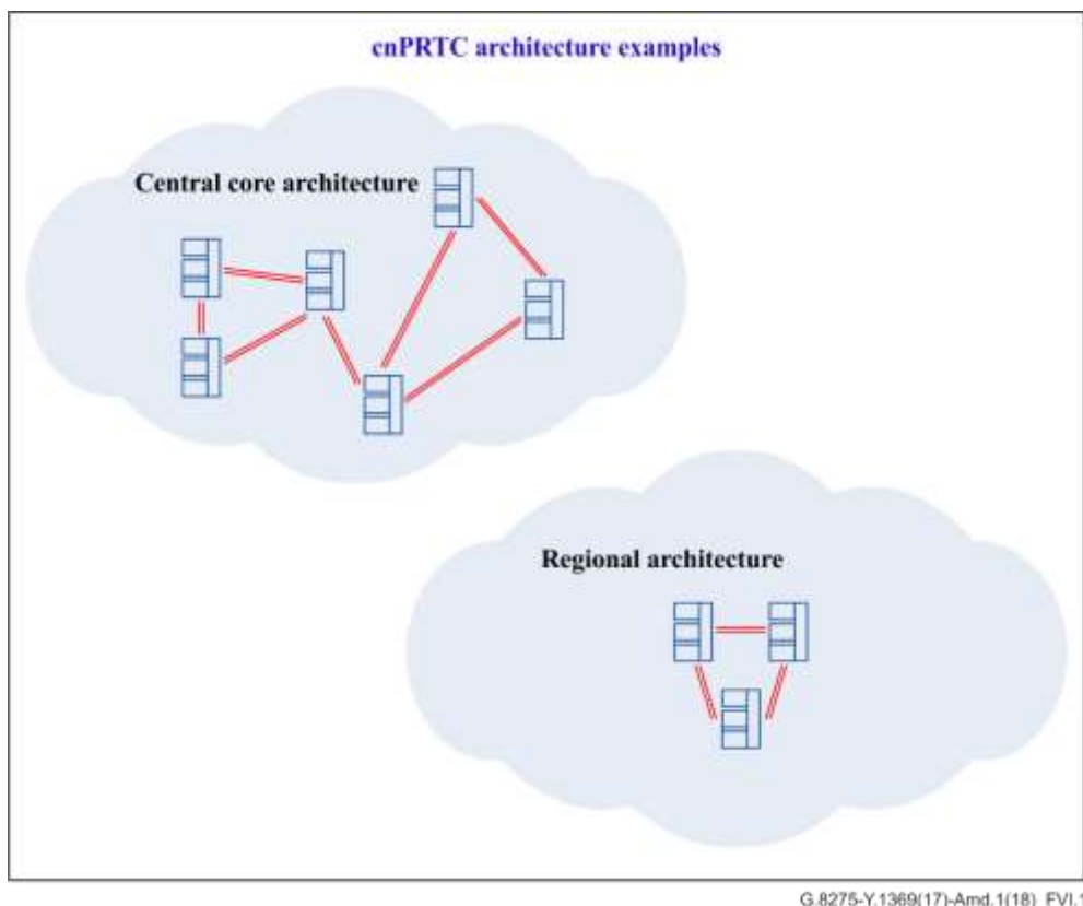
Figure VI.1 – Coherent network PRTC architecture examples
