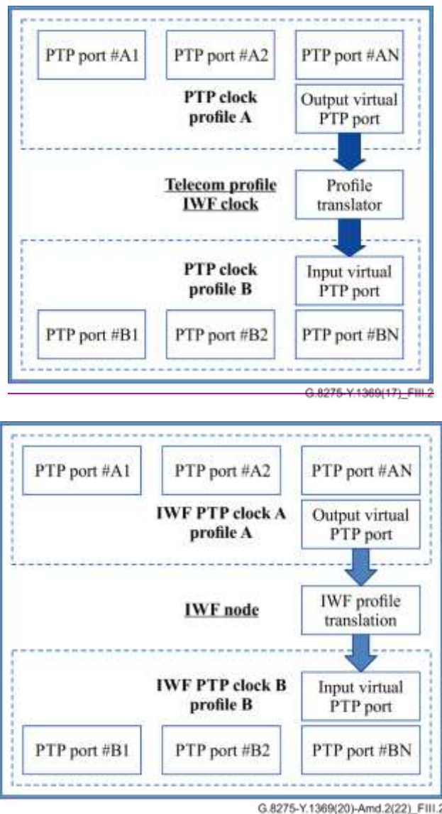
Figure III.2 – Model of telecom profile IWF clock node
