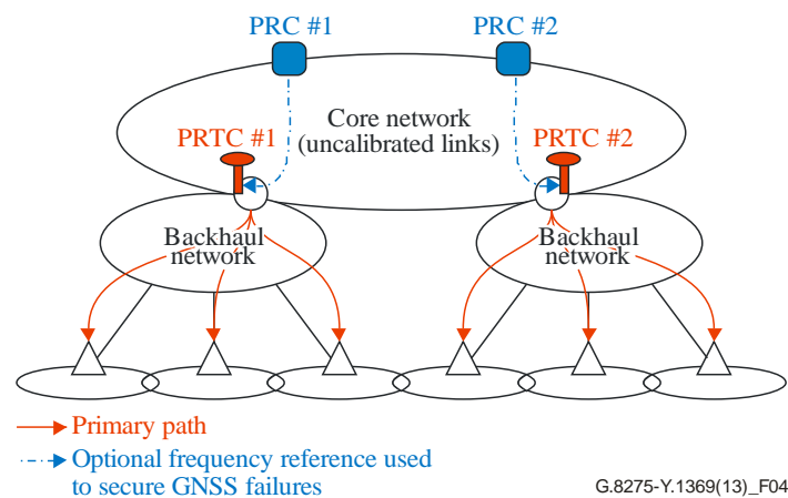
Case C: distributed PRTC in aggregation sites
