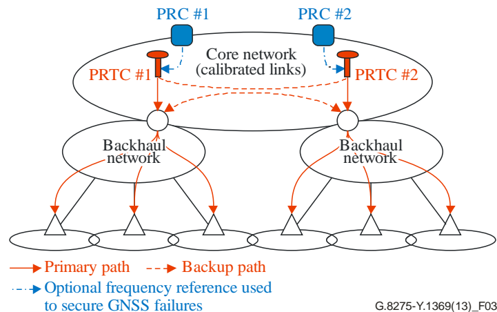
Figure 3 – Architecture with centralized PRTC functions not collocated with PRC
