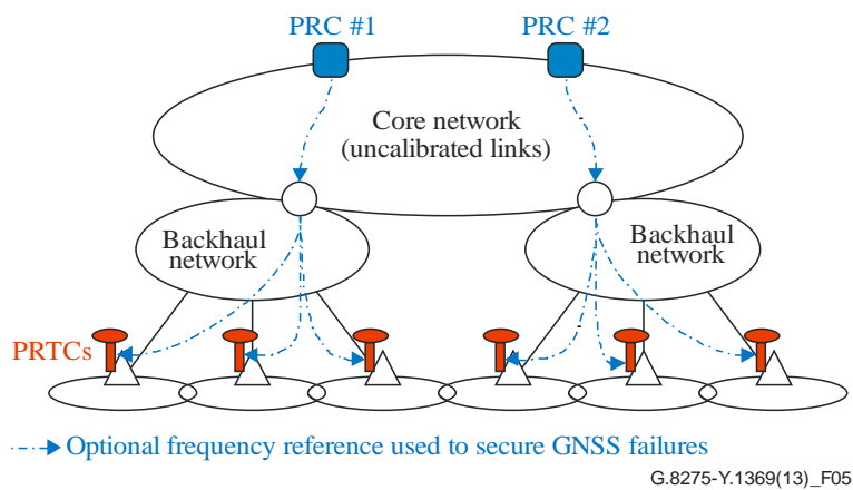
Figure 5a – Architecture with PRTC functions distributed at cell sites
