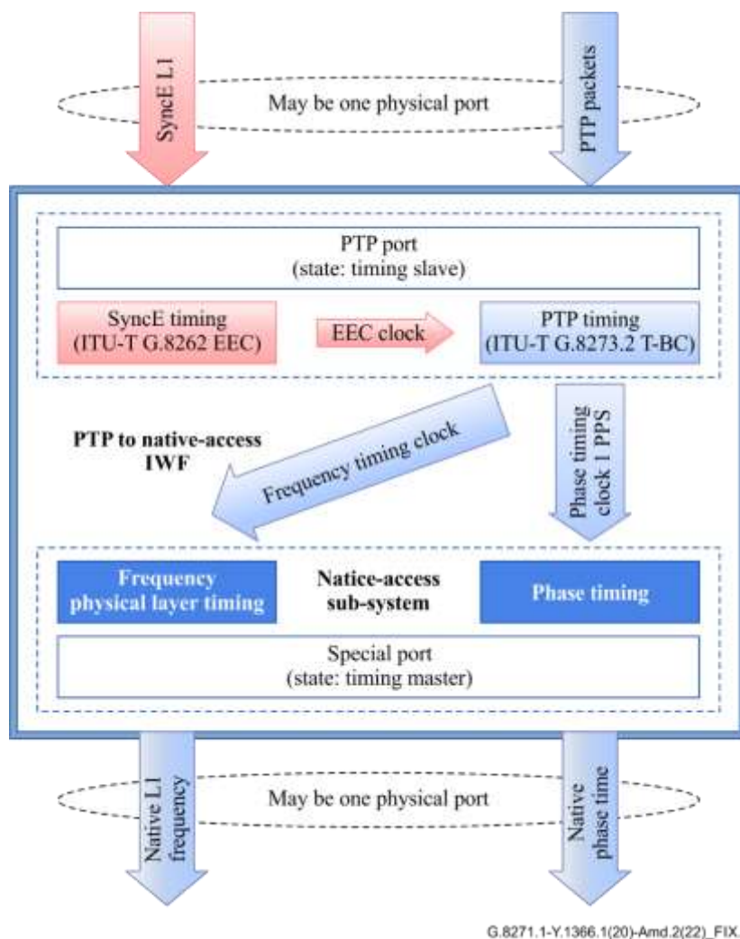
Figure IX.4 – Timing flow from PTP to native access media (downstream) with a dependence between physical layer timing and phase timing
