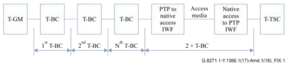
Figure IX.1 – Network reference model for phase/time synchronization over a native access media
