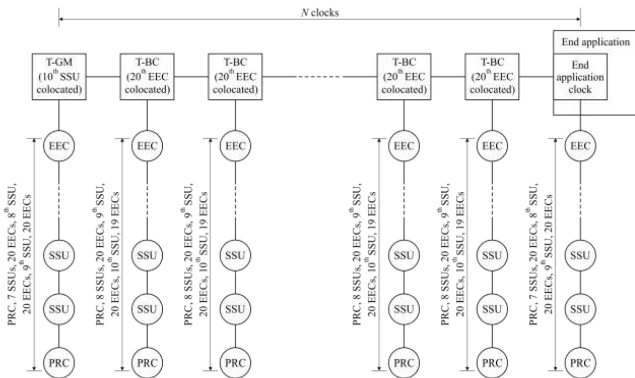
Figure II.4 – HRM-3 with physical layer frequency support – non-congruent scenario, deployment case 1
