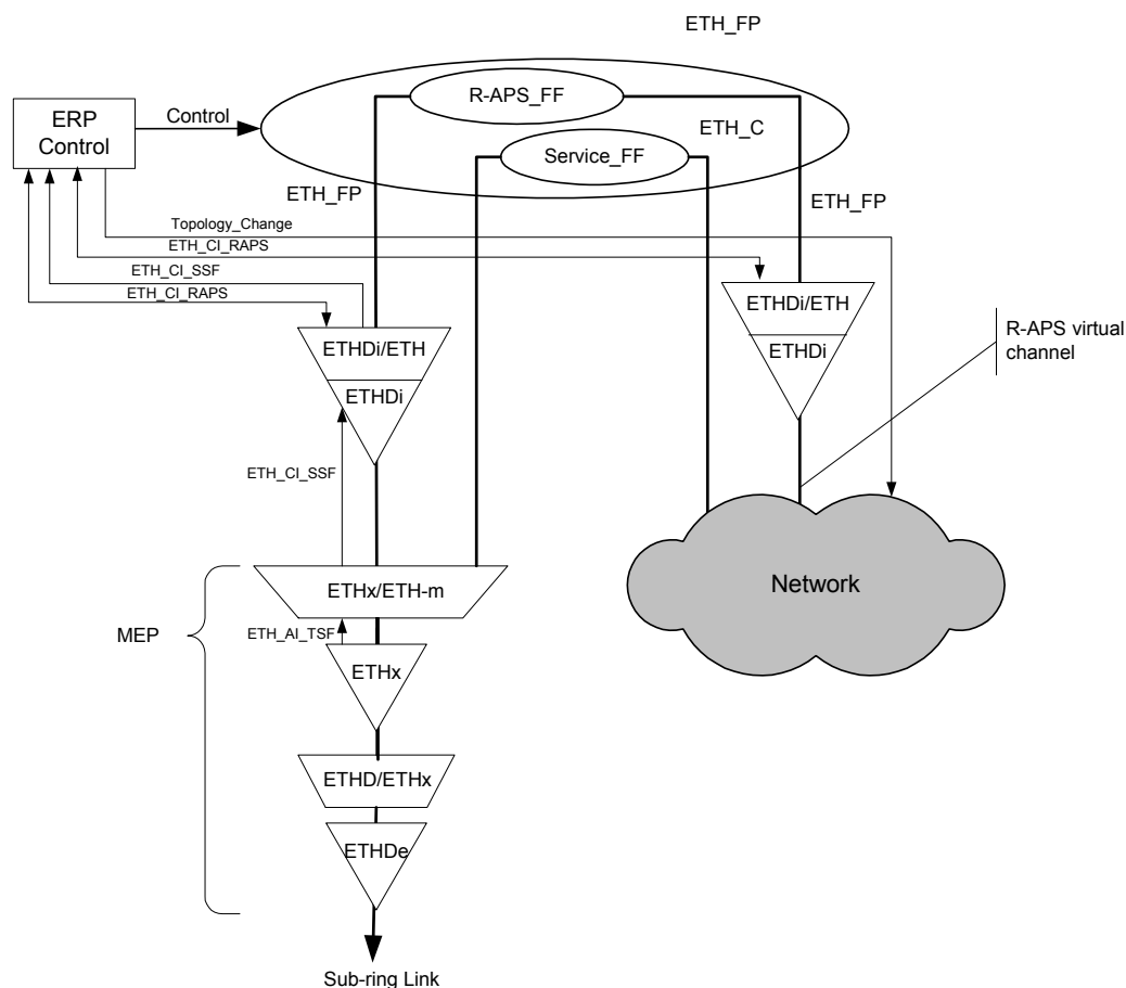
Figure 9-7 – MEPs and R-APS insertion function in an interconnection node (for a sub-ring connected to another network)
