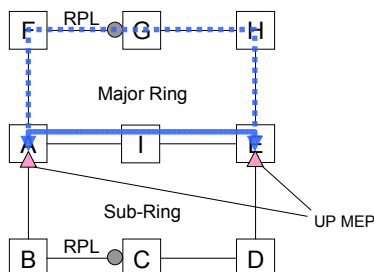
Figure X.3 – Interconnected rings connectivity verification
