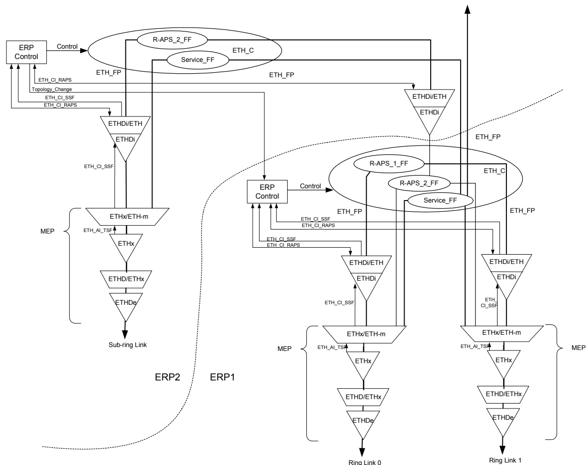
Figure 9-8 – MEPs and R-APS insertion function in an interconnection node with R-APS virtual channel (different R-APS VIDs)
