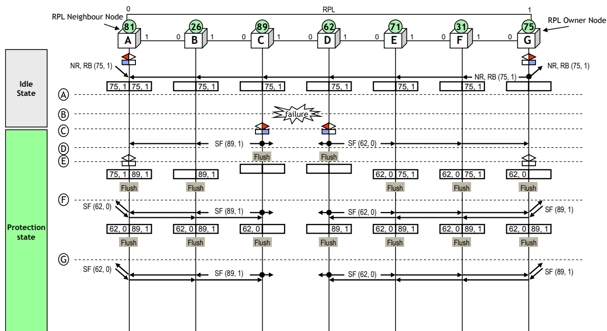
Figure III.1 – Single link failure
