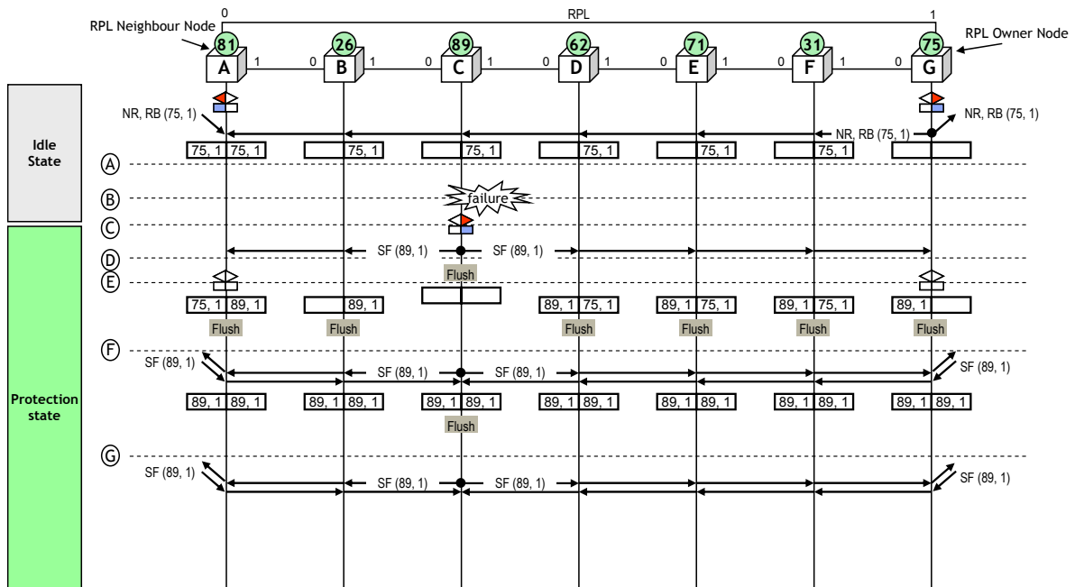
Figure III.4 – Unidirectional single link failure
