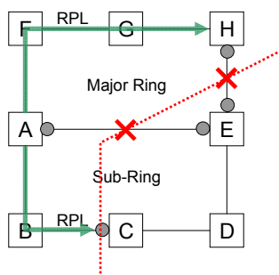
Figure X.2 – No connectivity between interconnection nodes
