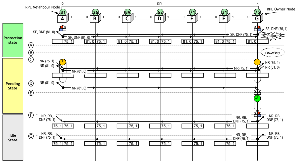
Figure III.7 – RPL failure recovery
