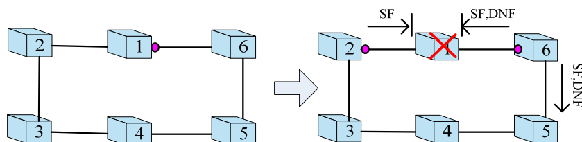
Figure VIII.2 – RPL owner node or RPL neighbour node failure case
