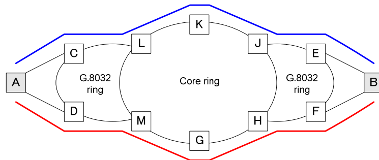
Figure XI.2 – End-to-end service resilience over interconnected rings
