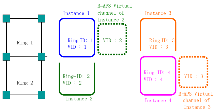
Figure VII.2 – Example 2: Different VIDs for different ERP instances; same VID for an ERP instance of sub-ring and an R-APS virtual channel
