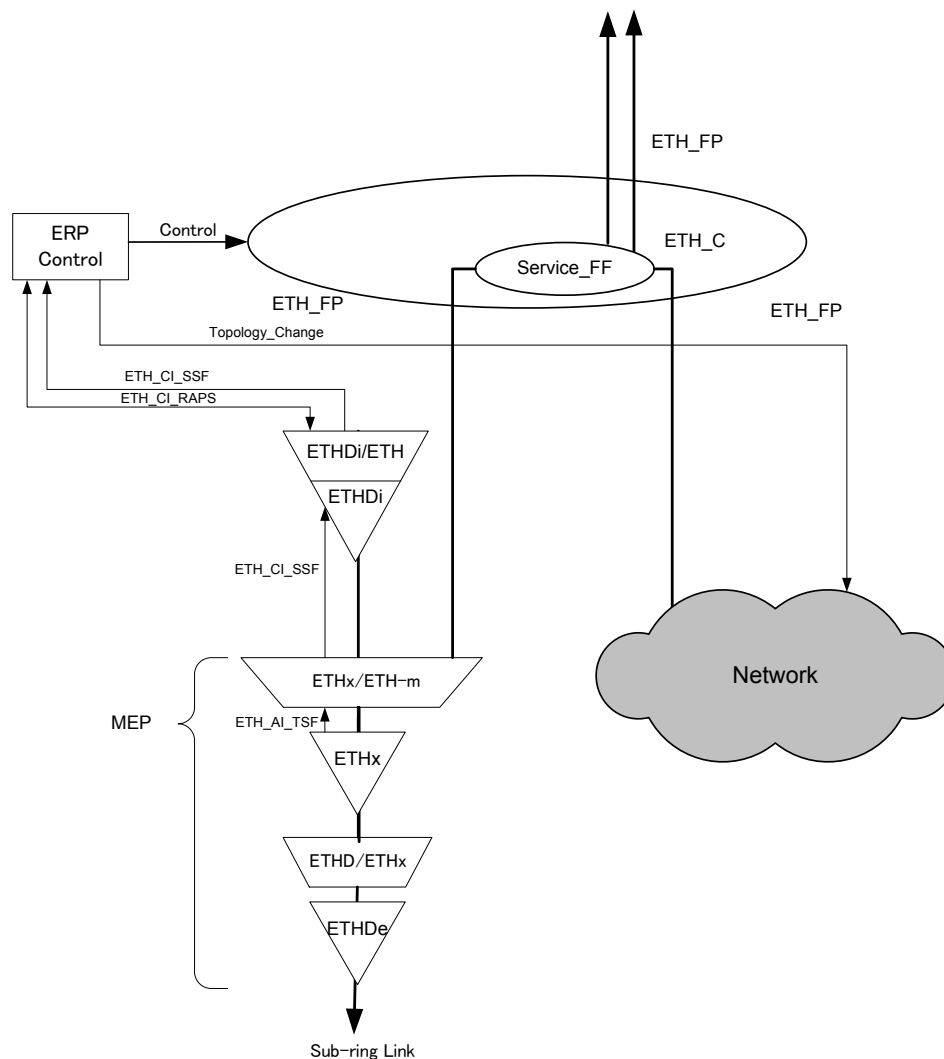
Figure 9-9 – MEPs and R-APS insertion function in a sub-ring interconnection node without R-APS virtual channel (for a sub-ring connected to another network)
