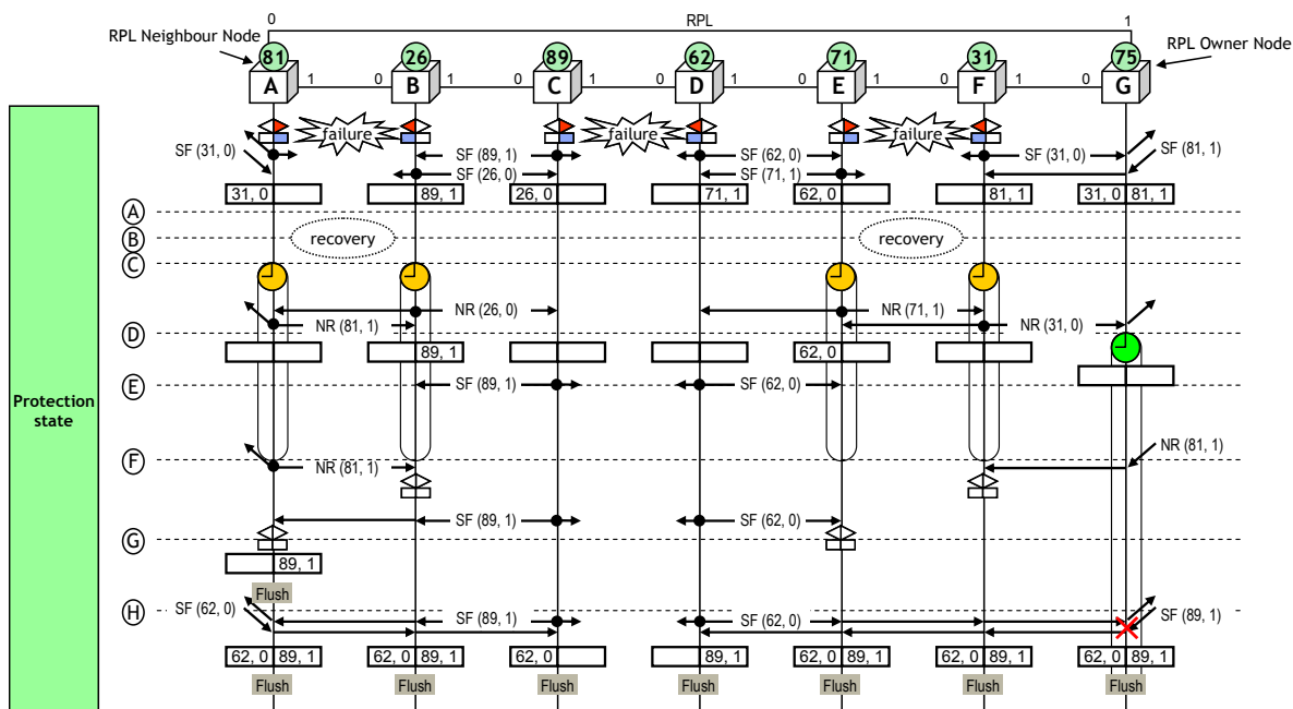
Figure III.8 – Multiple link failure
