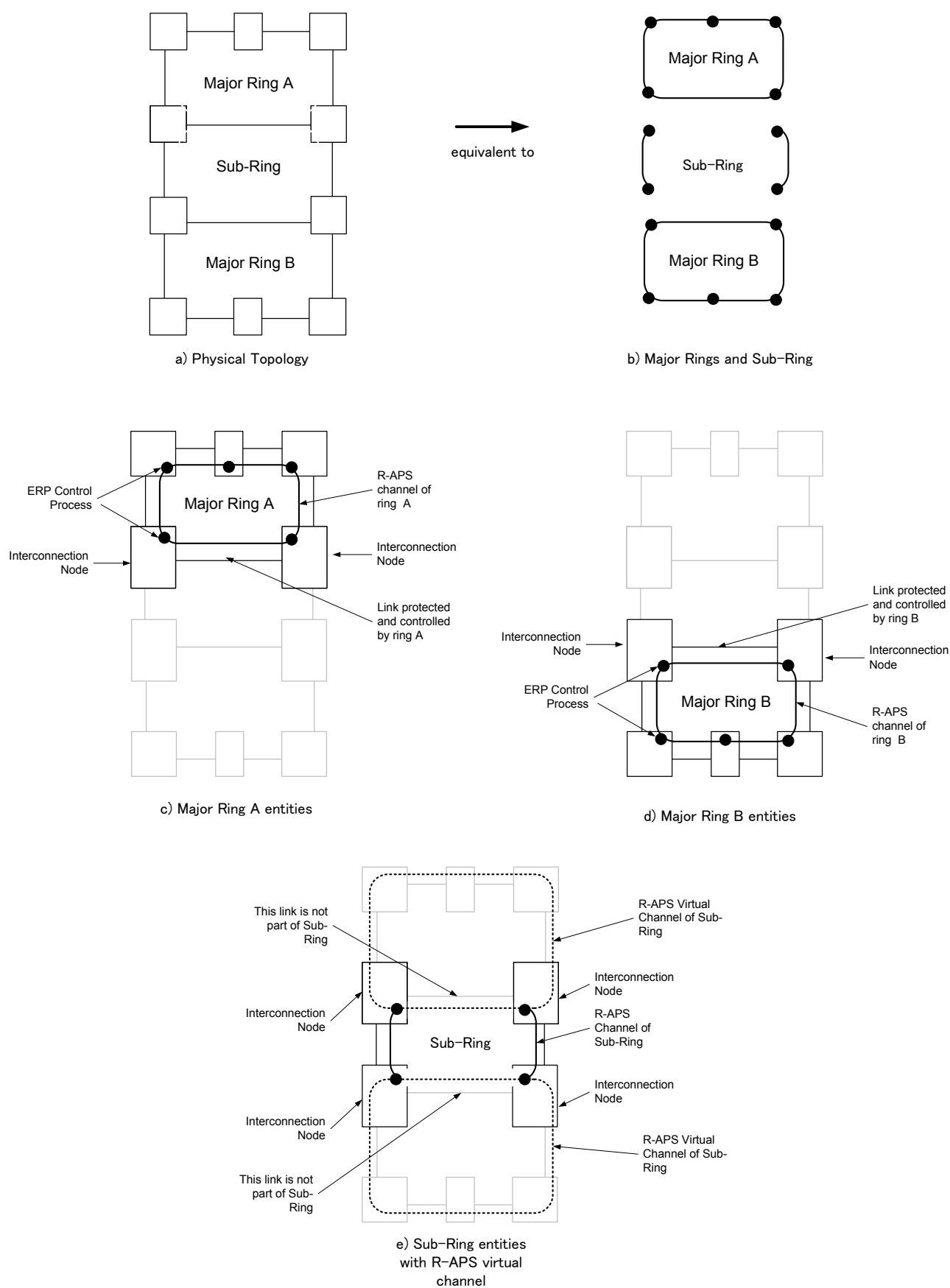
Figure V.2 – Configuration for interconnection between multiple major rings and a sub-ring
