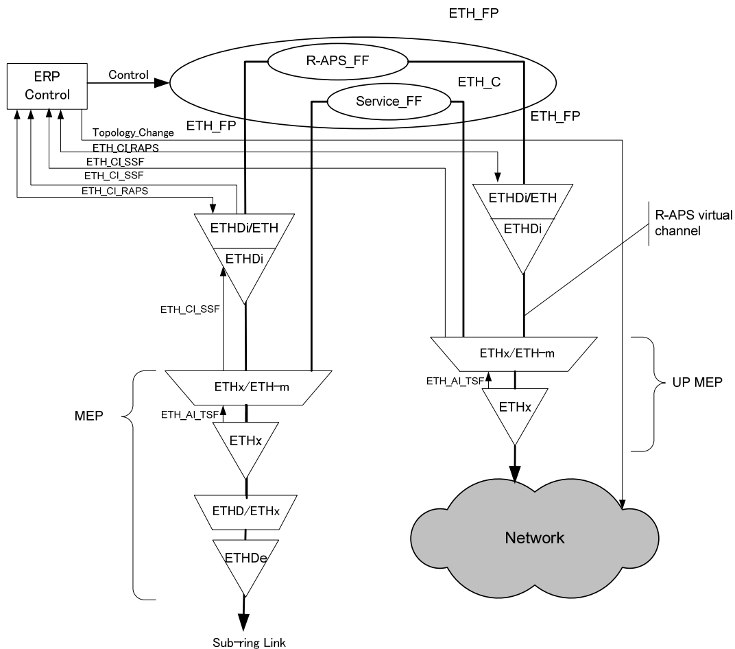
Figure X.4 – MEPs and R-APS insertion function in the interconnection node for minimization of ring segmentation in interconnected rings
