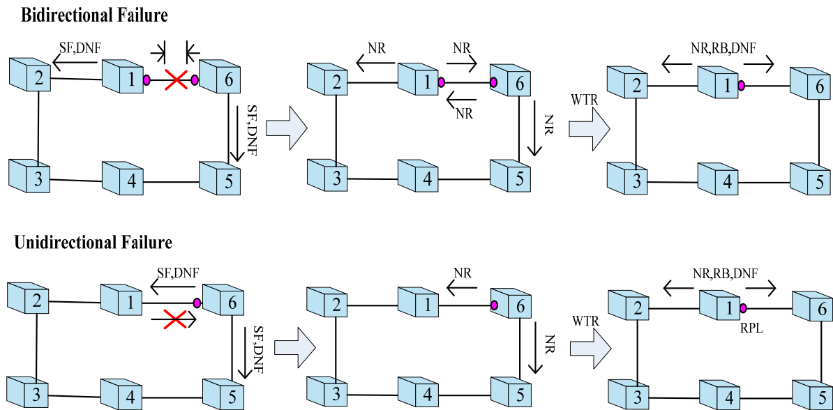
Figure VIII.3 – RPL recovery case
