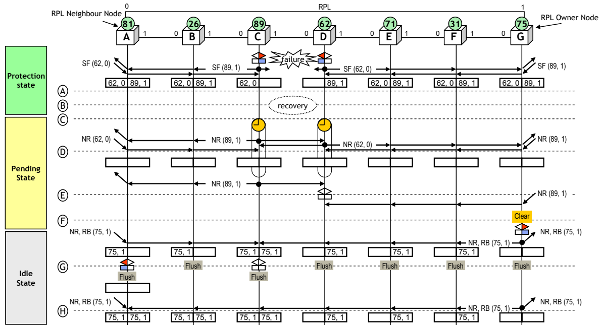
Figure III.3 – Single link failure recovery (Non-revertive operation)
