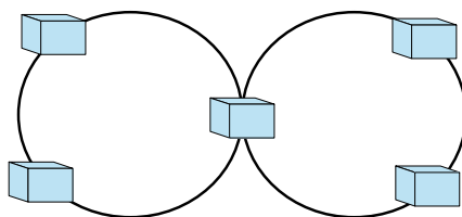
Figure II.1 – Interconnected Ethernet rings via an interconnection node
