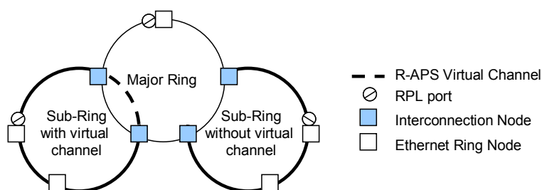
Figure 9-11 – Ring interconnection options
