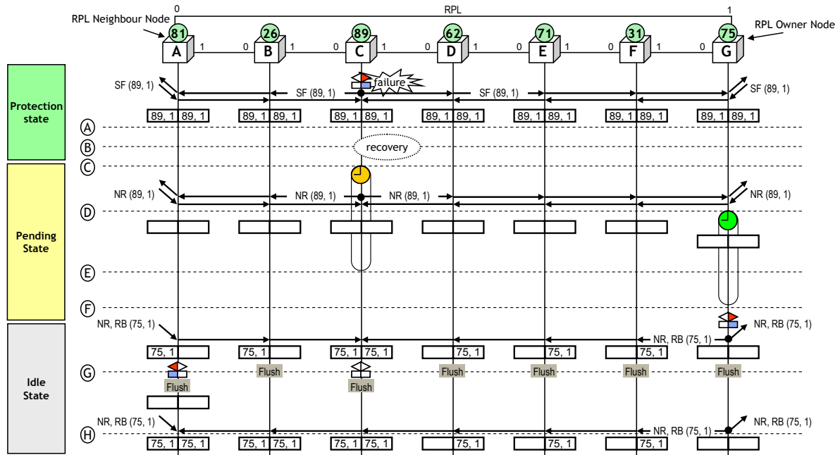
Figure III.5 – Single link failure unidirectional recovery
