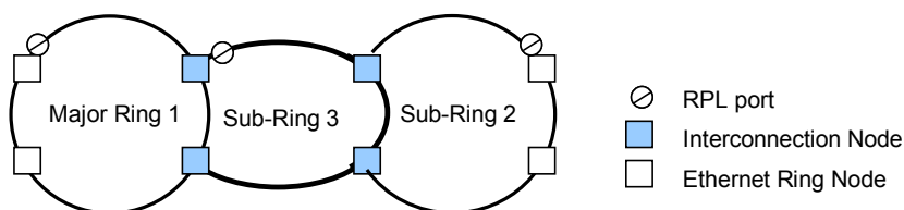
Figure 9-13 – Interconnection of two Ethernet rings with option 2
