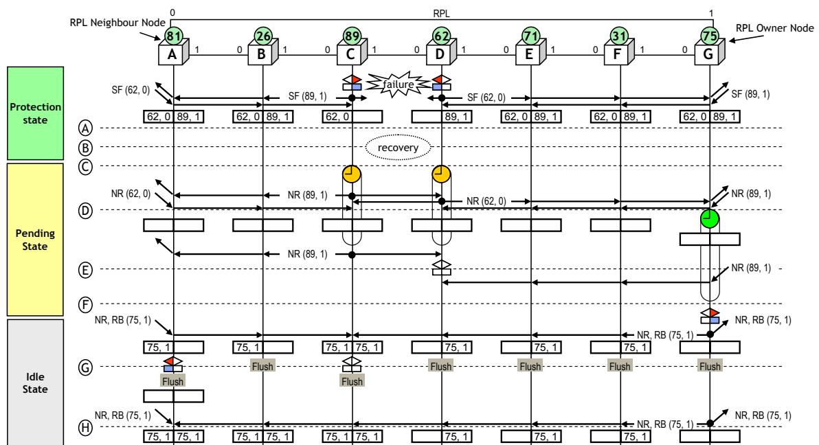
Figure III.2 – Single link failure recovery (revertive operation)
