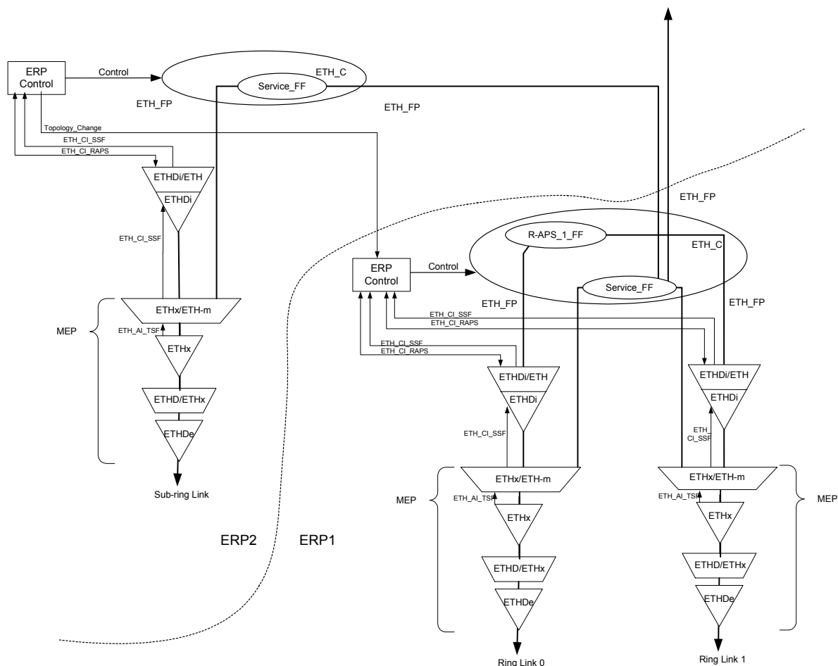
Figure 9-10 – MEPs and R-APS insertion function in a sub-ring interconnection node without R-APS virtual channel (for a sub-ring connected to major ring)
