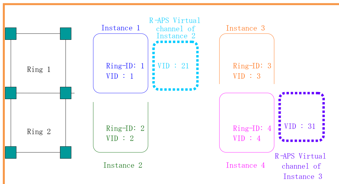
Figure VII.1 – Example 1: Different VIDs for different ERP instances; different VIDs for the ERP instances of sub-ring and an R-APS virtual channel
