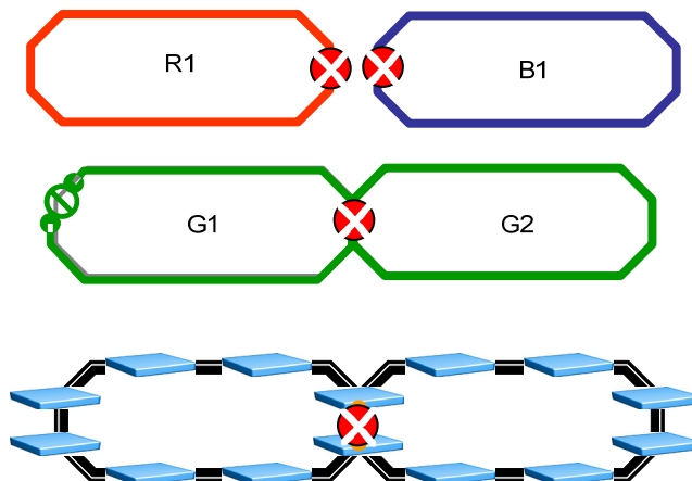
Figure VI.3 – Multiple ERP instances on interconnected physical Ethernet rings (the ring link between interconnection nodes failure condition)
