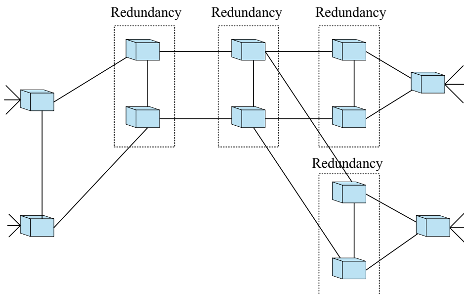
Figure II.3 – Example of multi-ring/ladder network
