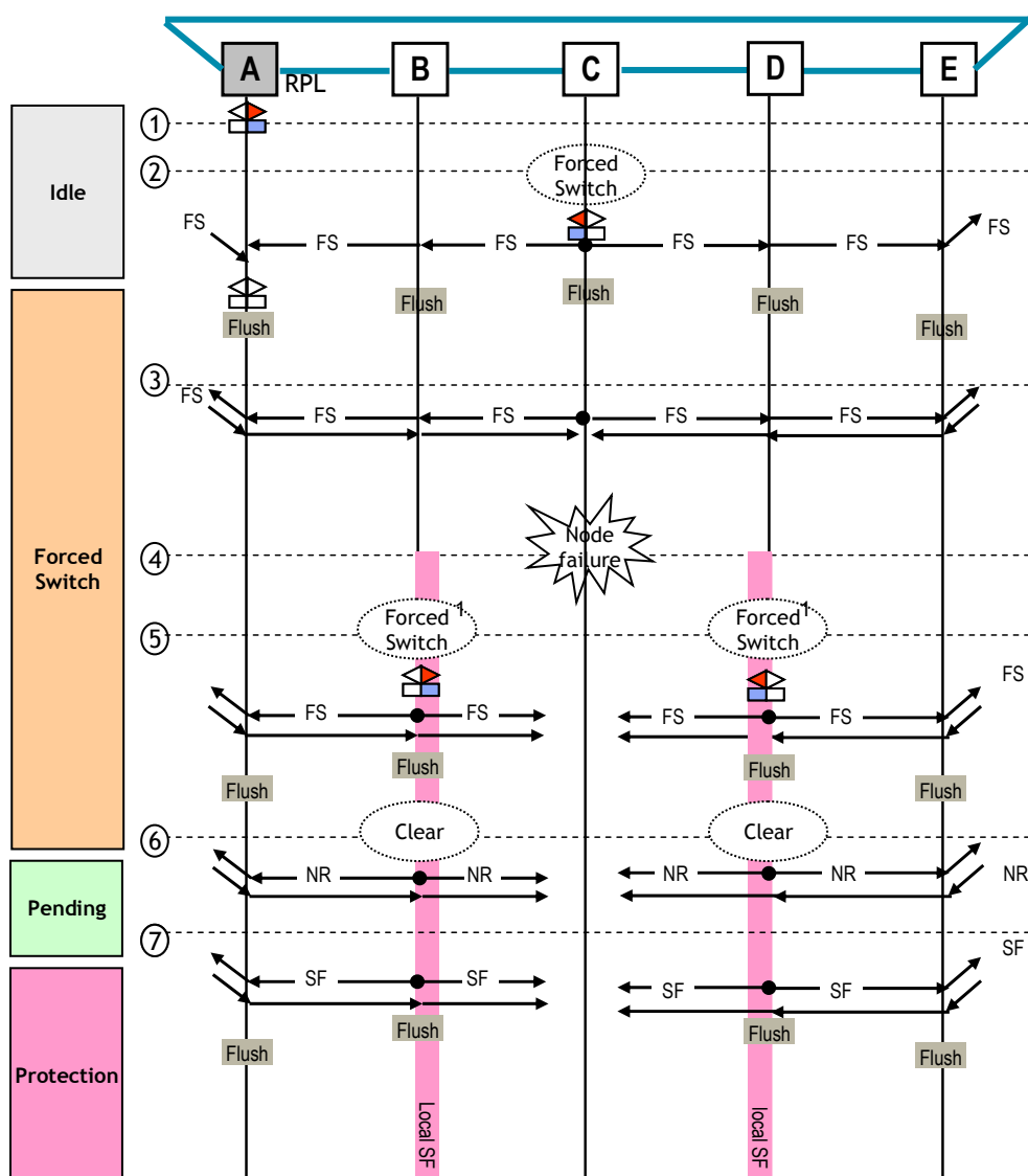
Figure IX.2 – Ethernet ring node failure scenario with management procedure
