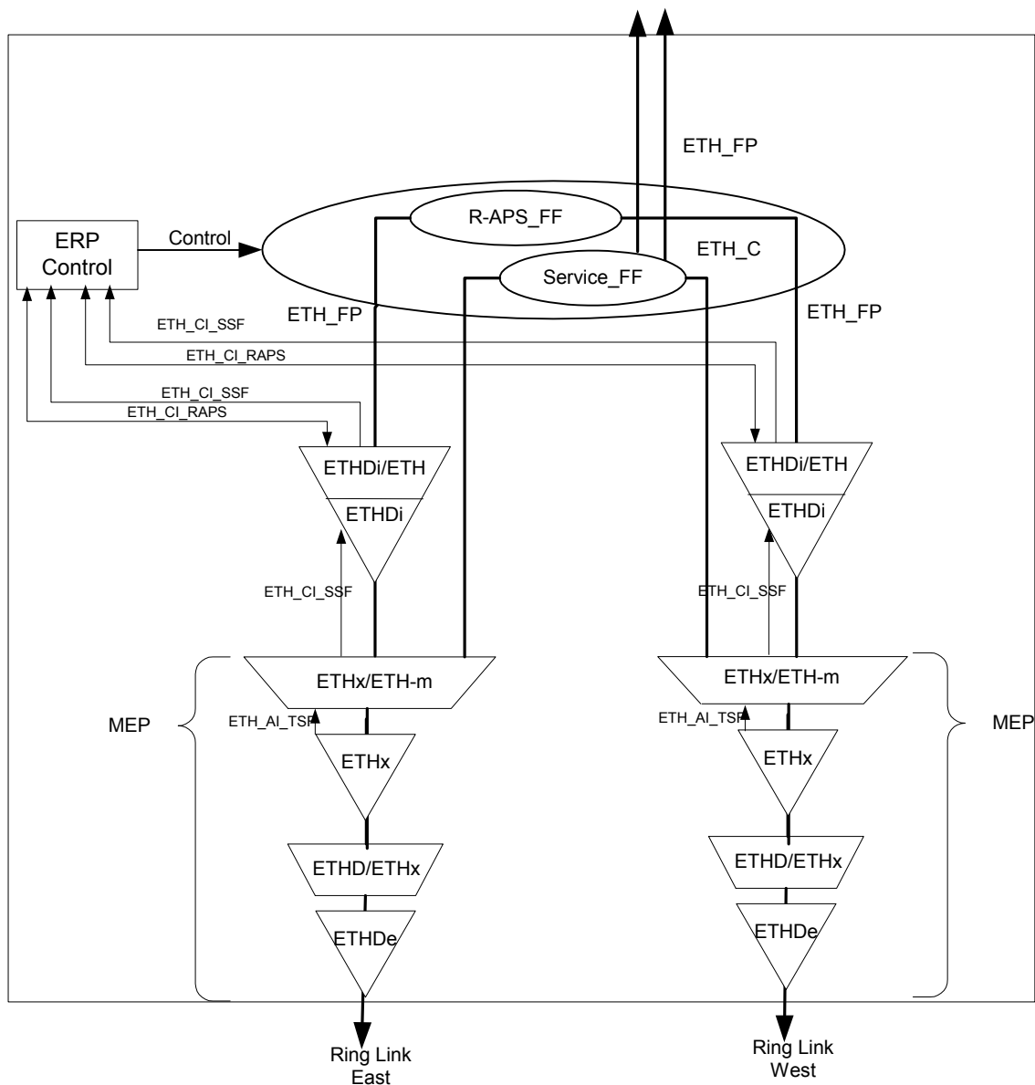
Figure 9-4 – MEPs and R-APS insertion function in Ethernet ring node (normal Ethernet ring node)
