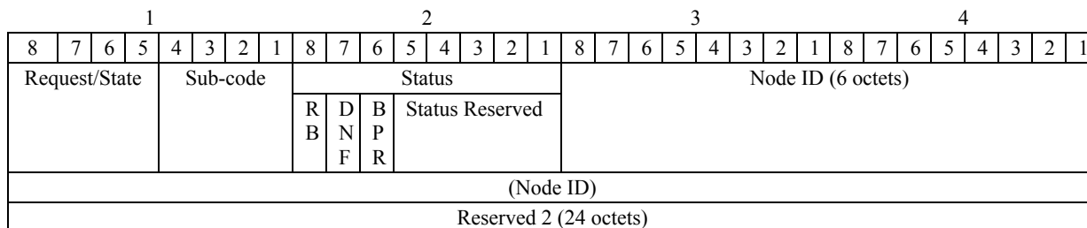
Figure 10-3 – R-APS specific information format
