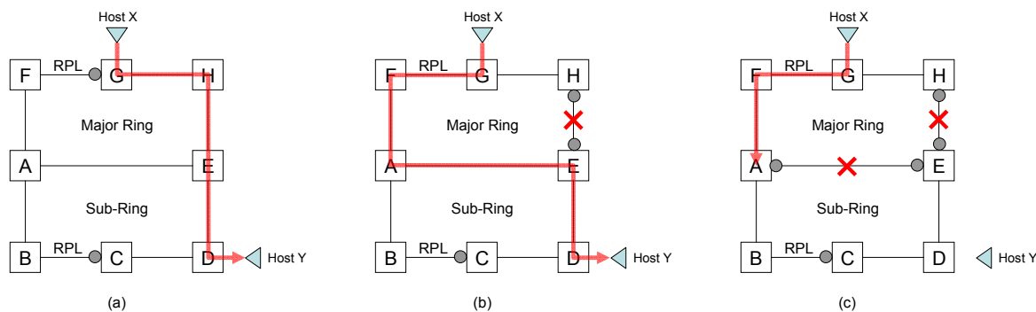
Figure X.1 – Scenario showing loss of connectivity between a major ring and a sub-ring
