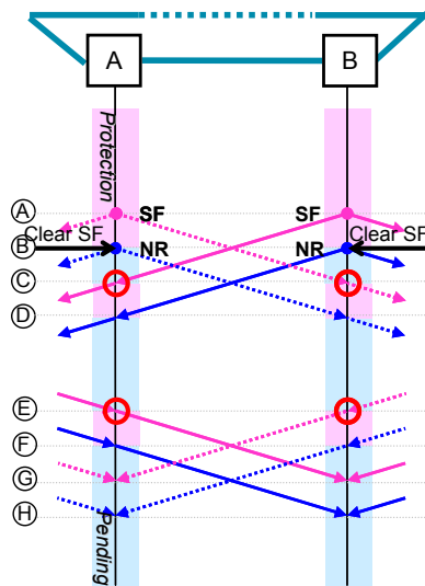
Figure IV.1 – Simultaneous requests from multiple Ethernet ring nodes
