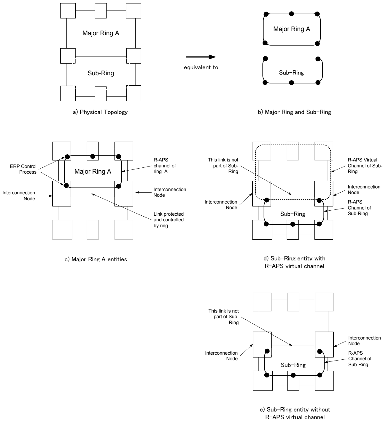
Figure V.1 – Configuration for interconnection between a major ring and a sub-ring
