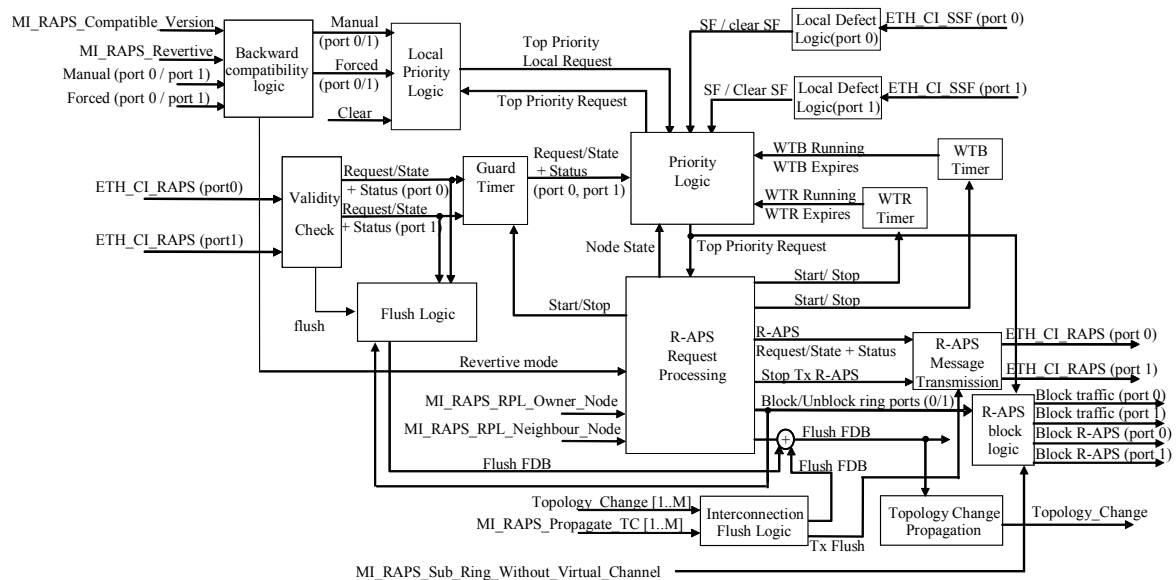
Figure 10-1 – Decomposition of the ERP control process
