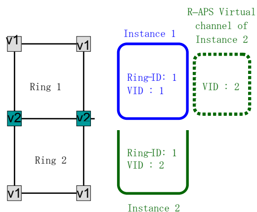
Figure VII.4 – Example 4: Co-existence of Ethernet ring nodes running ITU-T G.8032v1 and ITU-T G.8032v2 (with an R-APS virtual channel)
