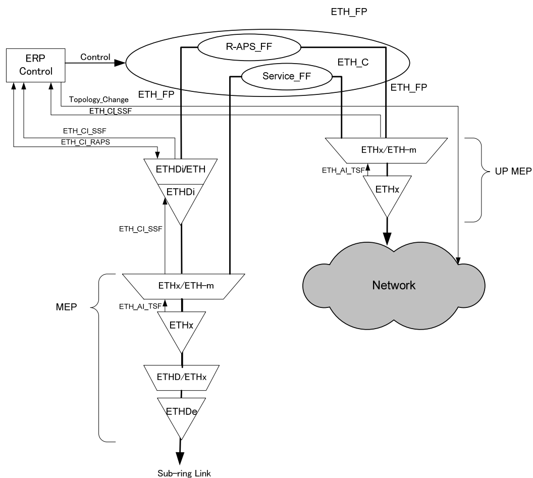
Figure X.5 – MEPs and R-APS insertion function in the interconnection node without R-APS virtual channel for minimization of ring segmentation in interconnected rings
