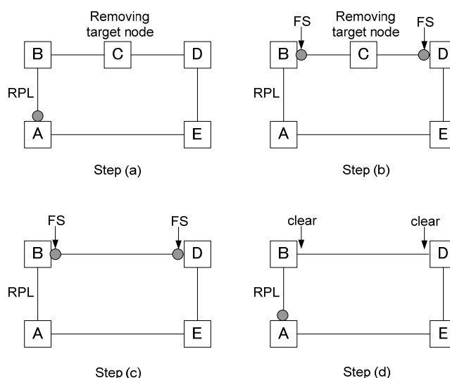
Figure IX.1 – Example procedure for removing an Ethernet ring node
