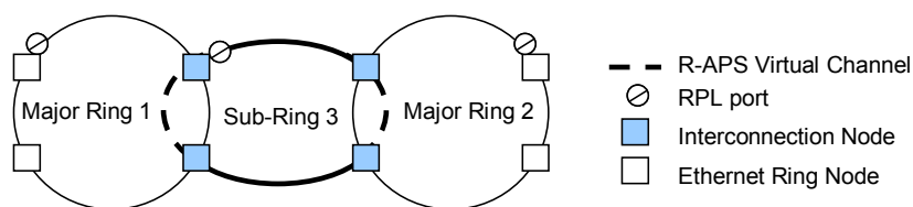
Figure 9-12 – Interconnection of two Ethernet rings with option 1
