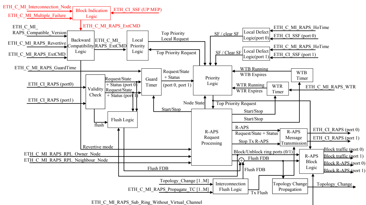
Figure X.6 – ERP control process for minimization of ring segmentation in interconnected rings
