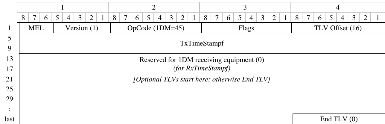
Figure 9.14-1 – 1DM PDU format
