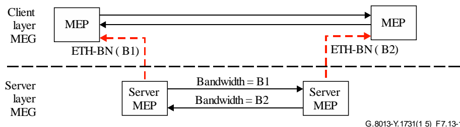
Figure 7.13-1 – Example of ETH-BN transmission
