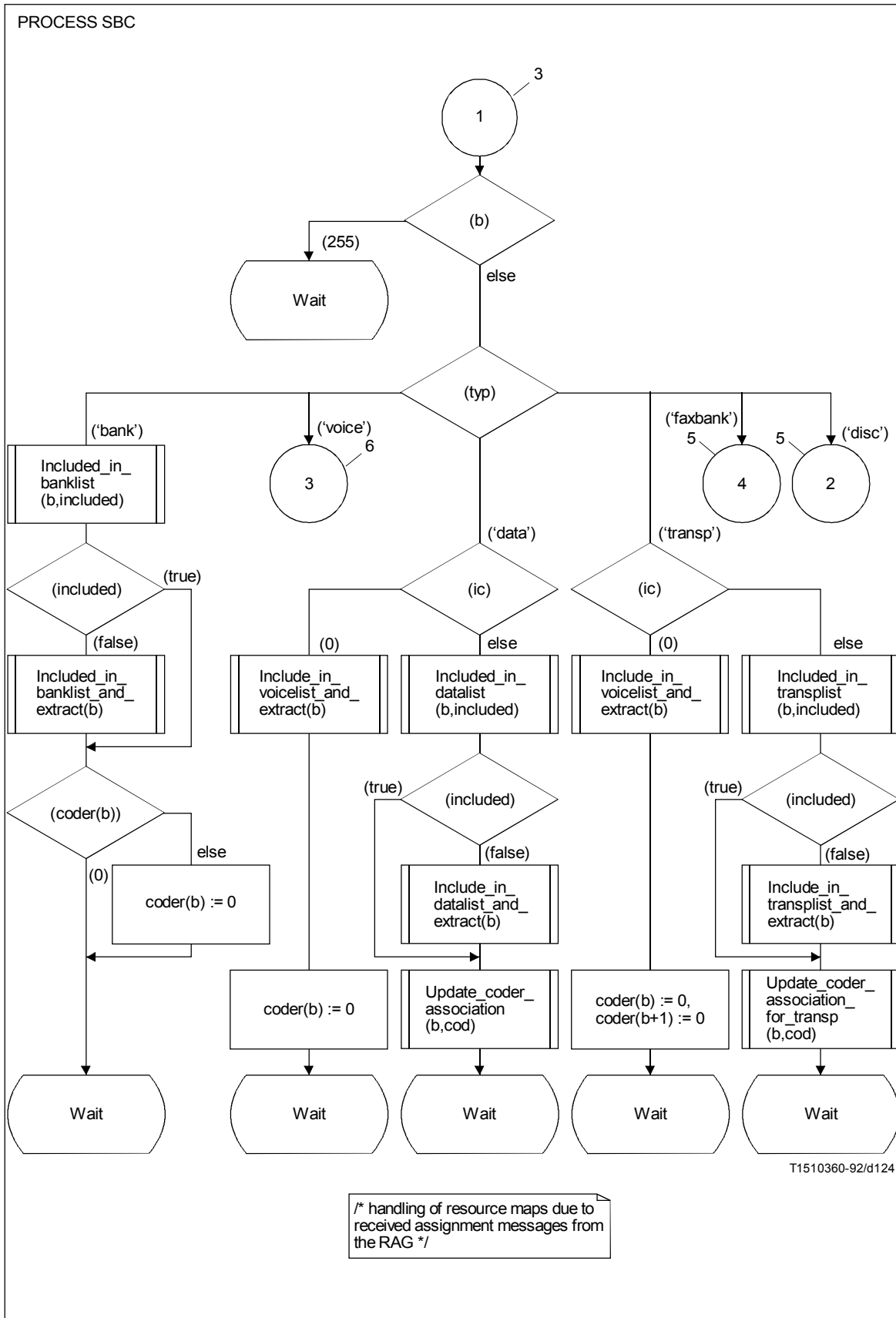
FIGURE A.26/G.763 (sheet 4 of 6)
