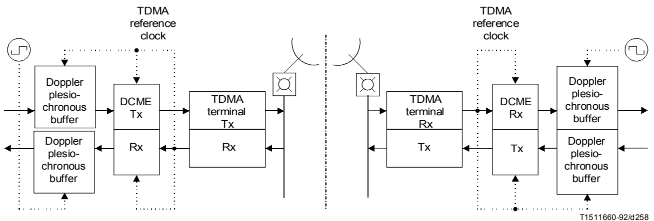
FIGURE B.13/G.763 DCME synchronous operation (between two plesiochronous networks)
