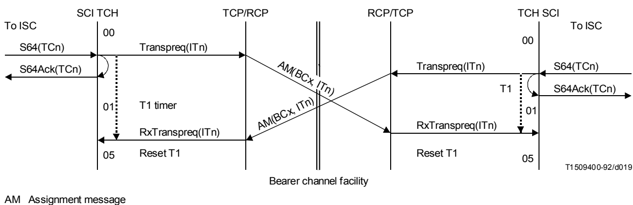
FIGURE 20/G.763 Sequence chart for 64 kbit/s circuit establishment in dual-seizure situation
