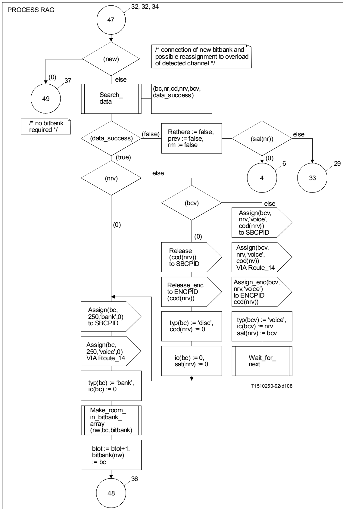
FIGURE A.23/G.763 (sheet 35 of 45)
