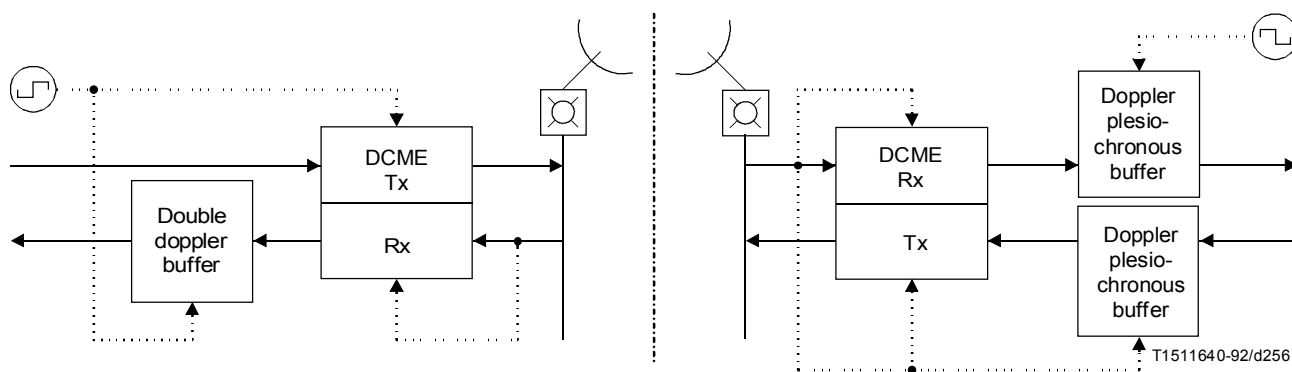
FIGURE B.11/G.763 DCME synchronous loop operation (between two plesiochronous networks)
