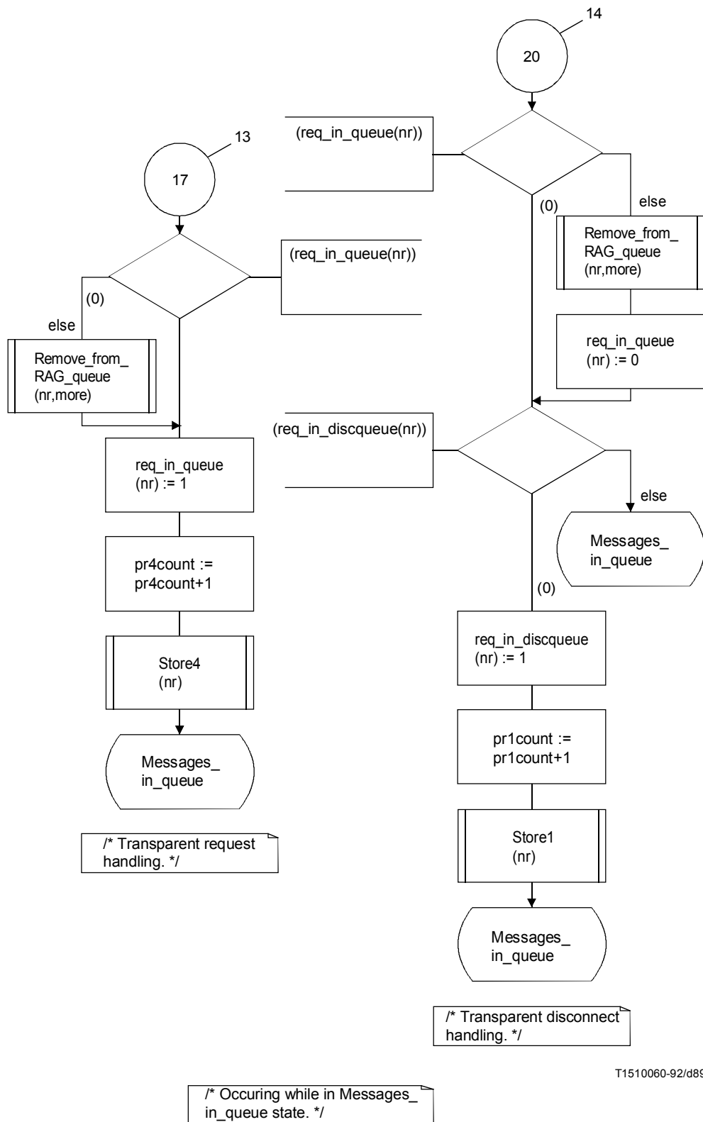
FIGURE A.23/G.763 (sheet 16 of 45)
