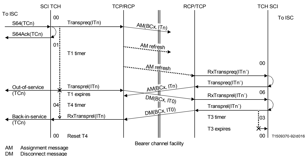
FIGURE 17/G.763 Sequence chart for automatic recovery after unsuccessful (delayed) 64 kbit/s circuit establishment
