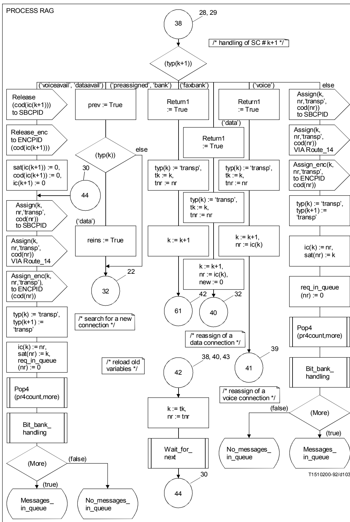
FIGURE A.23/G.763 (sheet 30 of 45)
