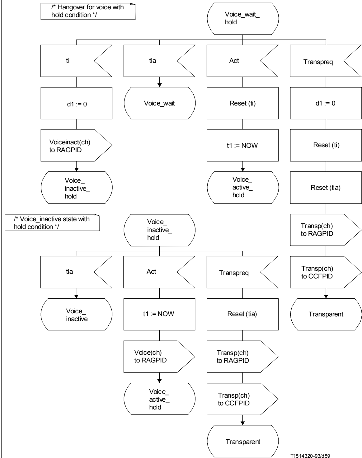
FIGURE A.19/G.763 (sheet 6 of 17)
