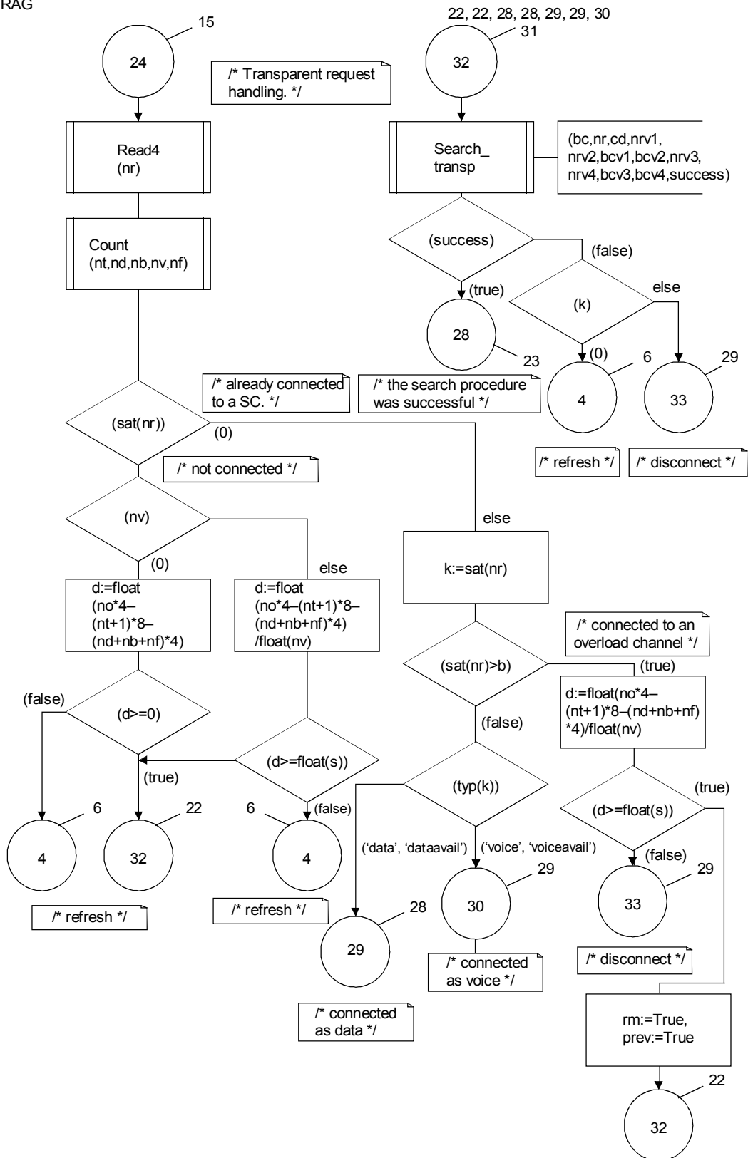
FIGURE A.23/G.763 (sheet 22 of 45)
