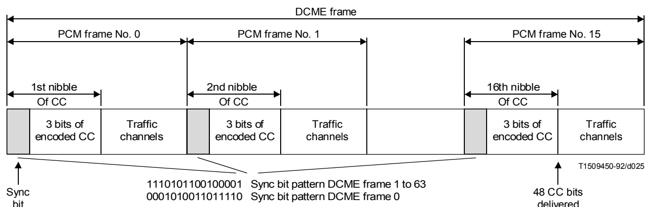
FIGURE 26/G.763 CC message transmission scheme
