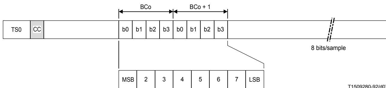
FIGURE 7/G.763 64 kbit/s bearer channel (8 bits/sample)
