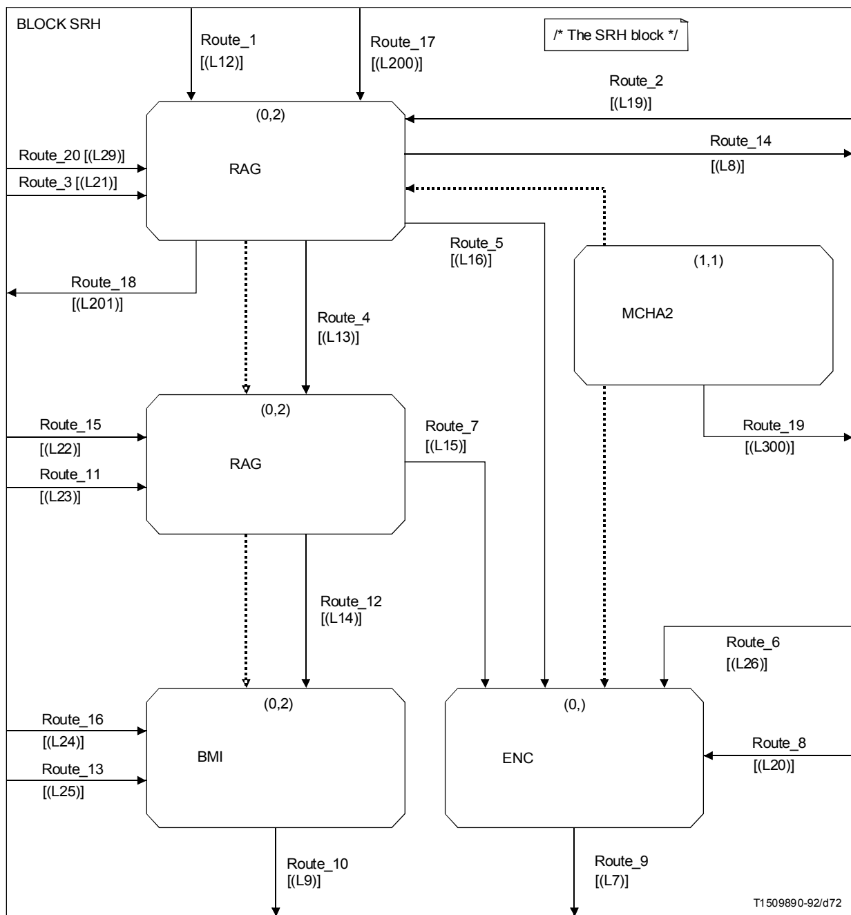
FIGURE A.21/G.763 Block SRH
