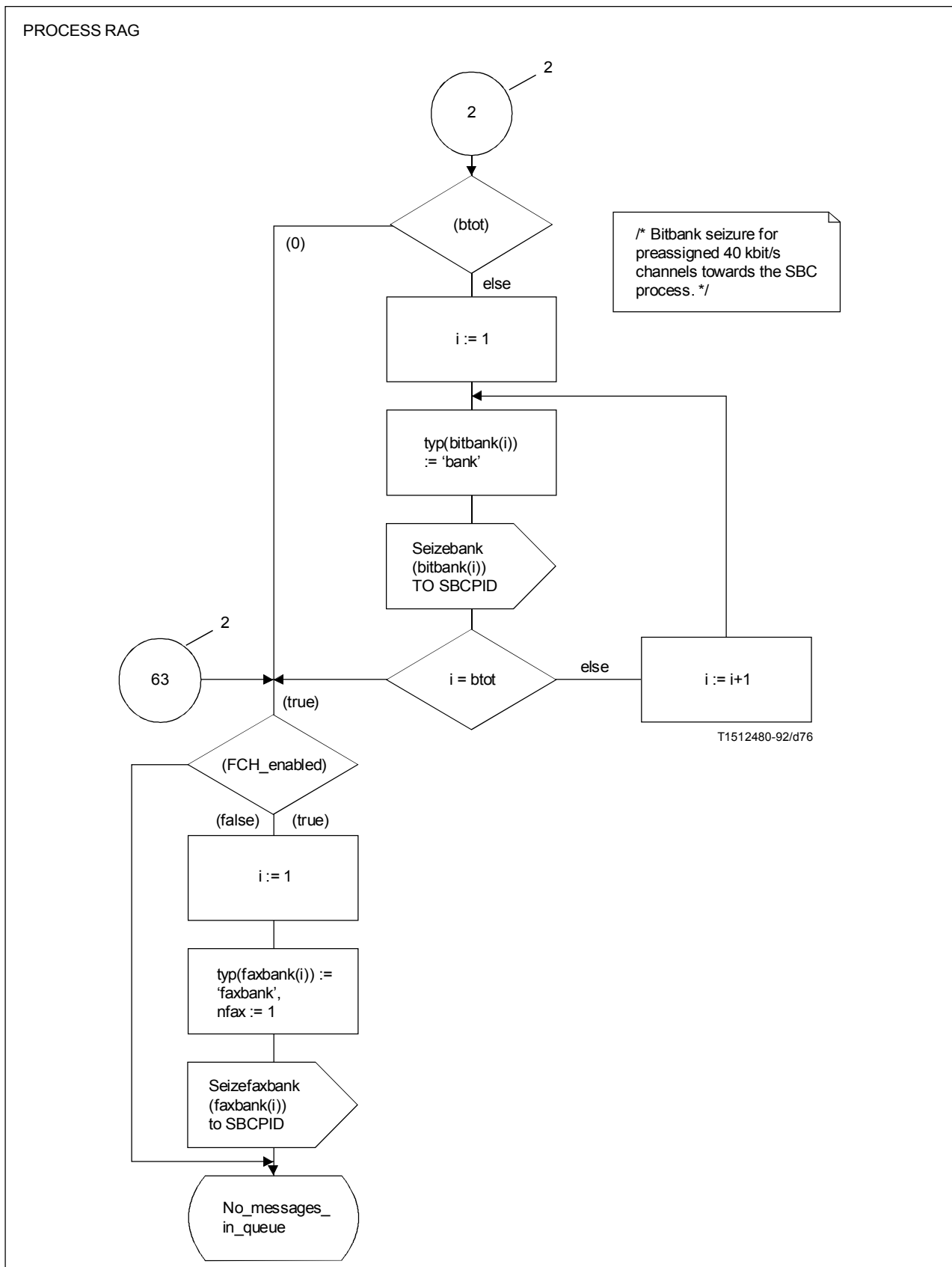
FIGURE A.23/G.763 (sheet 3 of 45)
