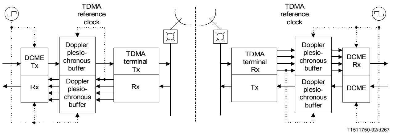
FIGURE B.22/G.763 DCME buffered plesiochronous operation (between two plesiochronous networks)
