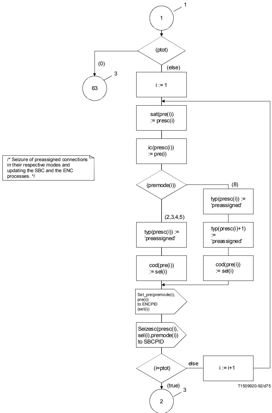
FIGURE A.23/G.763 (sheet 2 of 45)
