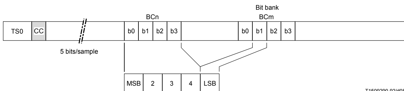
FIGURE 8/G.763 40 kbit/s bearer channel (5 bits/sample)
