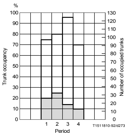
FIGURE 6 DCOA profile, trunk side
