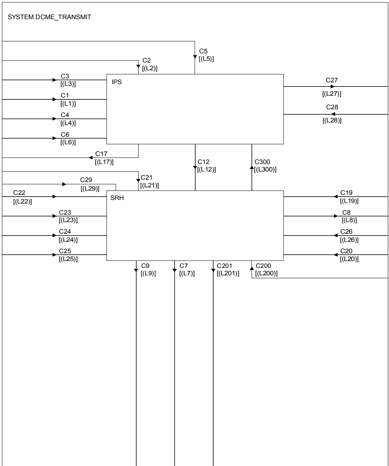
FIGURE A.15/G.763 SYSTEM DCME_TRANSMIT
