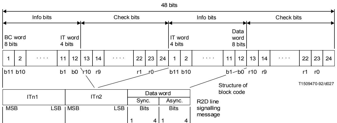
FIGURE 28/G.763 R2D line signalling message format for CC
