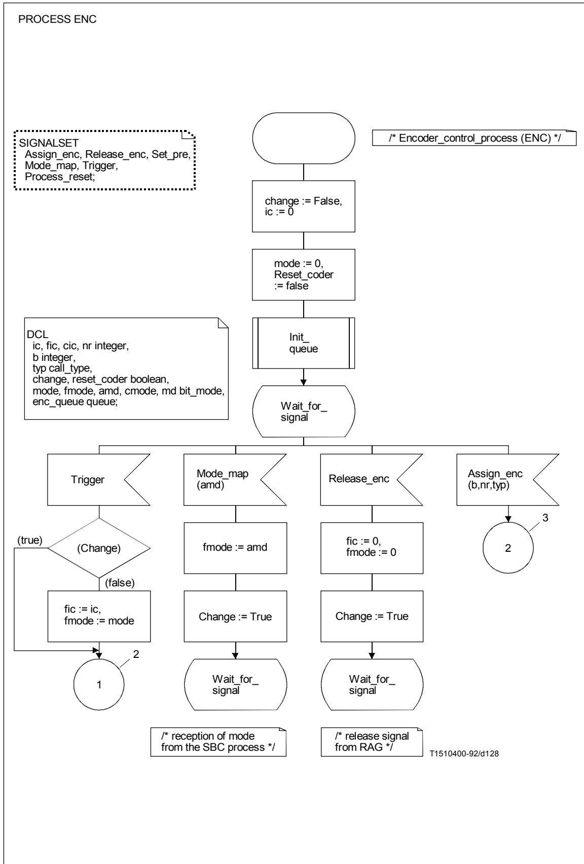
FIGURE A.28/G.763 (sheet 1 of 4)
