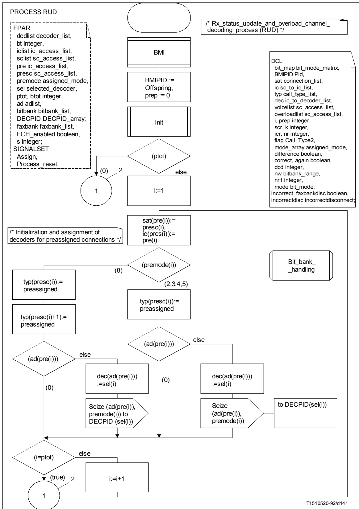
FIGURE A.35/G.763 (sheet 1 of 83)
