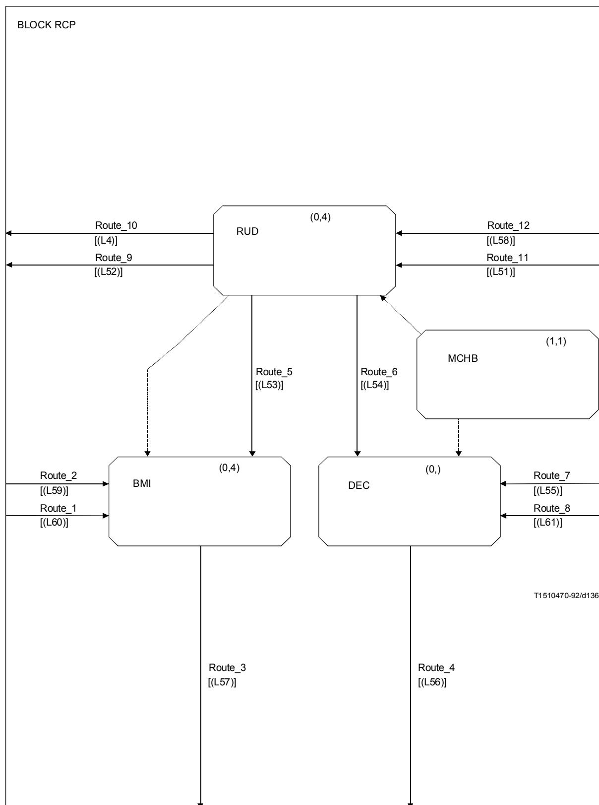
FIGURE A.32/G.763 BLOCK RCP
