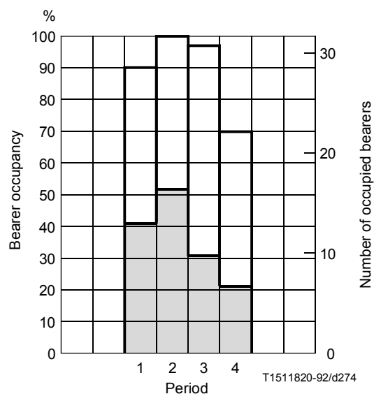
FIGURE 7 DCOA profile, bearer side
