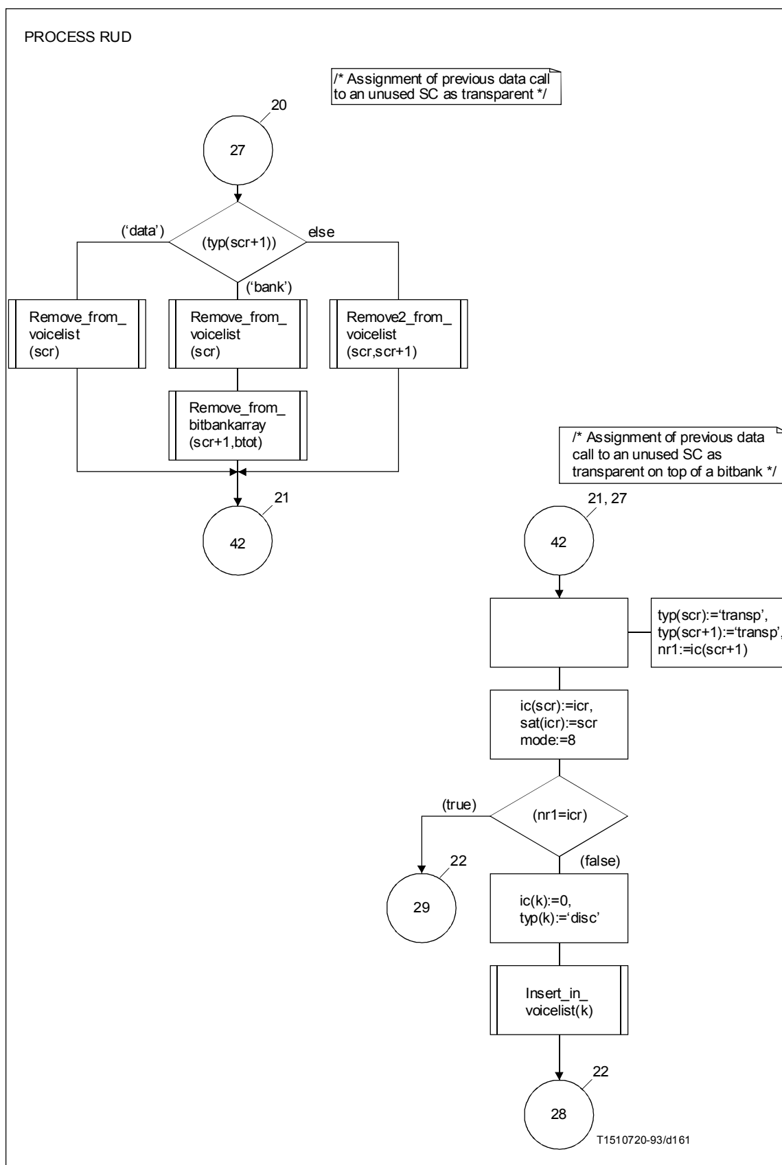
FIGURE A.35/G.763 (sheet 21 of 83)
