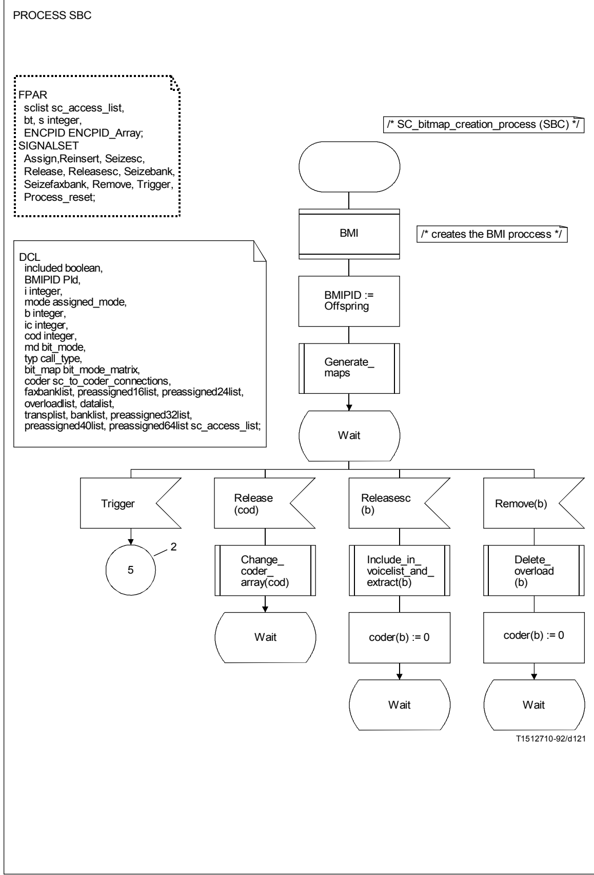
FIGURE A.26/G.763 (sheet 1 of 6)
