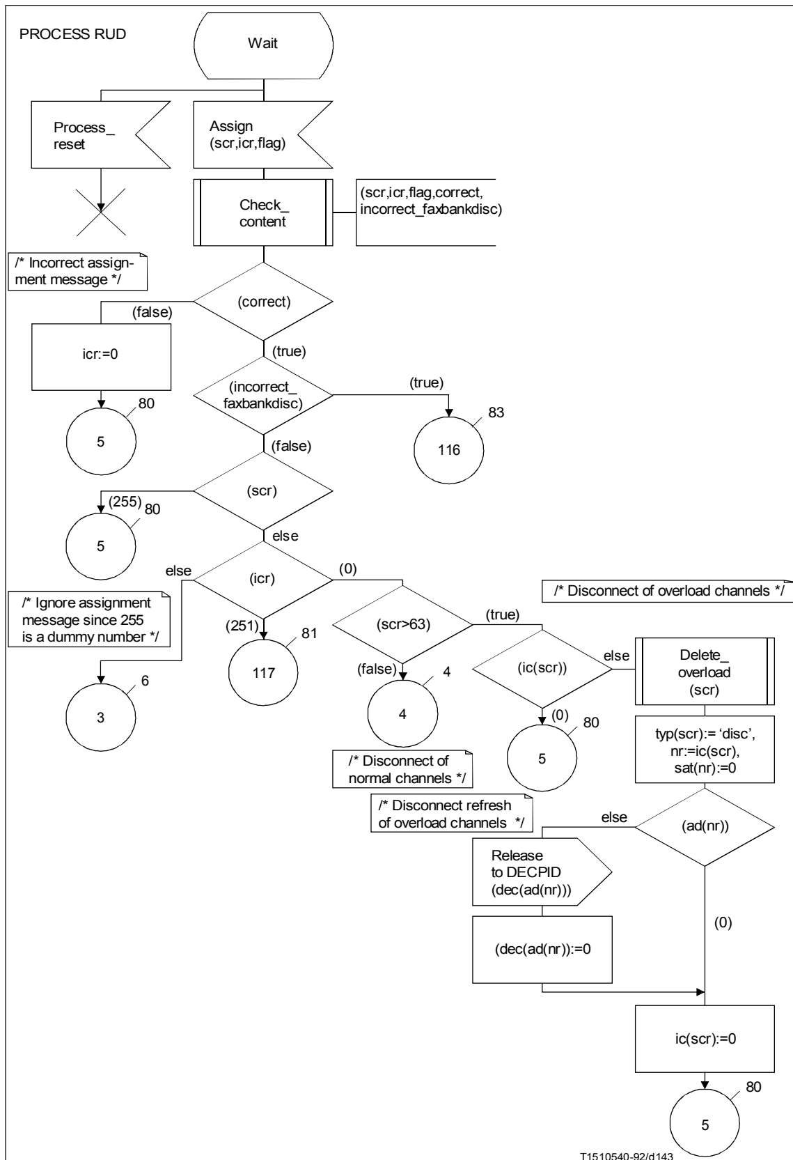
FIGURE A.35/G.763 (sheet 3 of 83)
