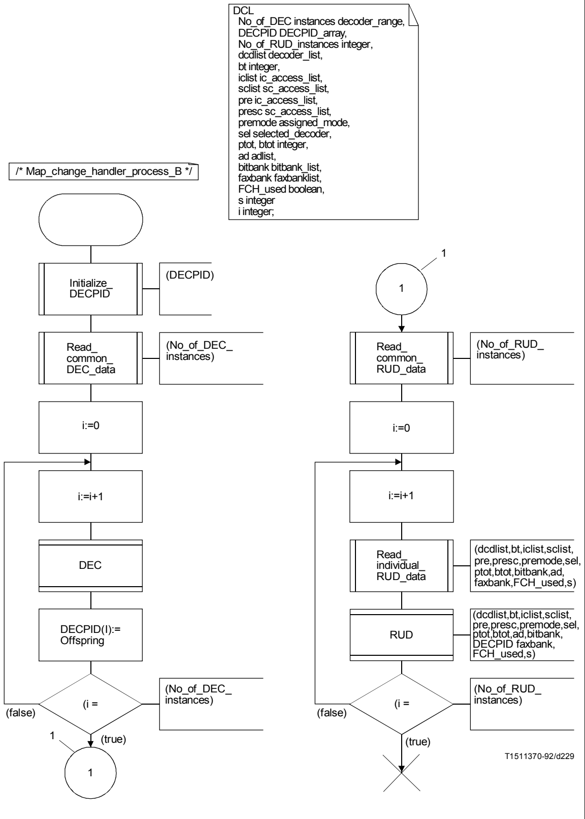
FIGURE A.39/G.763 PROCESS MCHB
