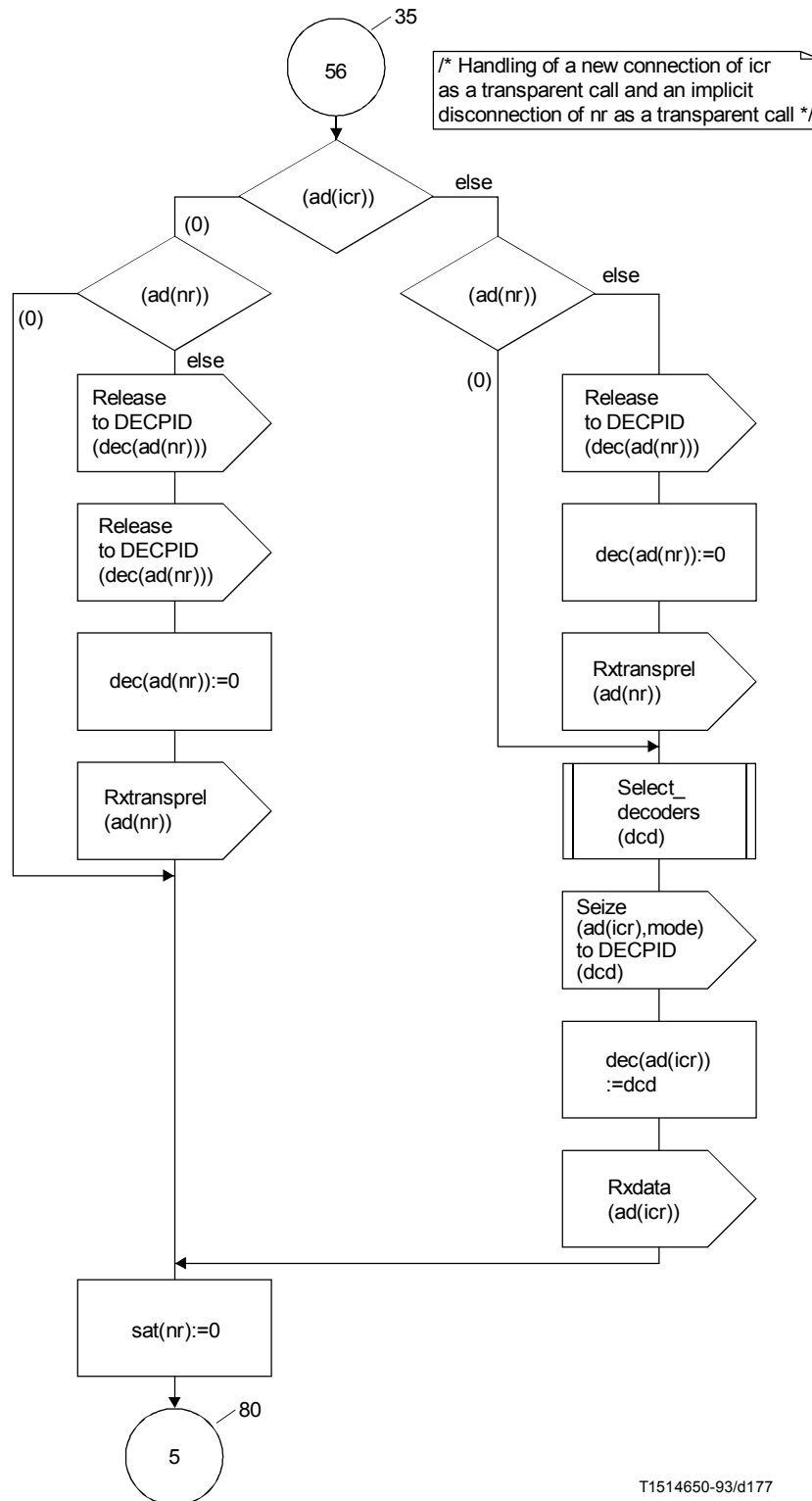
FIGURE A.35/G.763 (sheet 37 of 83)
