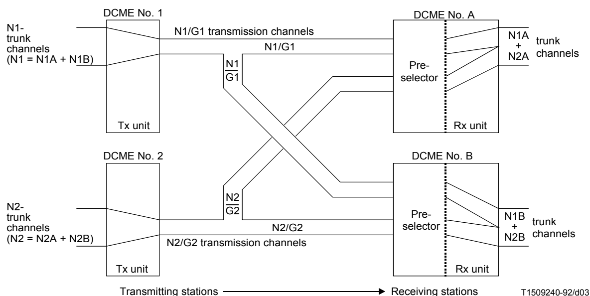
FIGURE 3/G.763 Multi-destination mode (only one direction shown)
