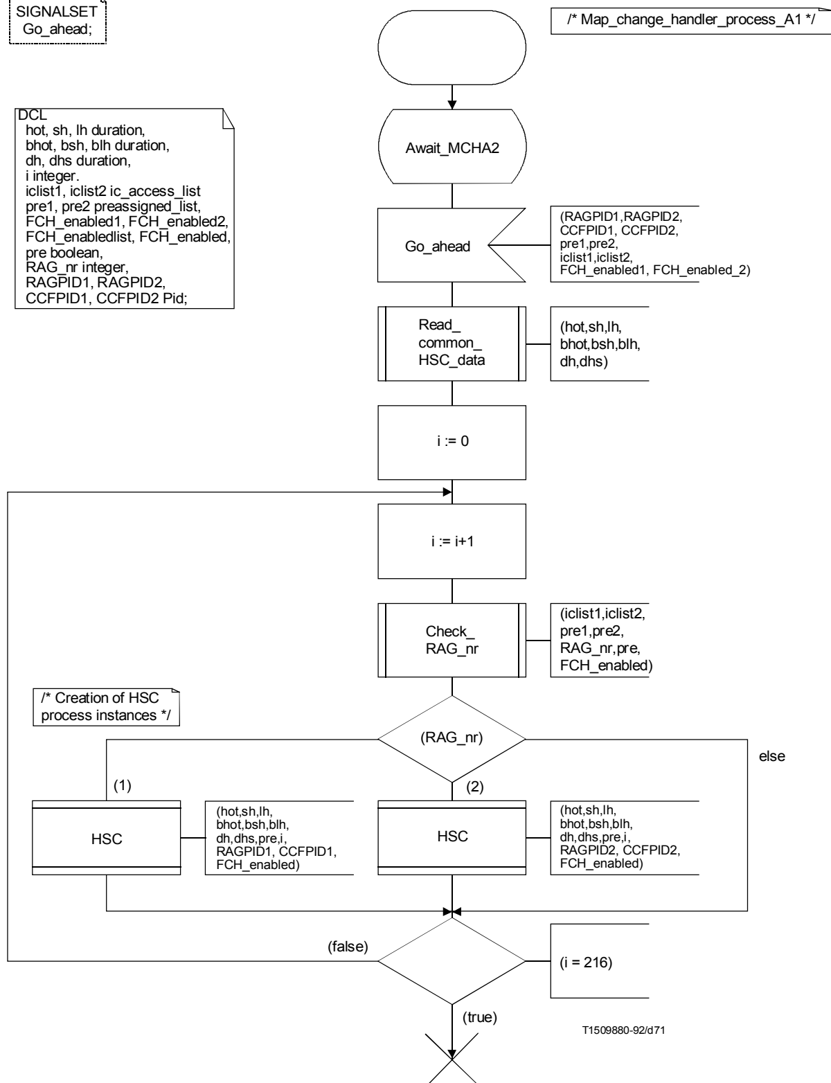
FIGURE A.20/G.763 PROCESS MCHA1
