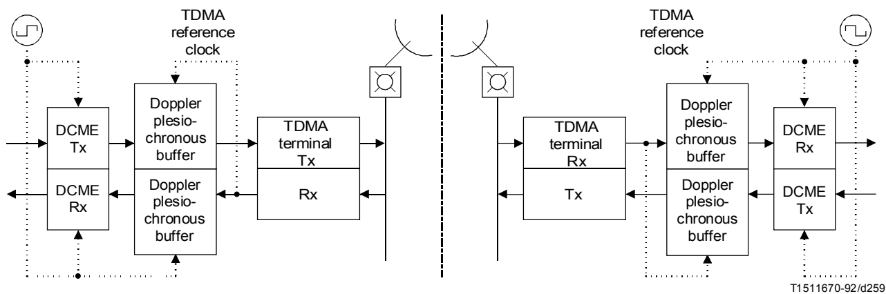
FIGURE B.14/G.763 DCME buffered plesiochronous operation (between two plesiochronous networks)
