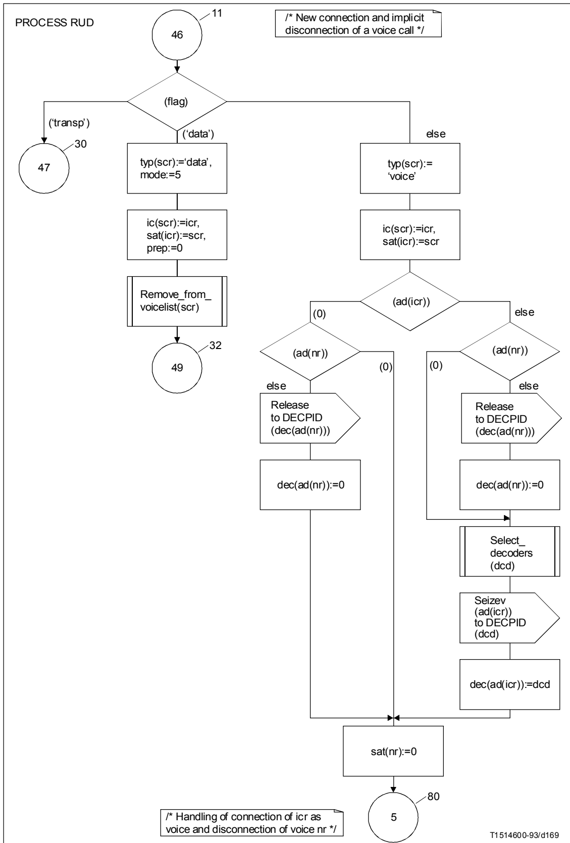
FIGURE A.35/G.763 (sheet 29 of 83)
