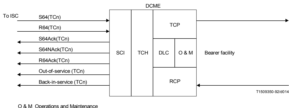
FIGURE 15/G.763 Block interaction diagram for 64 kbit/s circuit handling
