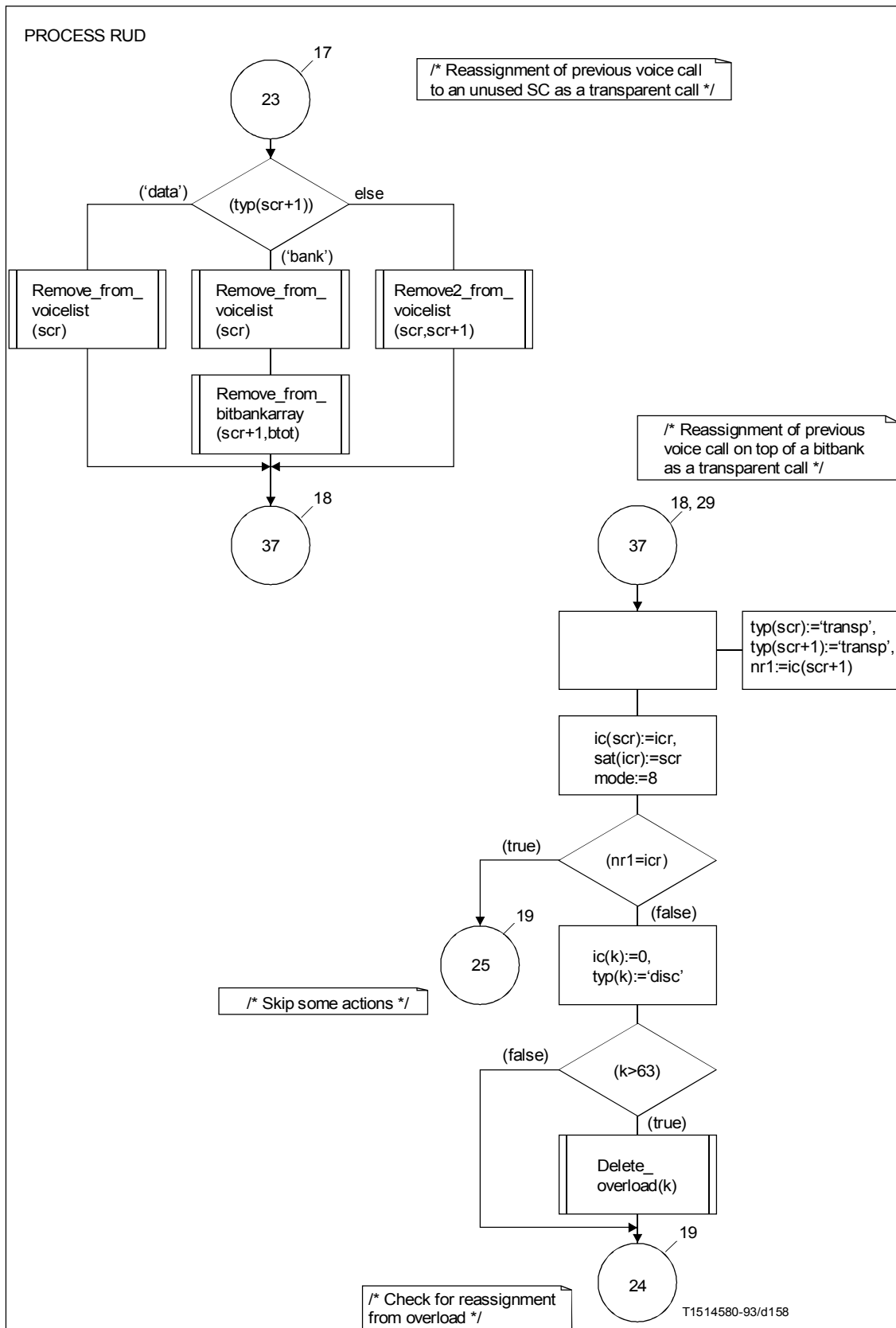
FIGURE A.35/G.763 (sheet 18 of 83)
