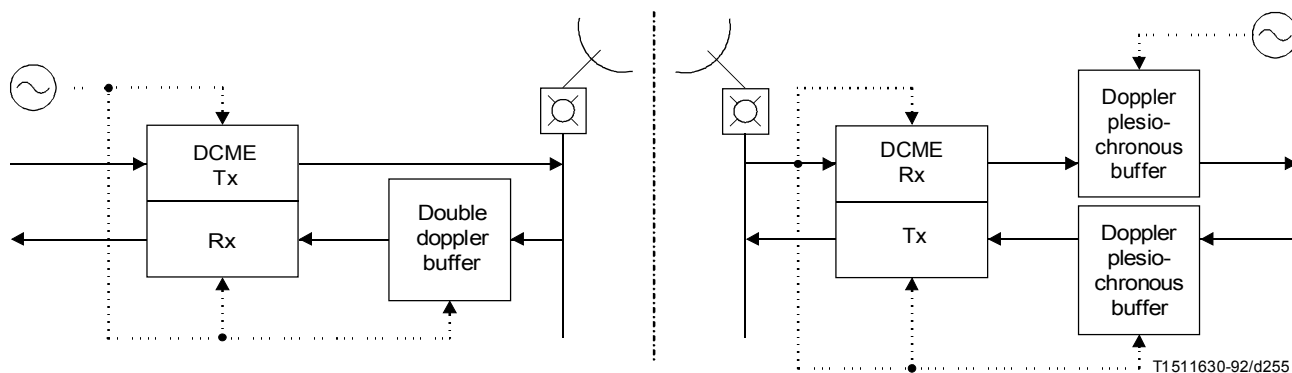
FIGURE B.10/G.763 DCME synchronous loop operation (between two plesiochronous networks)
