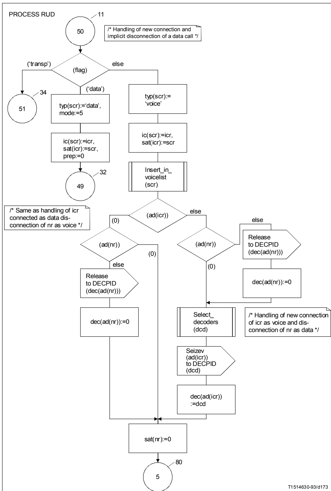
FIGURE A.35/G.763 (sheet 33 of 83)
