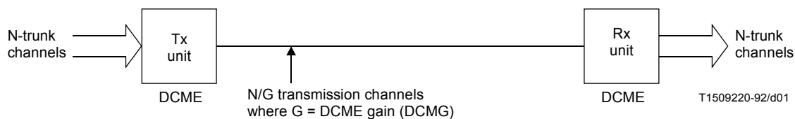
FIGURE 1/G.763 Point-to-point mode (only one direction shown)
