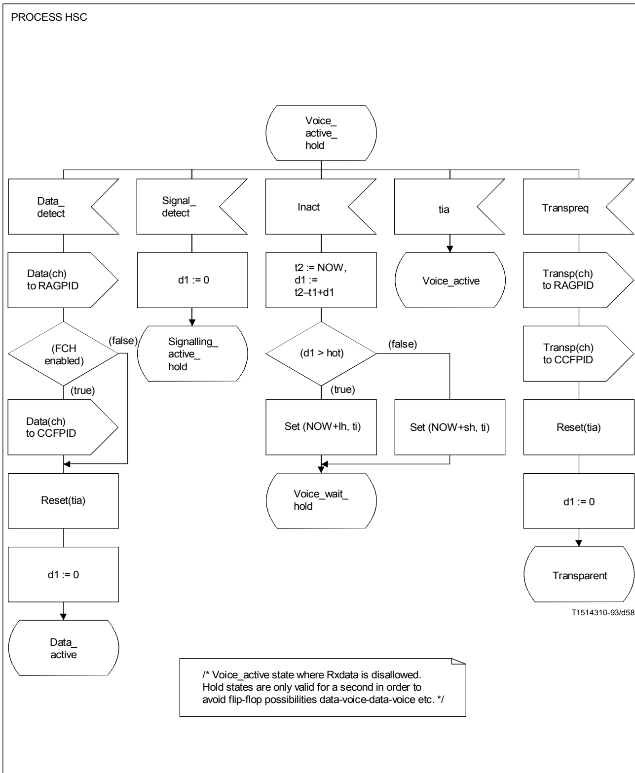
FIGURE A.19/G.763 (sheet 5 of 17)
