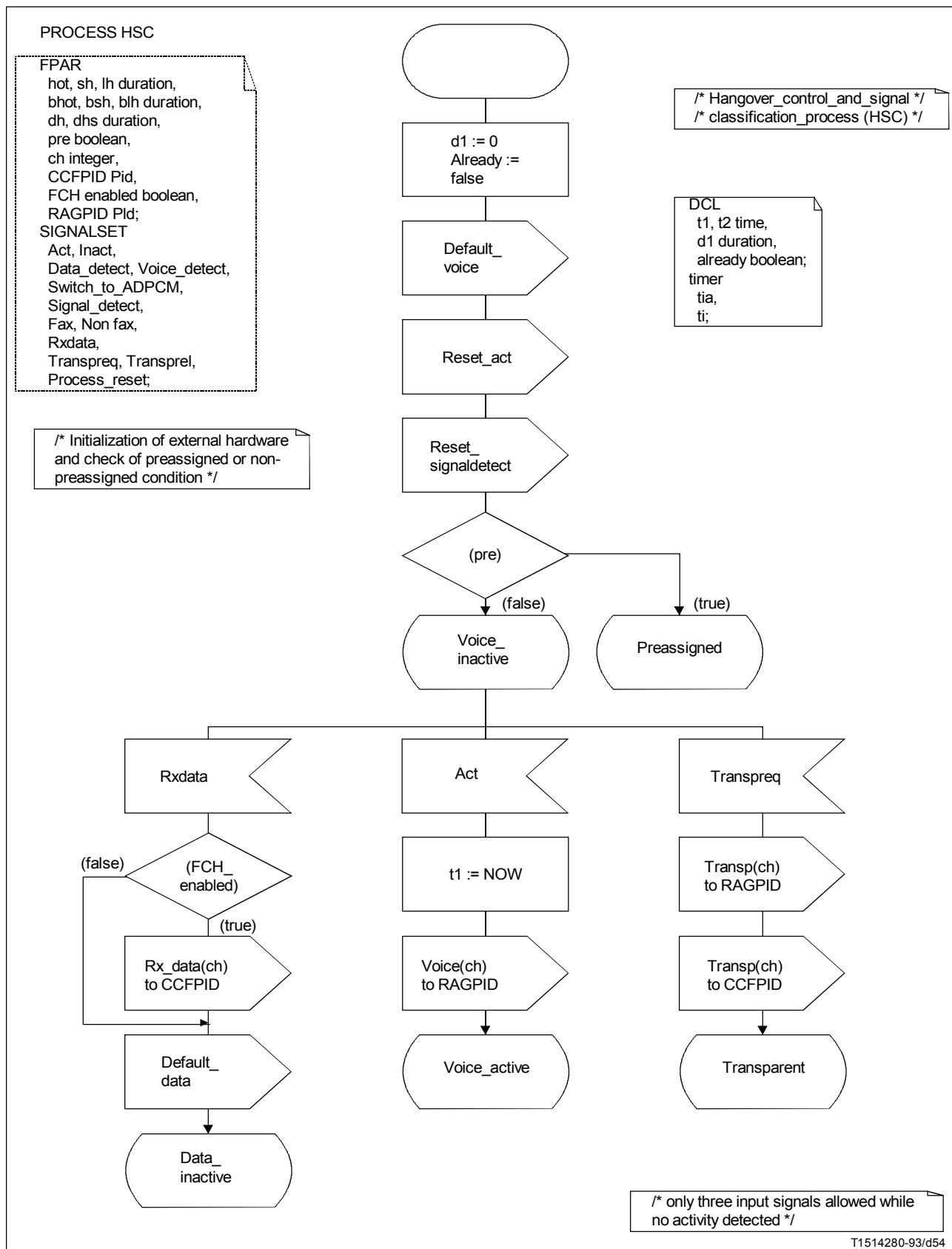
FIGURE A.19/G.763 (sheet 1 of 17)
