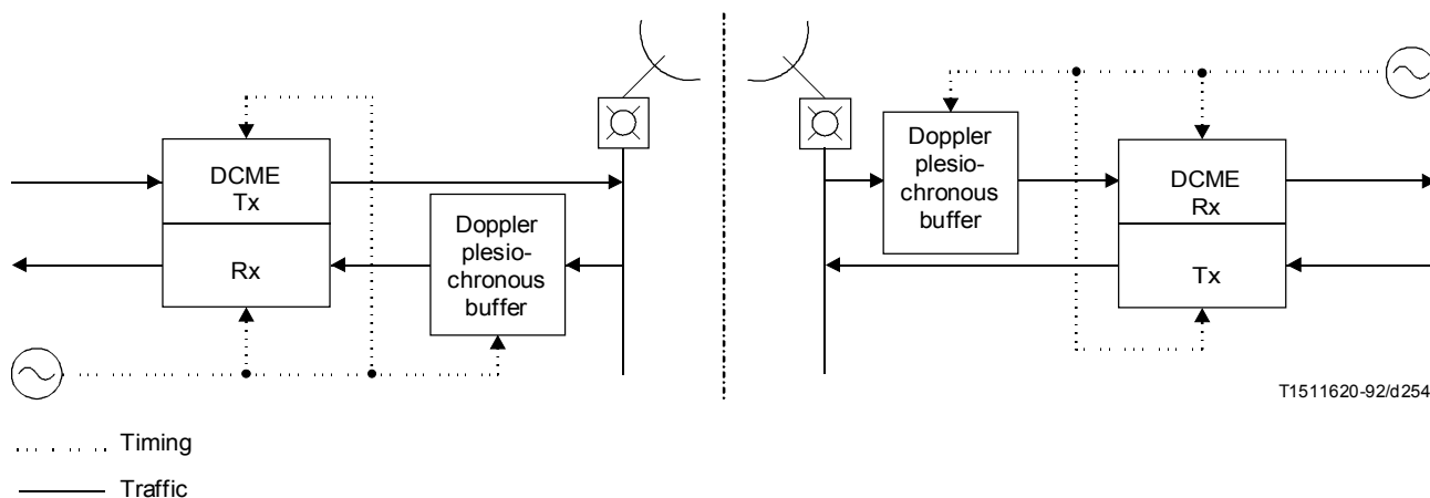
FIGURE B-9/G.763 DCME buffered plesiochronous operation (between two plesiochronous networks)
