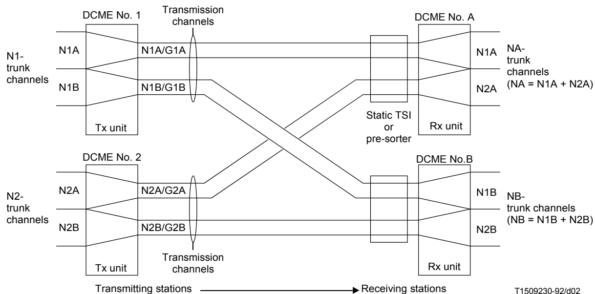
FIGURE 2/G.763 Multi-clique mode (only one direction shown)
