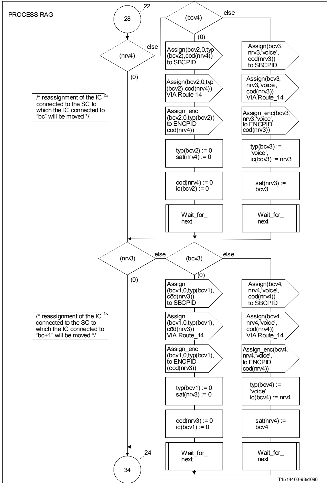
FIGURE A.23/G.763 (sheet 23 of 45)
