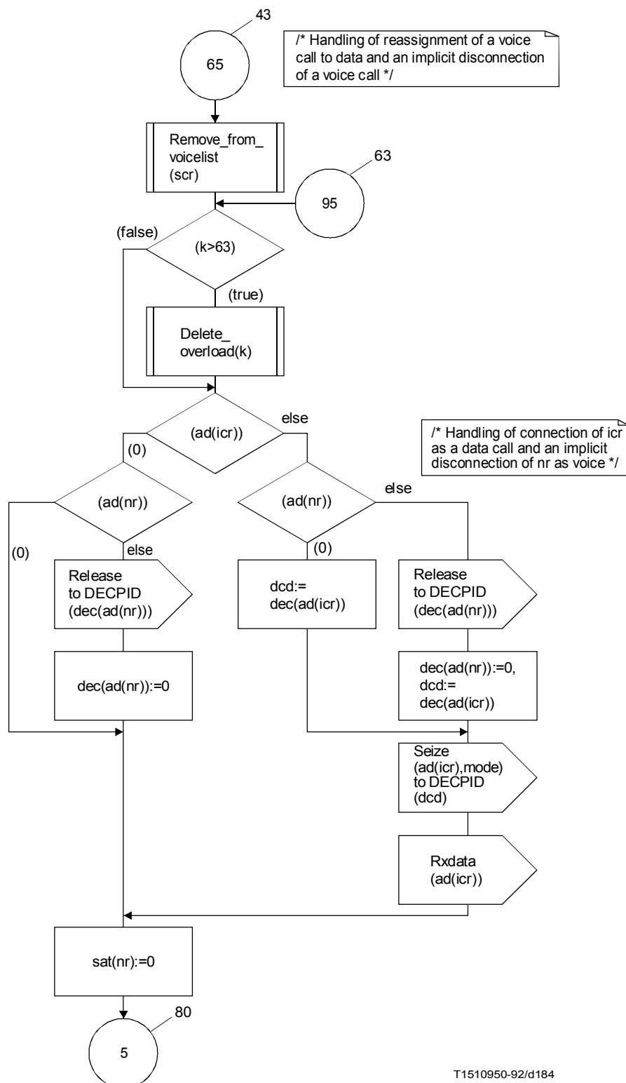
FIGURE A.35/G.763 (sheet 44 of 83)
