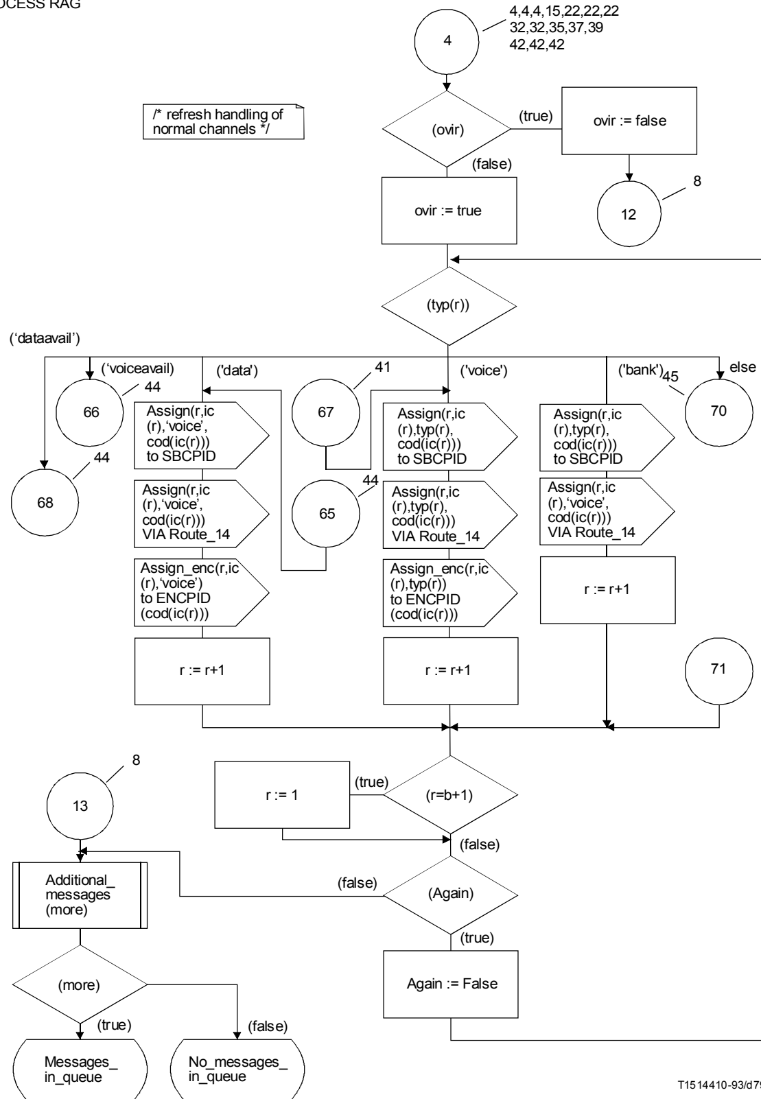
FIGURE A.23/G.763 (sheet 6 of 45)
