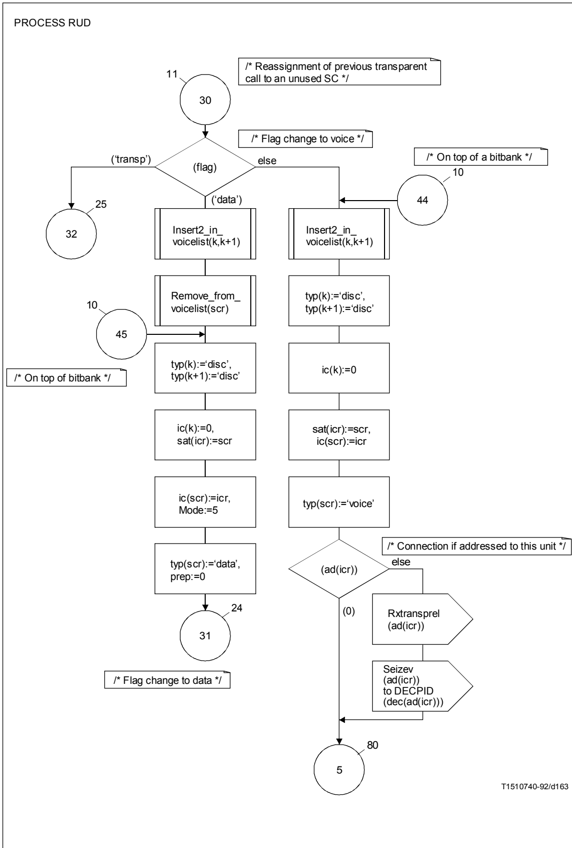
FIGURE A.35/G.763 (sheet 23 of 83)
