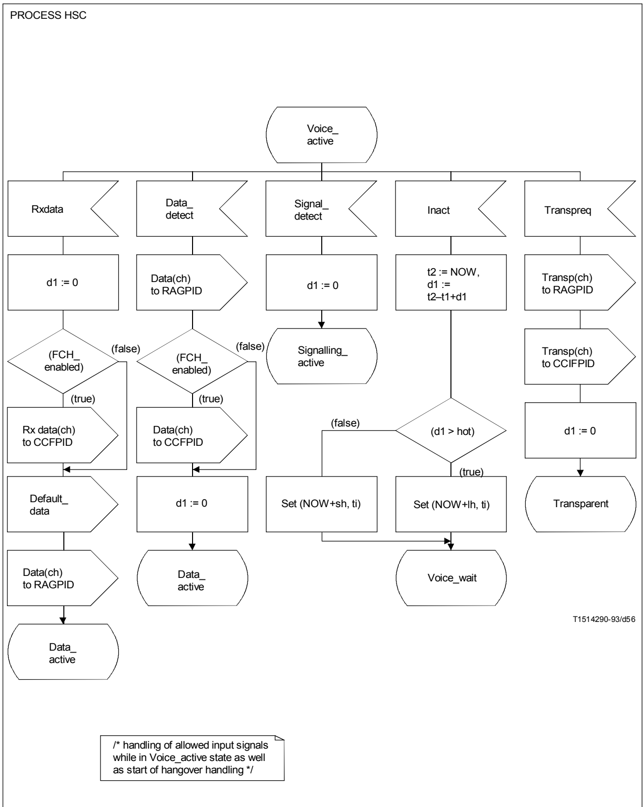
FIGURE A.19/G.763 (sheet 3 of 17)
