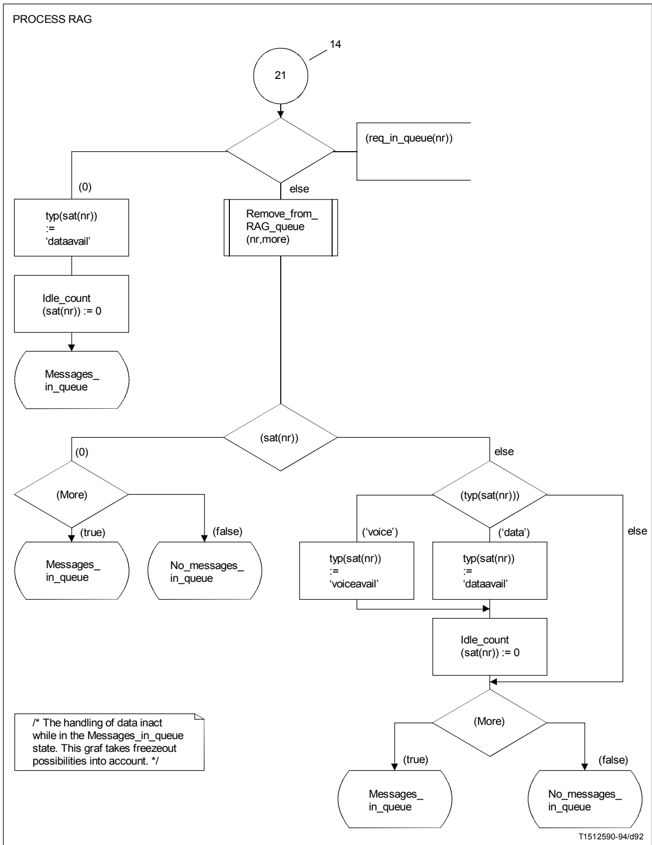
FIGURE A.23/G.763 (sheet 19 of 45)
