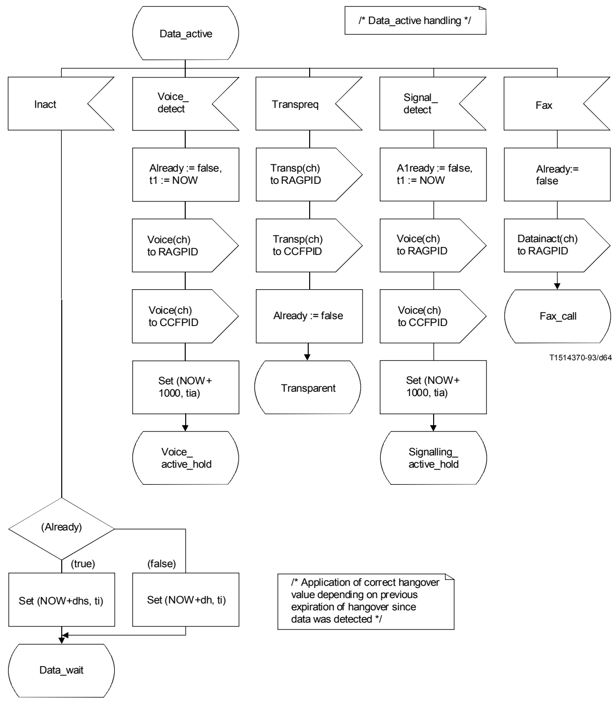
FIGURE A.19/G.763 (sheet 11 of 17)
