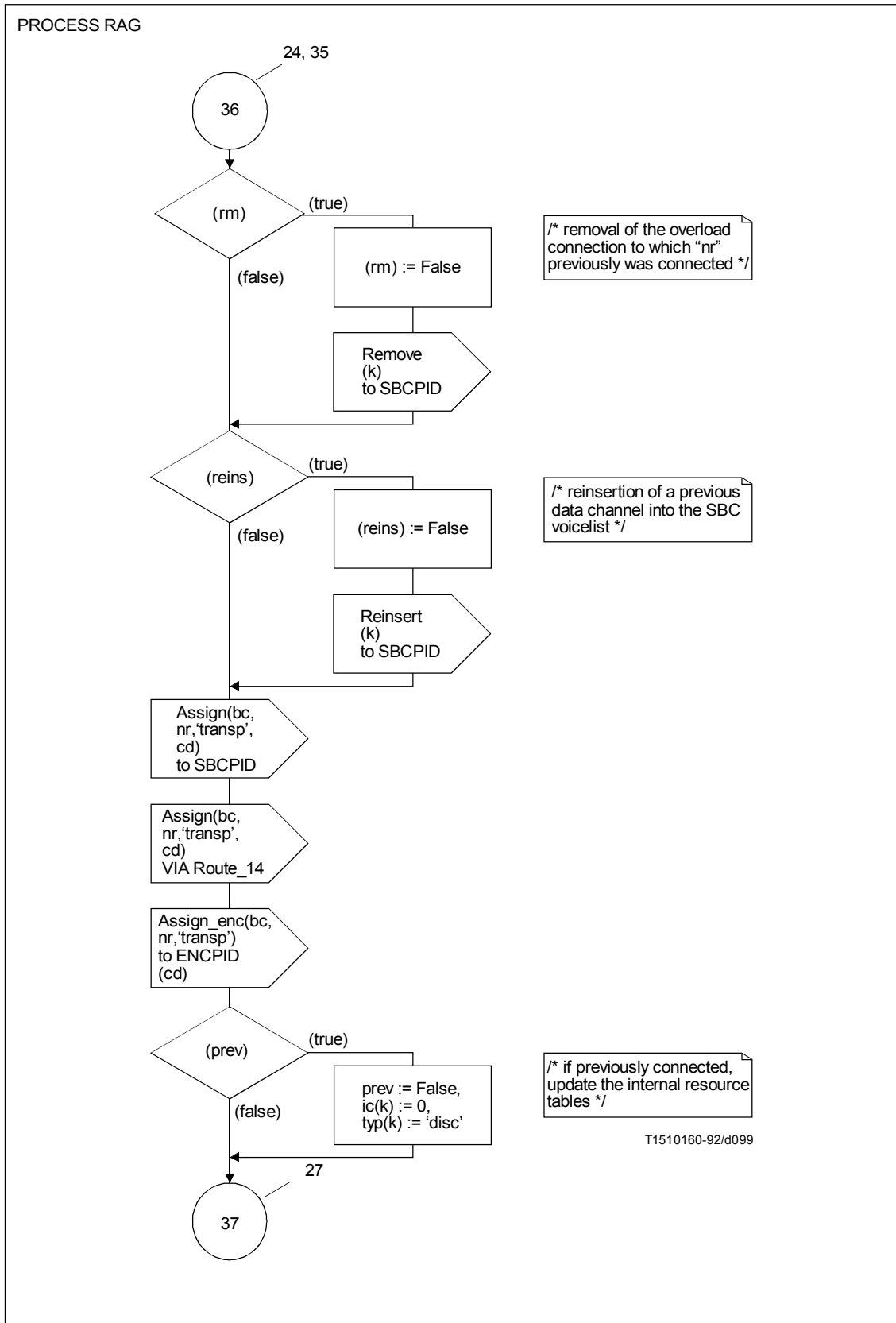
FIGURE A.23/G.763 (sheet 26 of 45)
