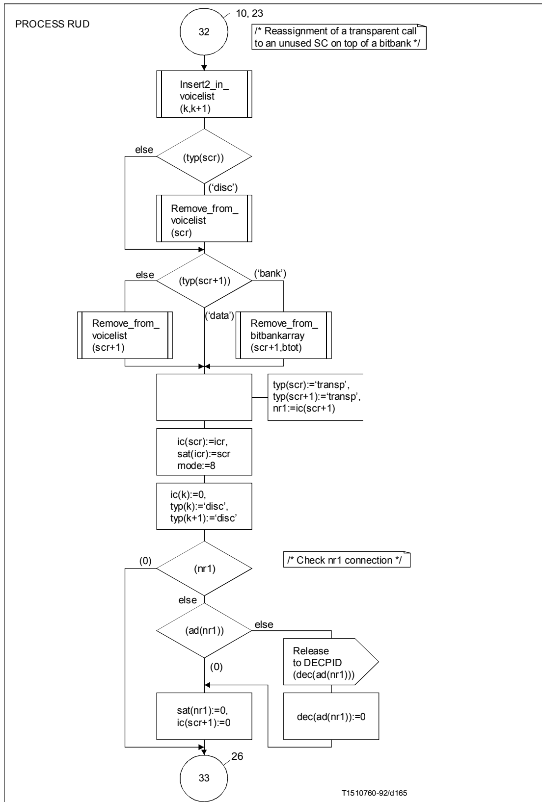
FIGURE A.35/G.763 (sheet 25 of 83)
