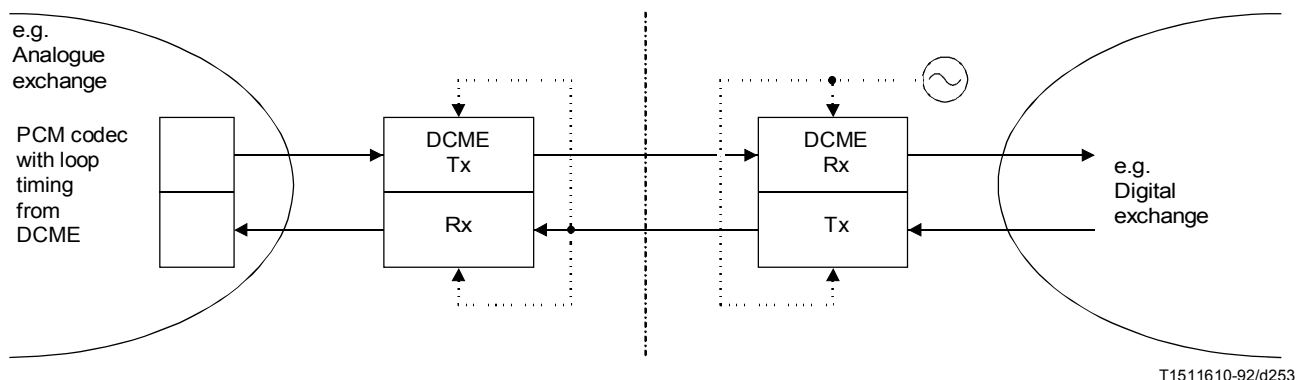
FIGURE B.8/G.763 DCME synchronous loop operation (between analogue and digital networks)
