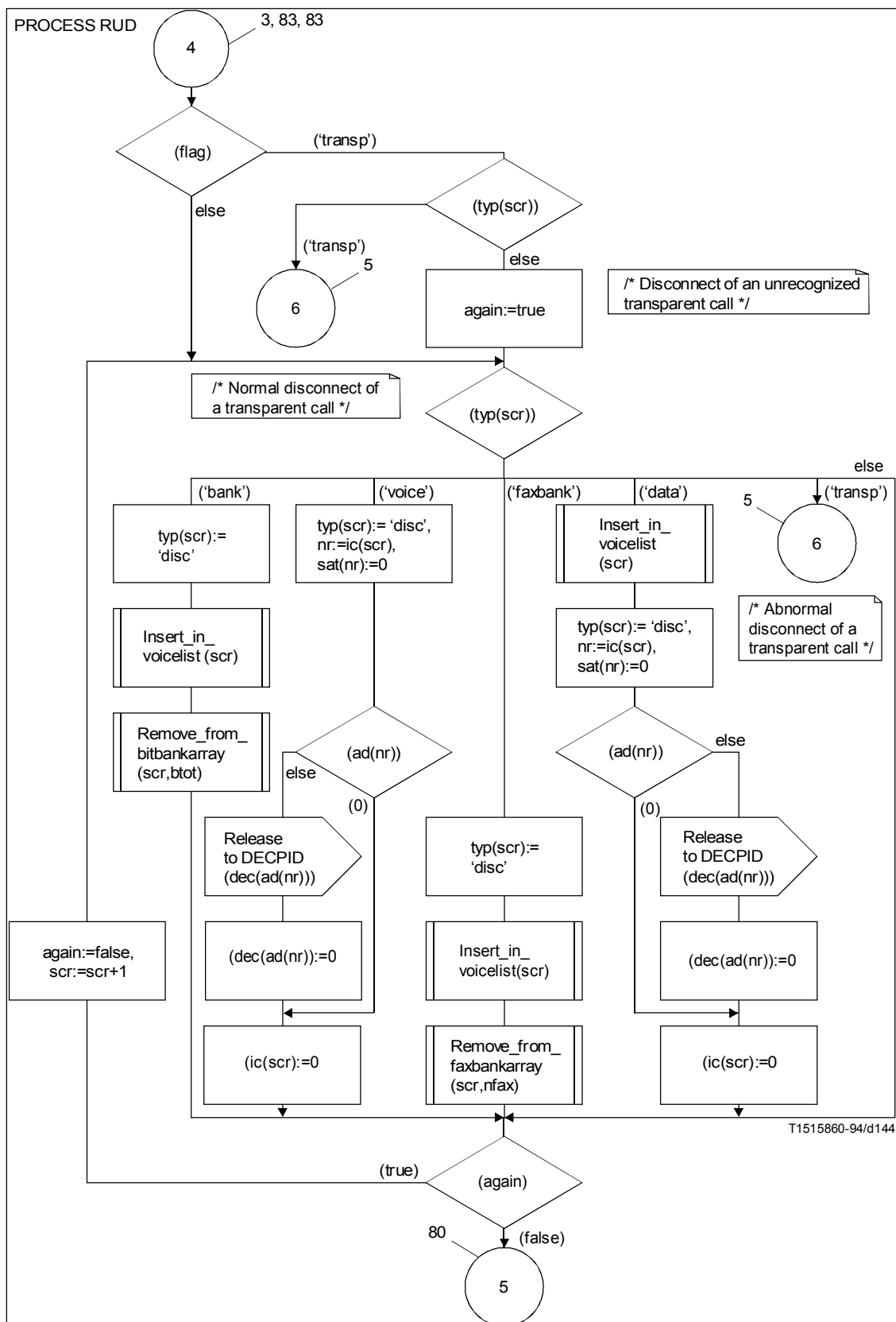
FIGURE A.35/G.763 (sheet 4 of 83)
