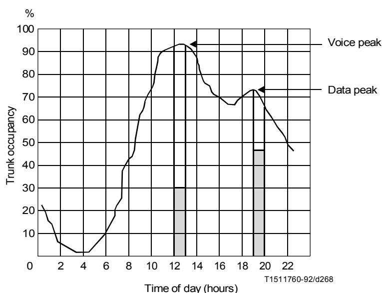
FIGURE 1 FDM profile
