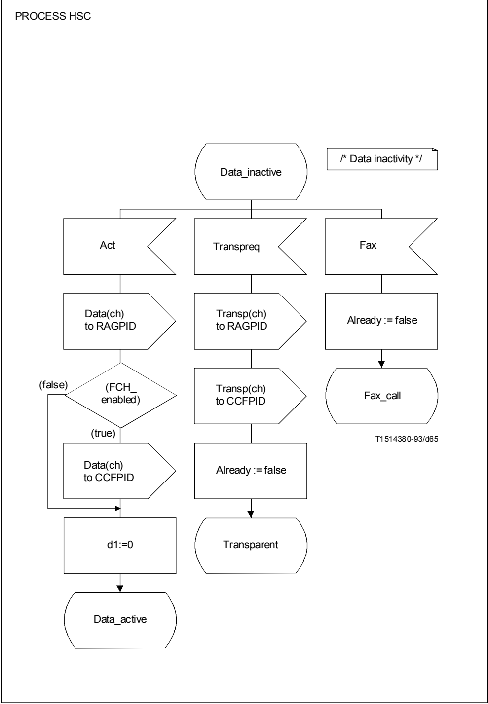
FIGURE A.19/G.763 (sheet 12 of 17) PROCESS HSC
