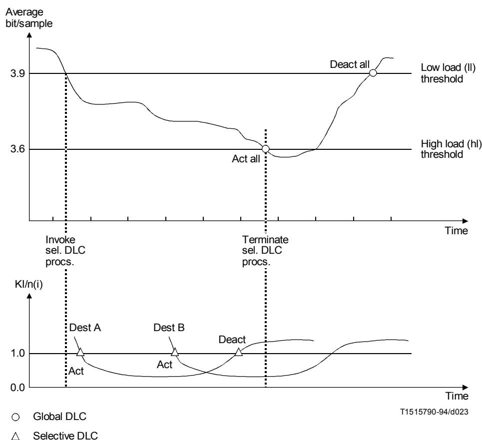
FIGURE 24/G.763 Example scenario of DLC activation/deactivation with only voice loading
