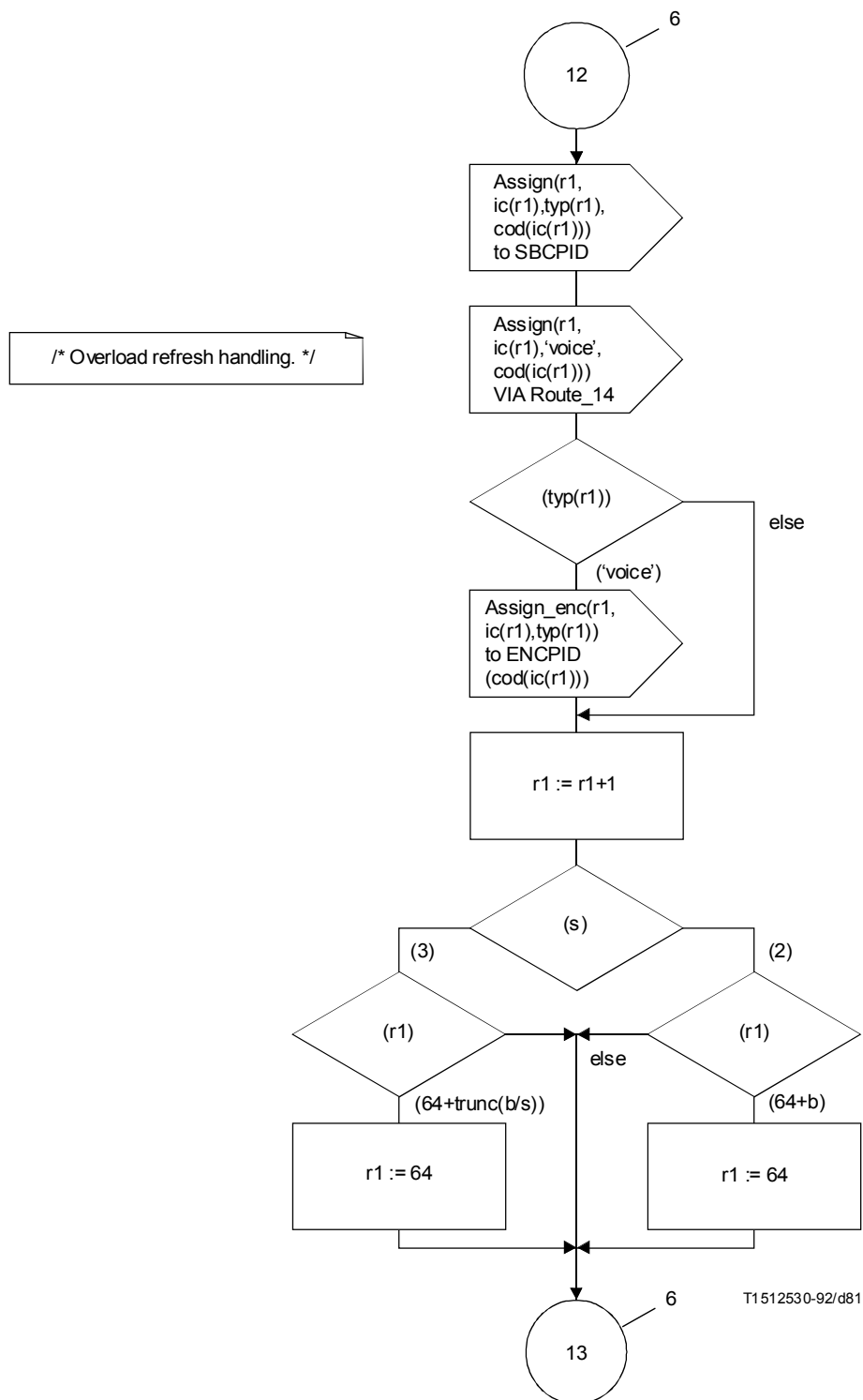
FIGURE A.23/G.763 (sheet 8 of 45)
