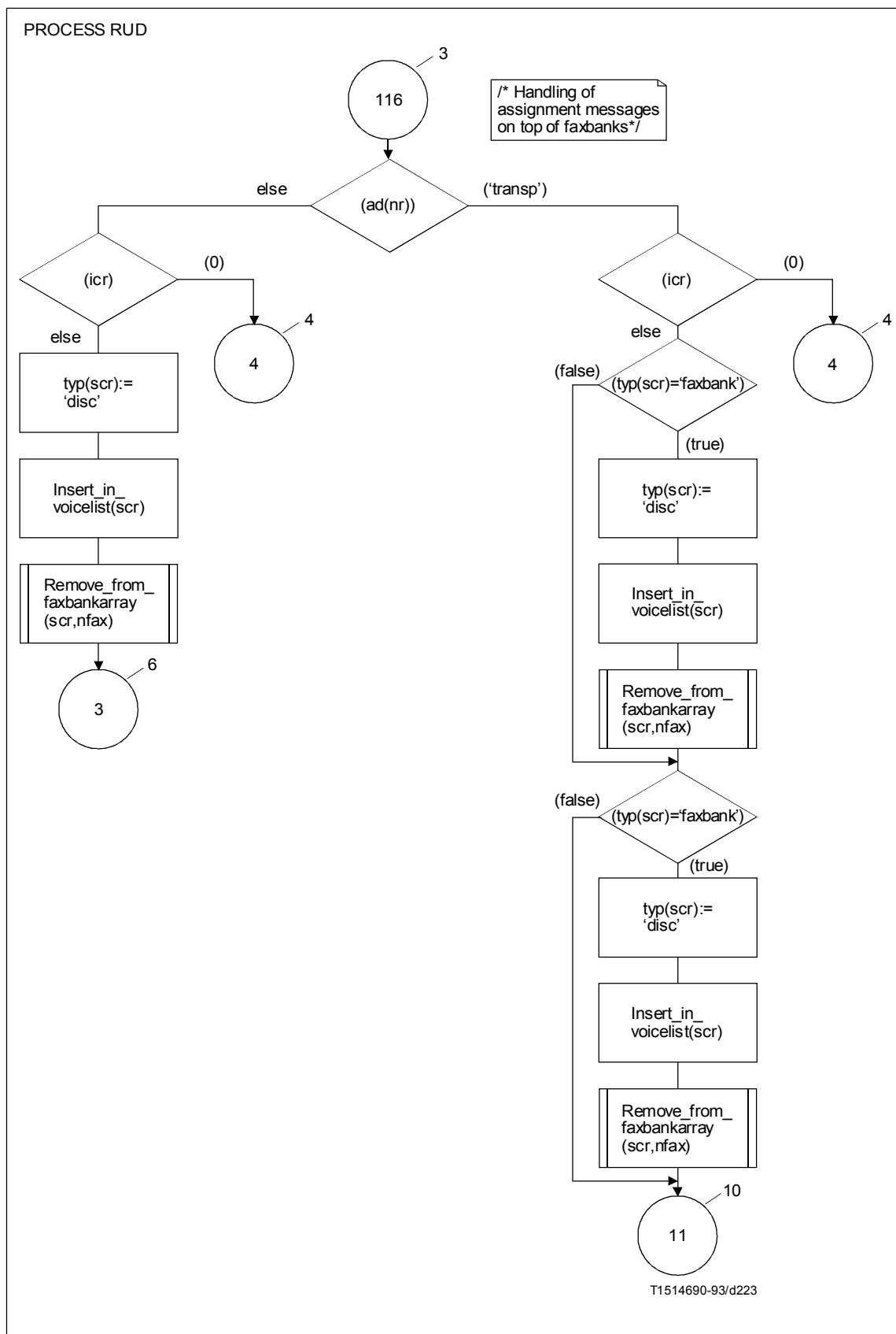
FIGURE A.35/G.763 (sheet 83 of 83)
