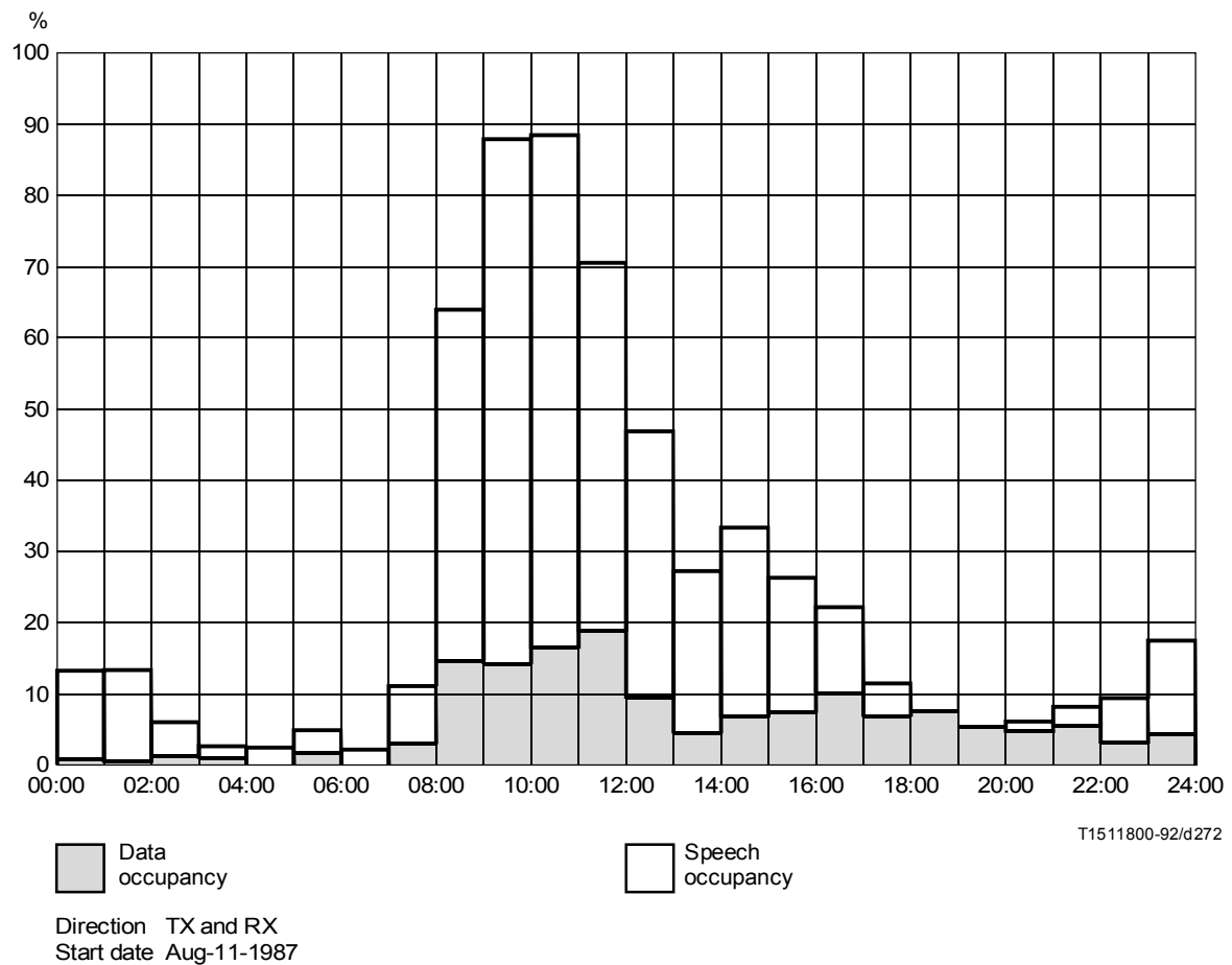
FIGURE 5 DCOA route profile for example 2
