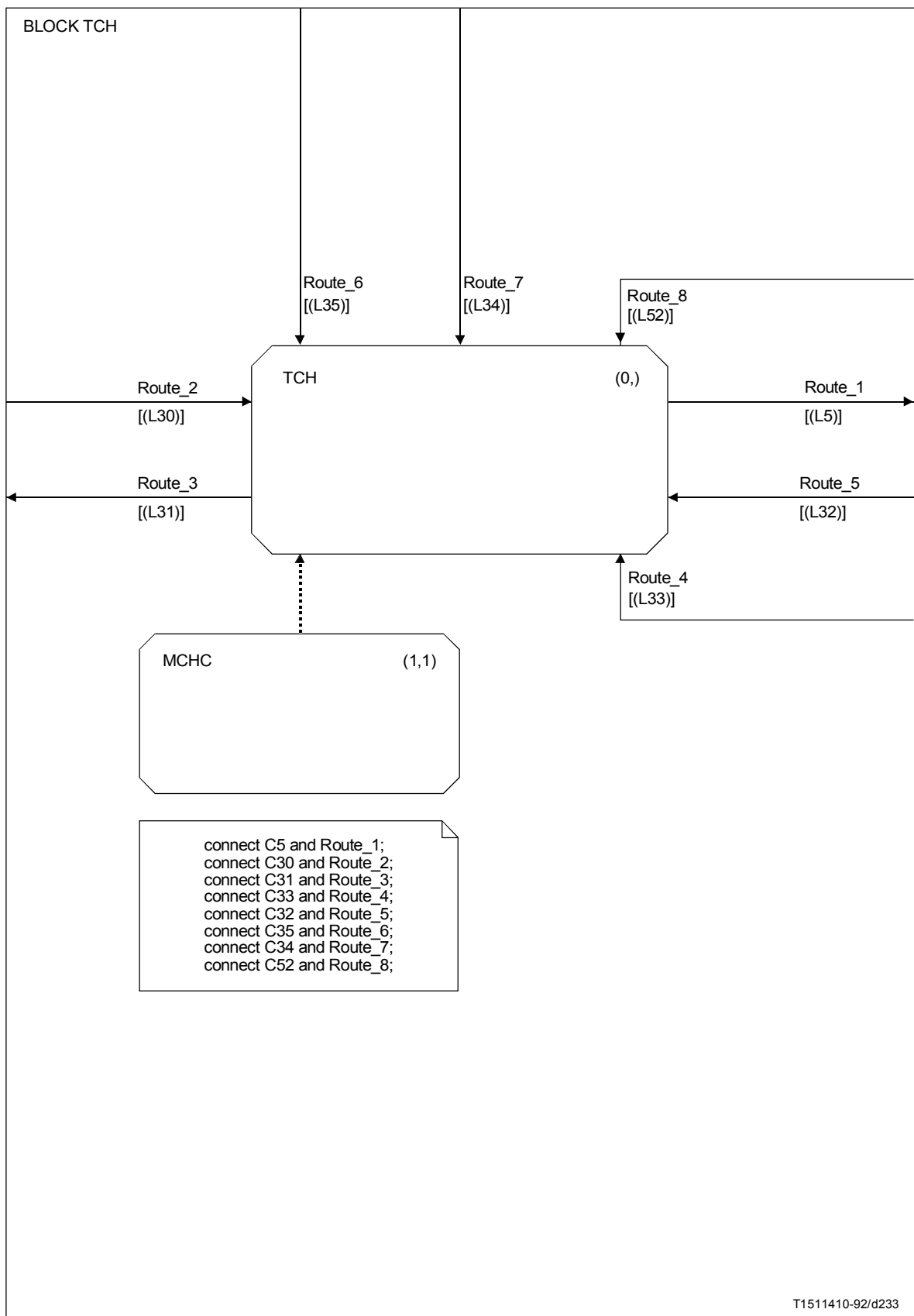
FIGURE A.41/G.763 BLOCH TCH
