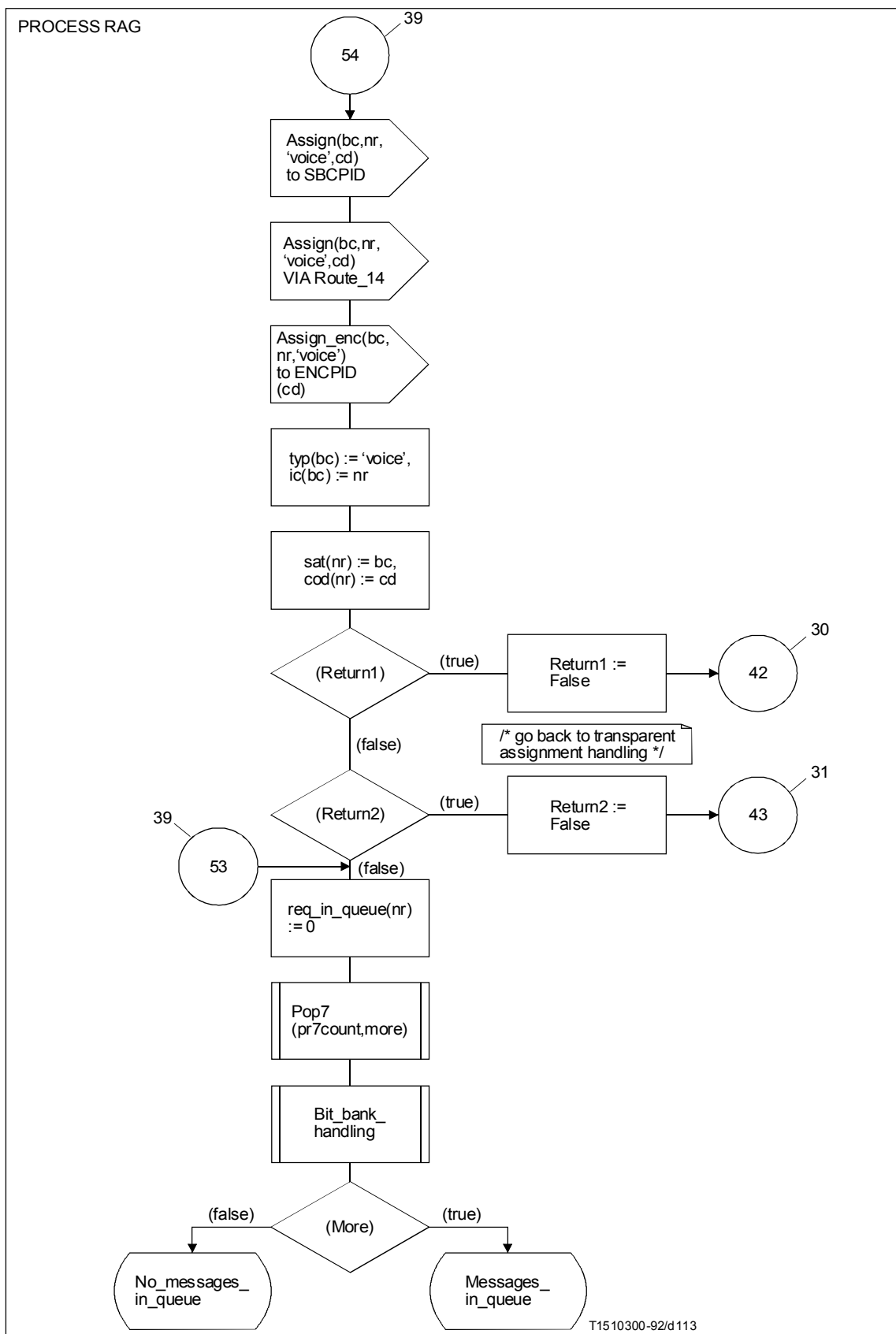
FIGURE A.23/G.763 (sheet 40 of 45)
