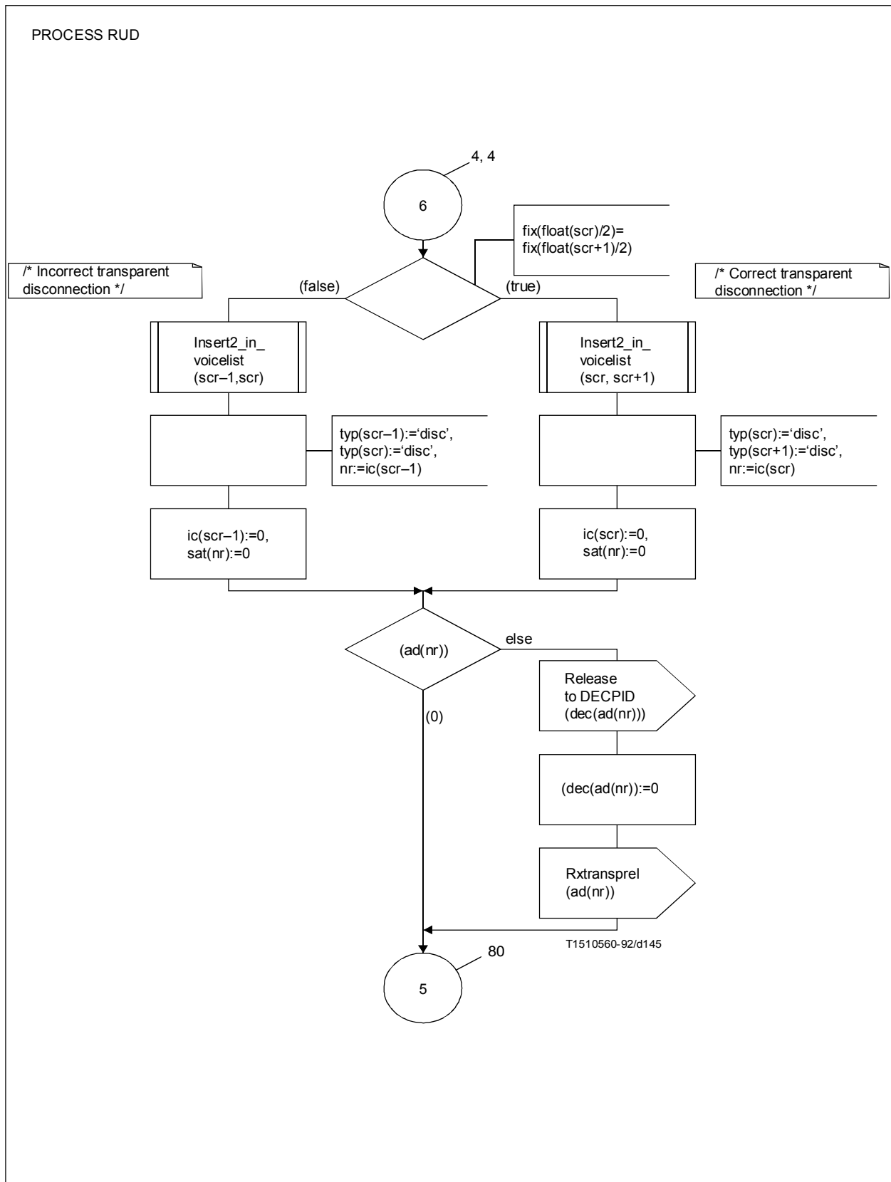
FIGURE A.35/G.763 (sheet 5 of 83)
