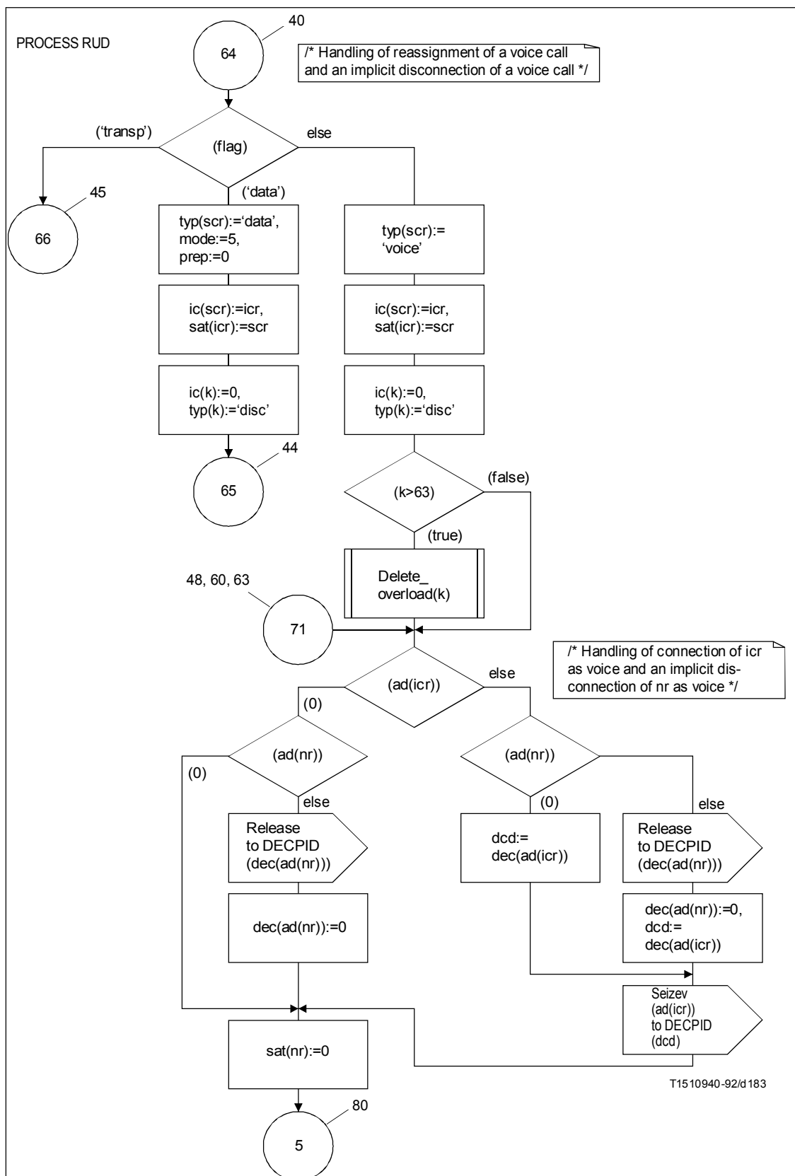
FIGURE A.35/G.763 (sheet 43 of 83)
