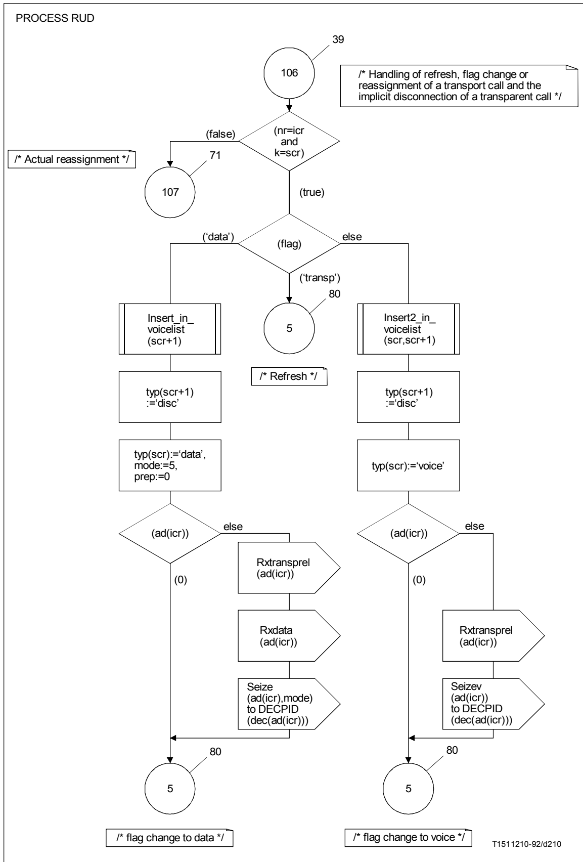
FIGURE A.35/G.763 (sheet 70 of 83)
