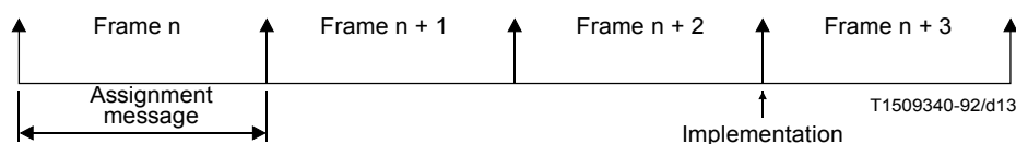
FIGURE 14/G.763 Implementation timing
