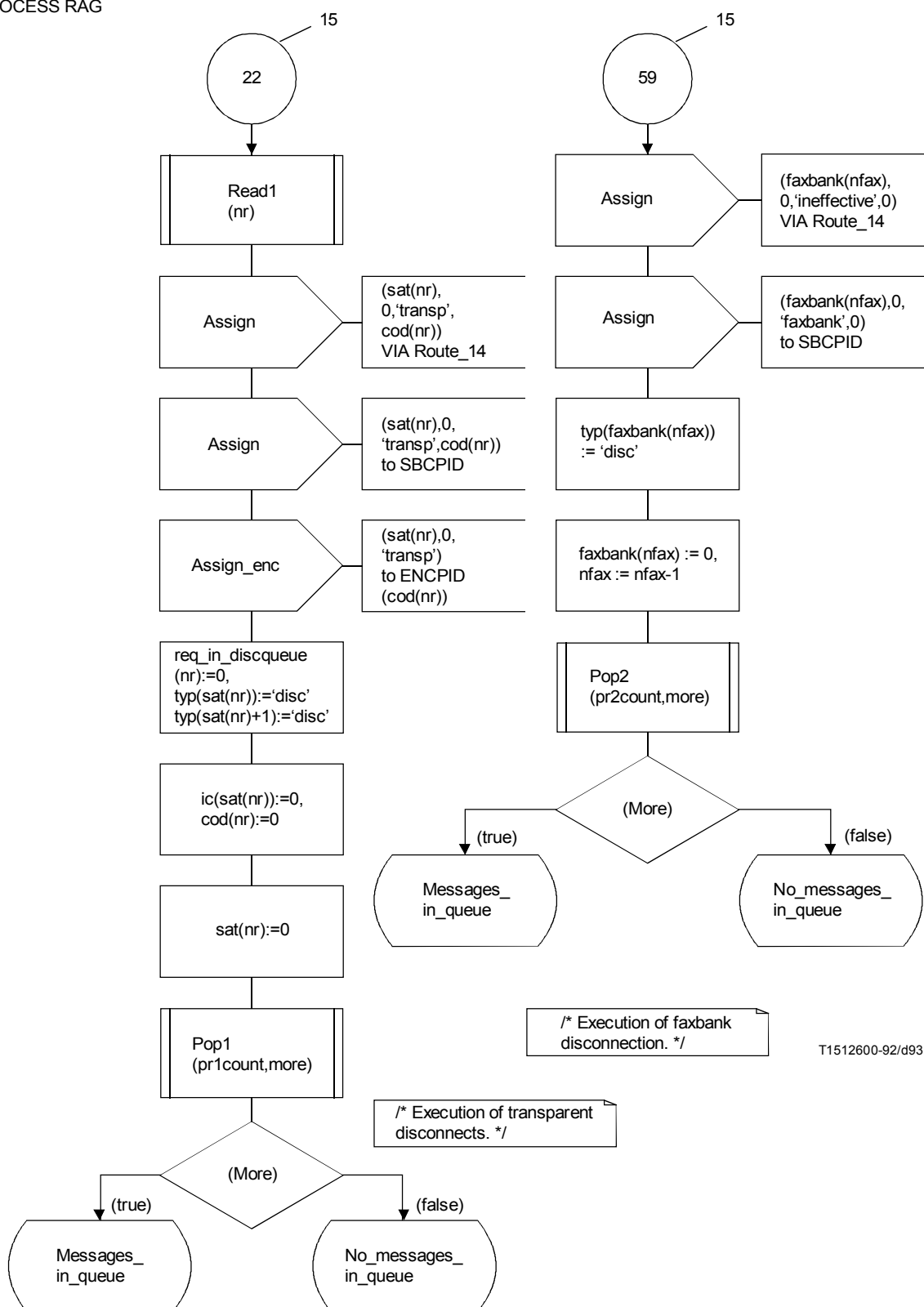
FIGURE A.23/G.763 (sheet 20 of 45)
