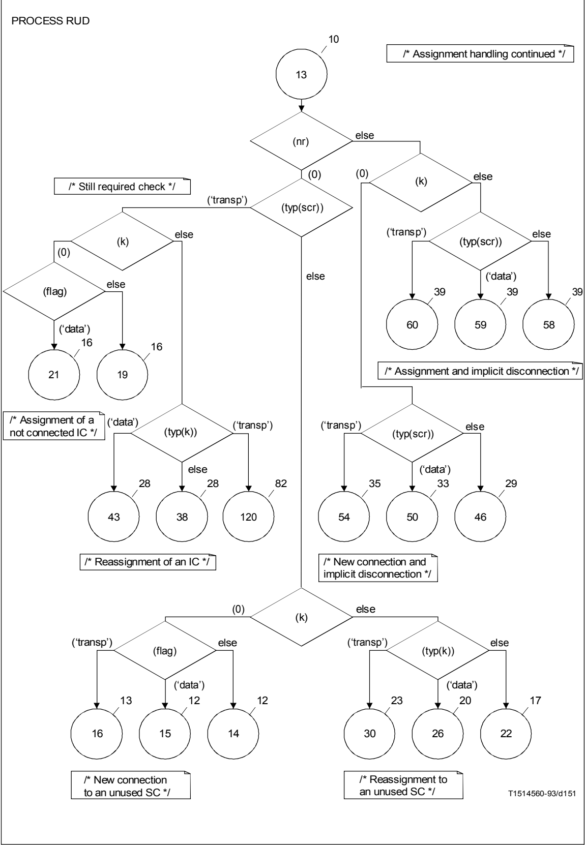
FIGURE A.35/G.763 (sheet 11 of 83)
