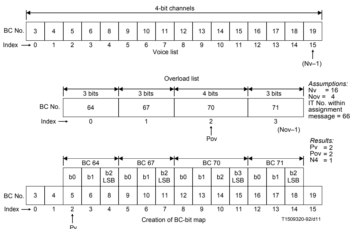
FIGURE 11/G.763 Example of 4/3 bit overload channel creation procedure
