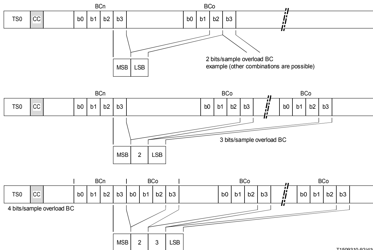
FIGURE 10/G.763 An example of 32, 24 and 16 kbit/s overload bearer channels (4, 3 and 2 bits/sample)
