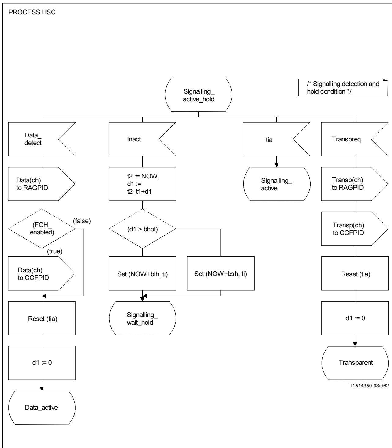
FIGURE A.19/G.763 (sheet 9 of 17)
