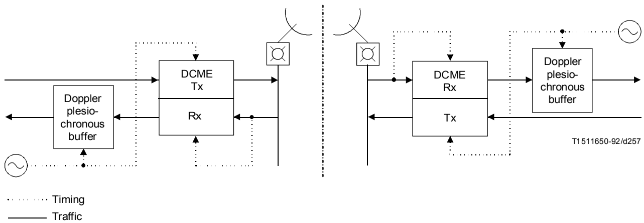
FIGURE B.12/G.763 DCME synchronous (independent) operation (between two plesiochronous networks)
