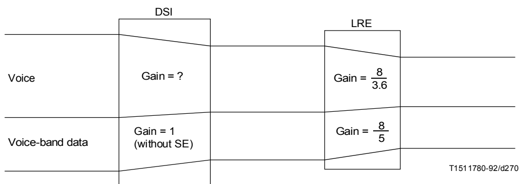
FIGURE 3 DCME gain
