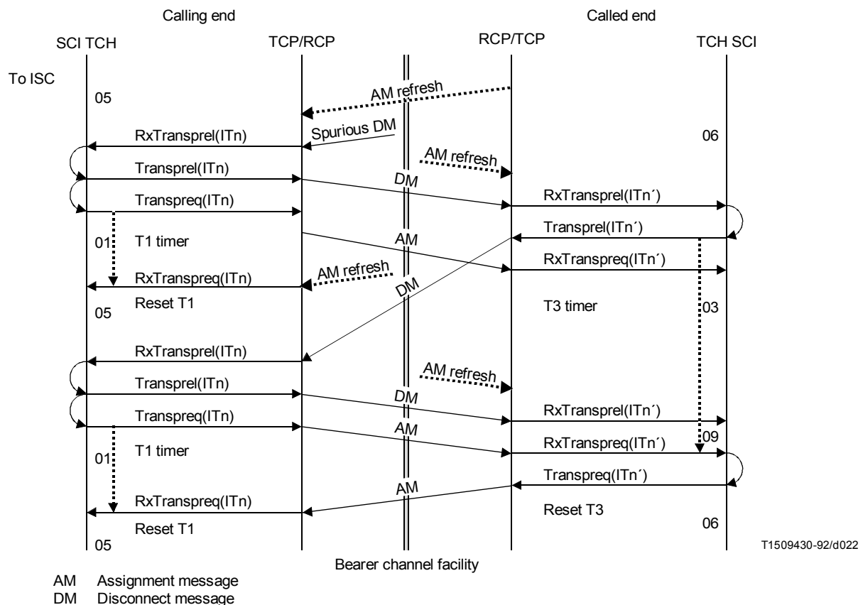
FIGURE 23/G.763 Sequence chart for 64 kbit/s circuit re-establishment after a spurious disconnect into calling end
