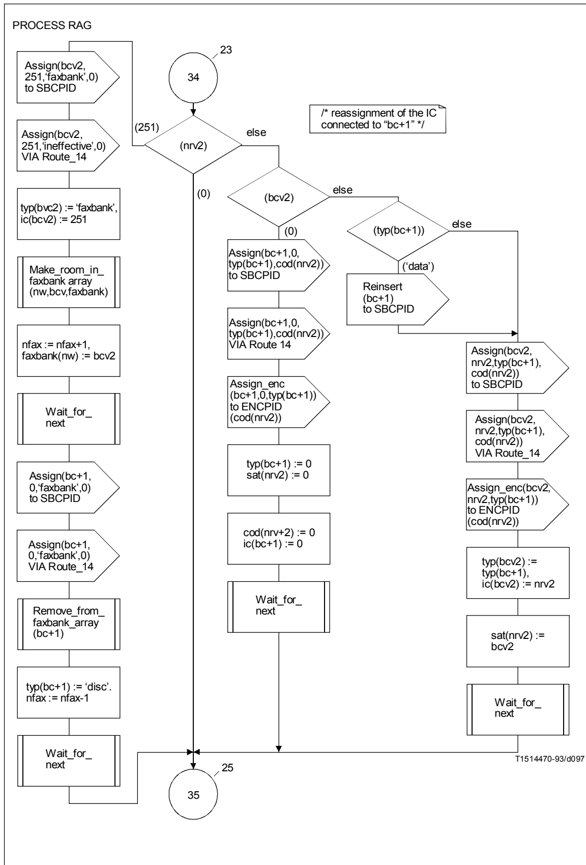
FIGURE A.23/G.763 (sheet 24 of 45)
