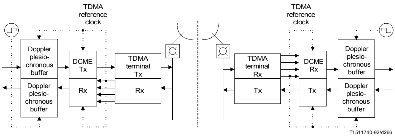
FIGURE B.21/G.763 DCME synchronous operation (between two plesiochronous networks)
