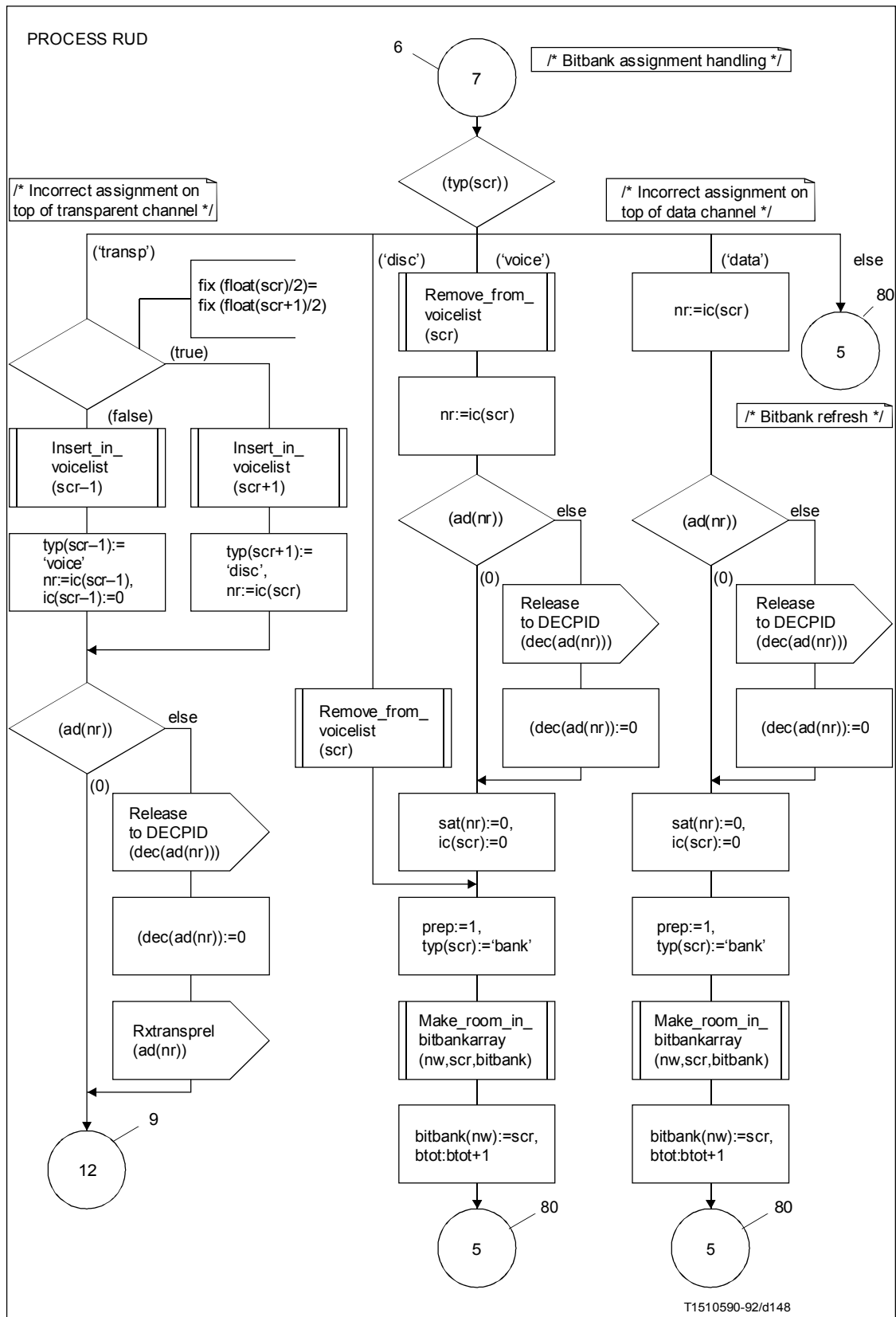
FIGURE A.35/G.763 (sheet 8 of 83)
