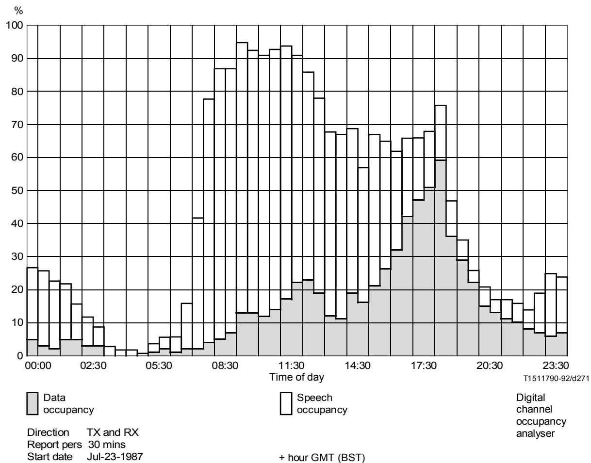
FIGURE 4 DCOA route profile for example 1
