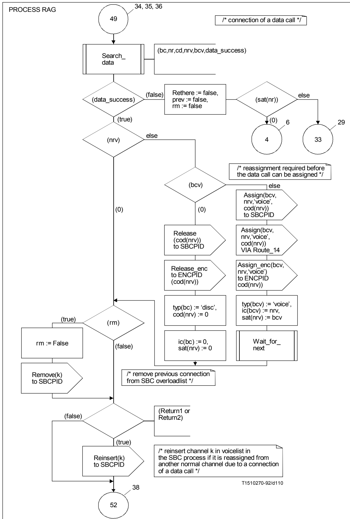
FIGURE A.23/G.763 (sheet 37 of 45)
