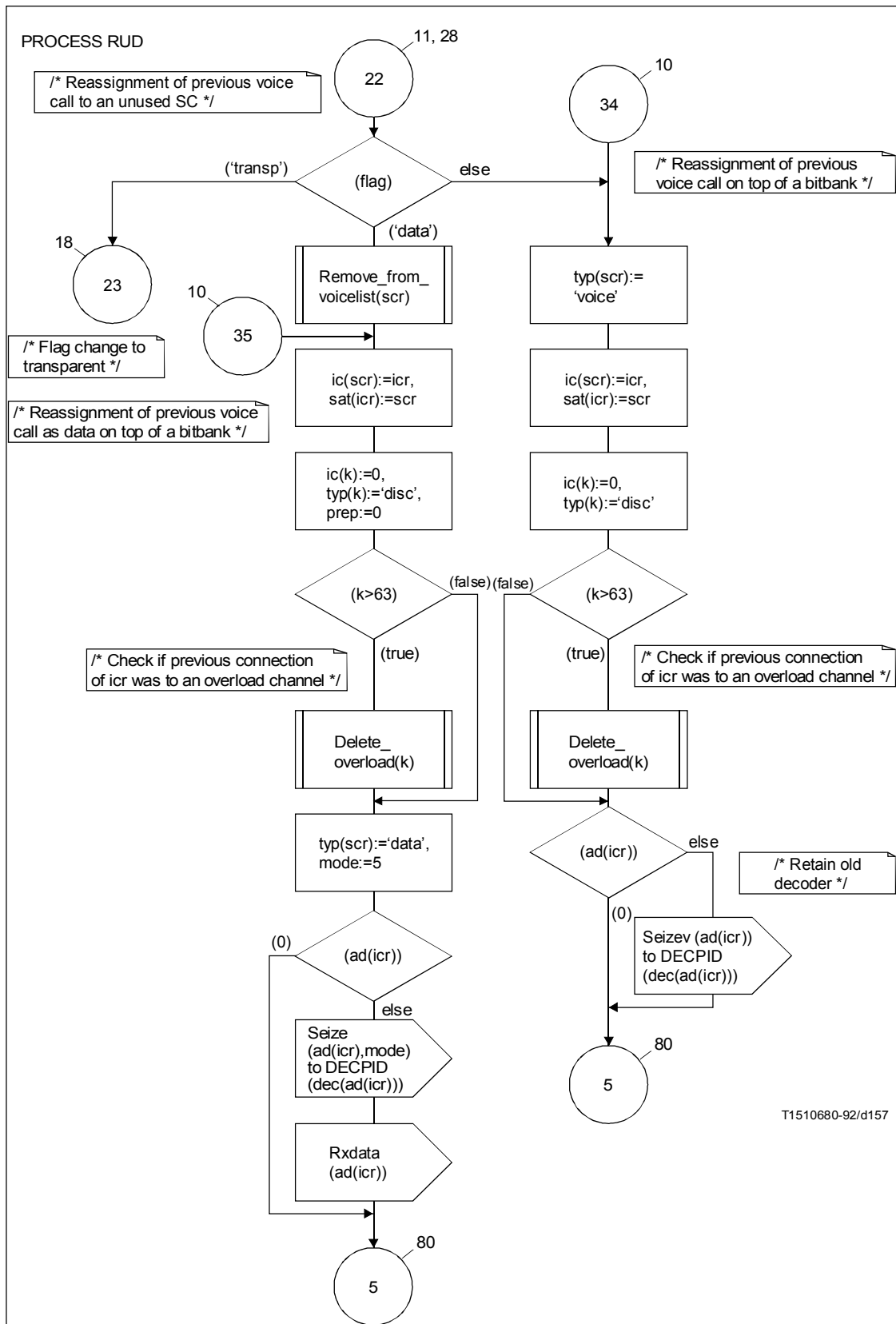
FIGURE A.35/G.763 (sheet 17 of 83)
