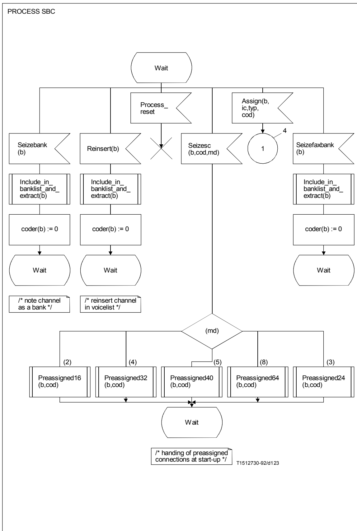
FIGURE A.26/G.763 (sheet 3 of 6)
