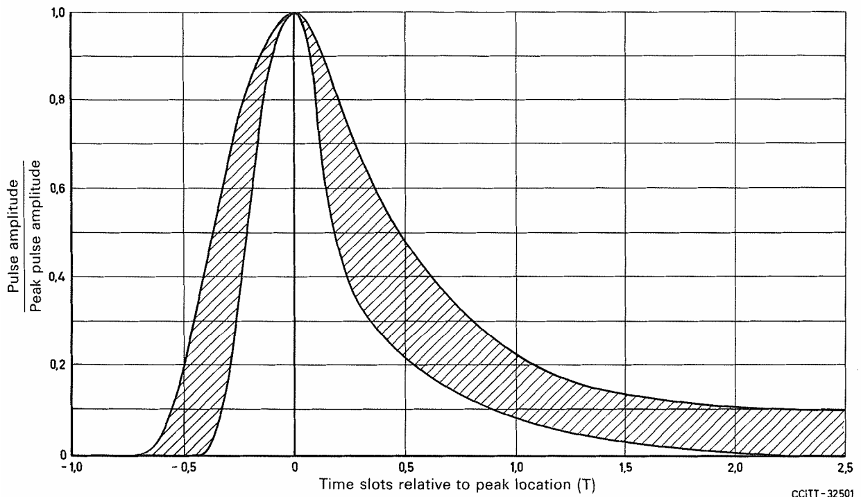
FIGURE 11/G.703
