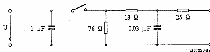
FIGURE B-1/G.703
