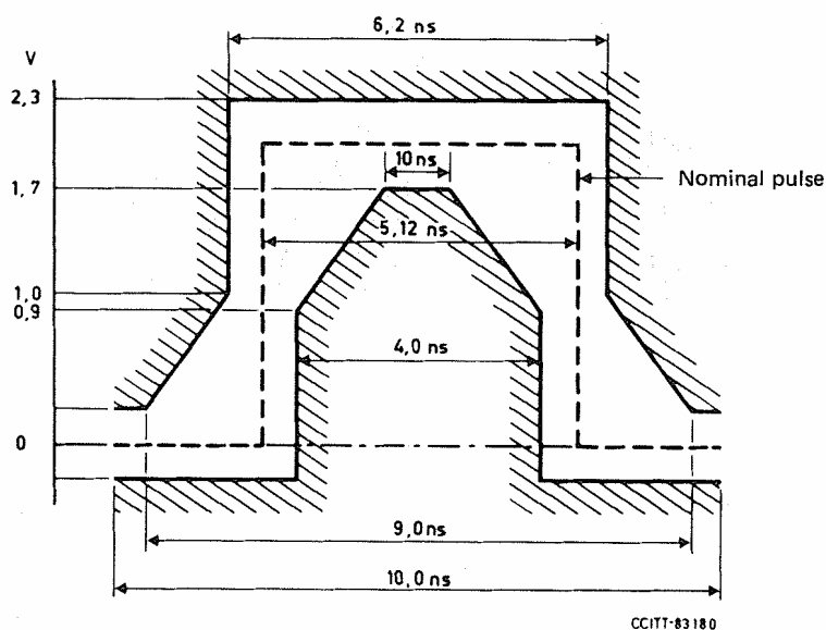
FIGURE 22/G.703
