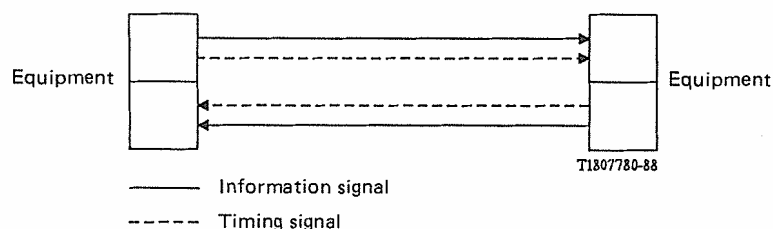
FIGURE 1/G.703
