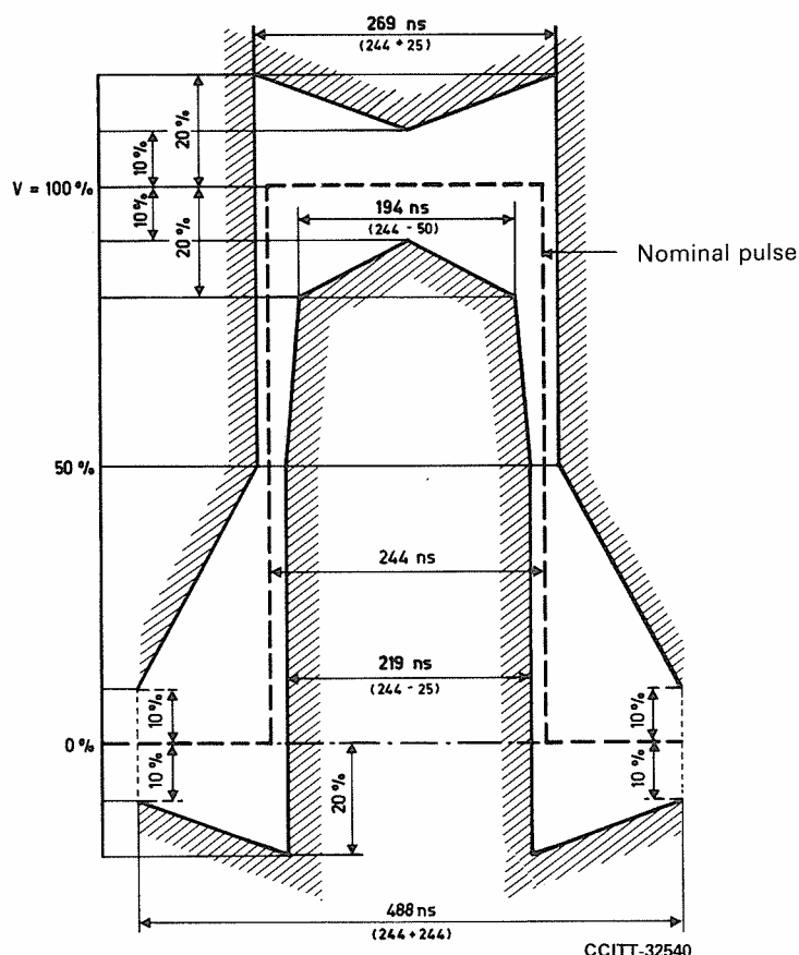
FIGURE 15/G.703
