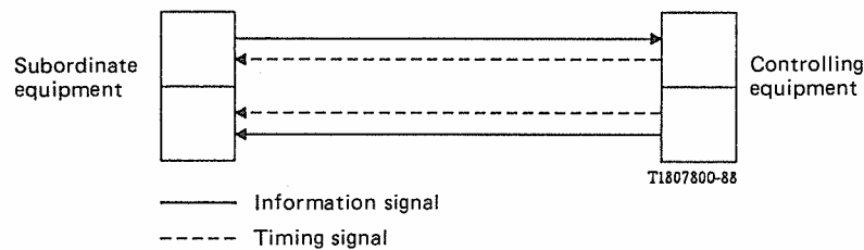
FIGURE 3/G.703
