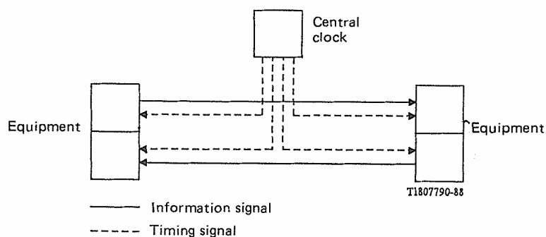
FIGURE 2/G.703
