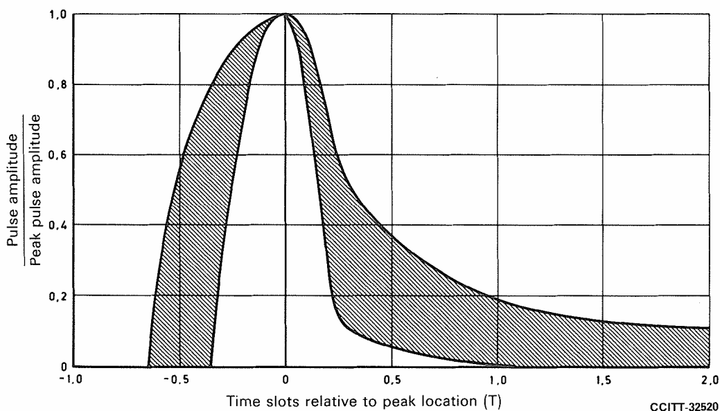
FIGURE 13/G.703
