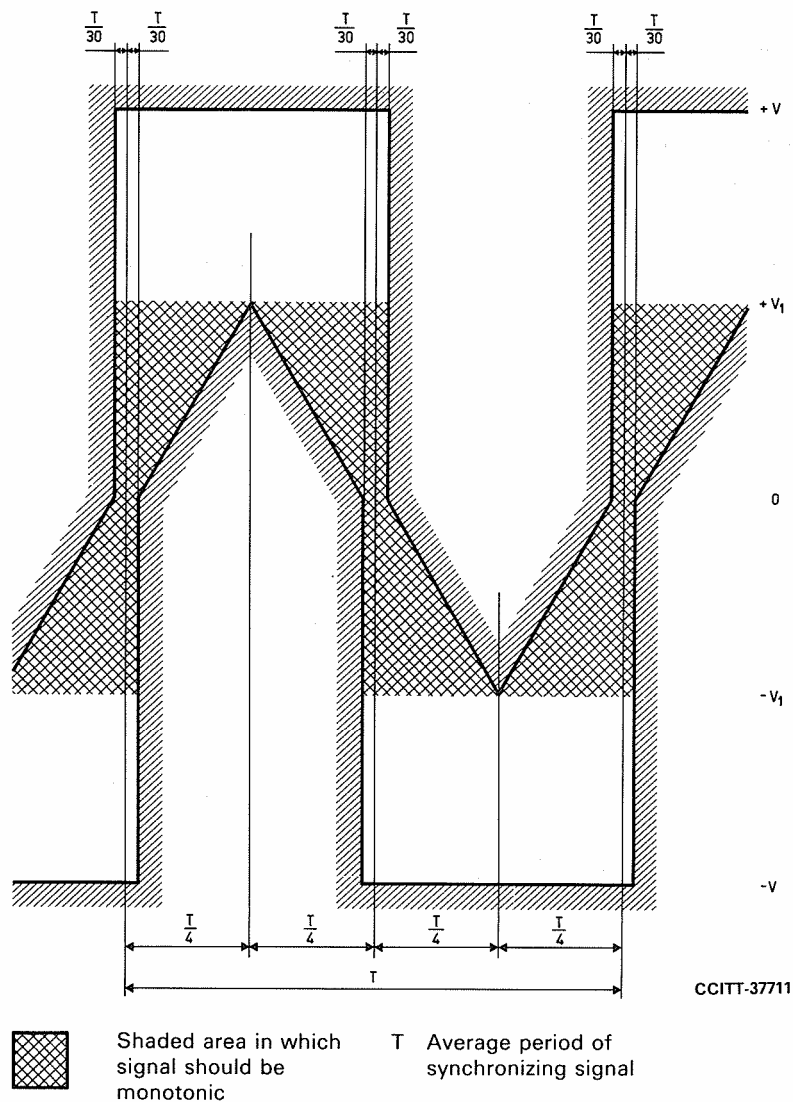
FIGURE 21/G.703
