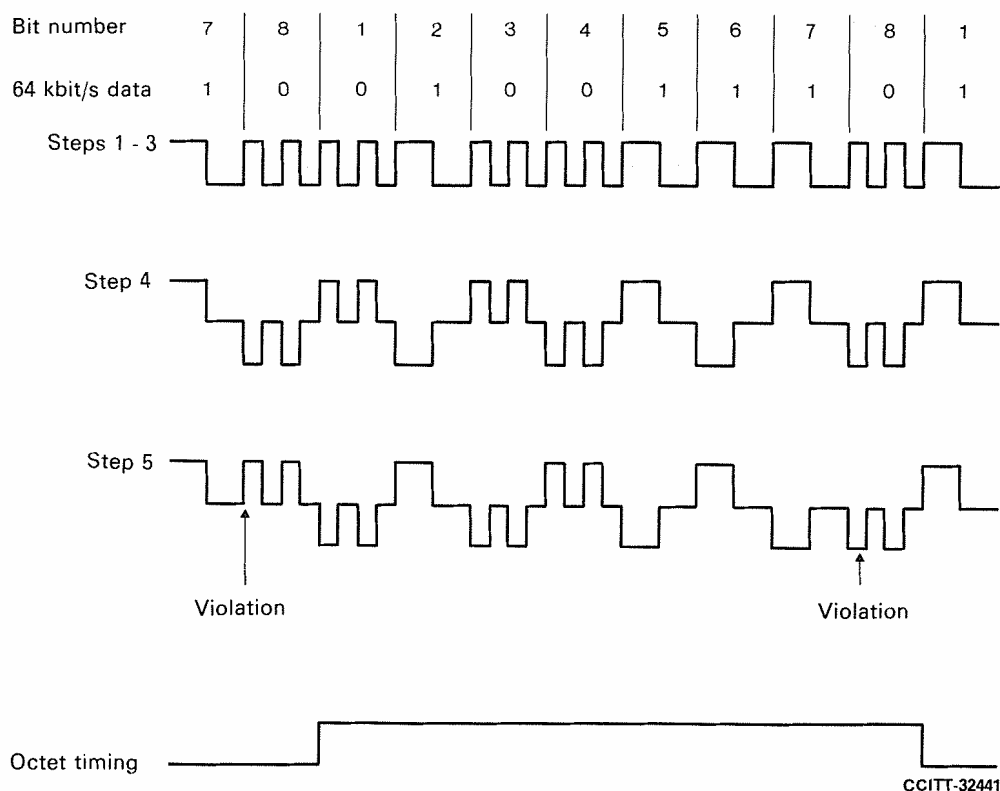
FIGURE 4/G.703
