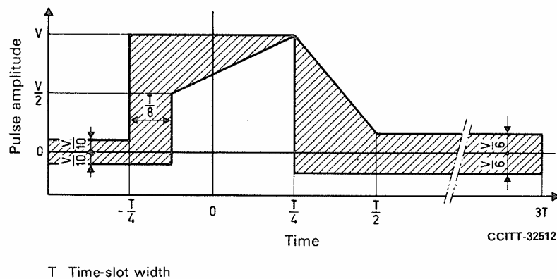
FIGURE 12/G.703
