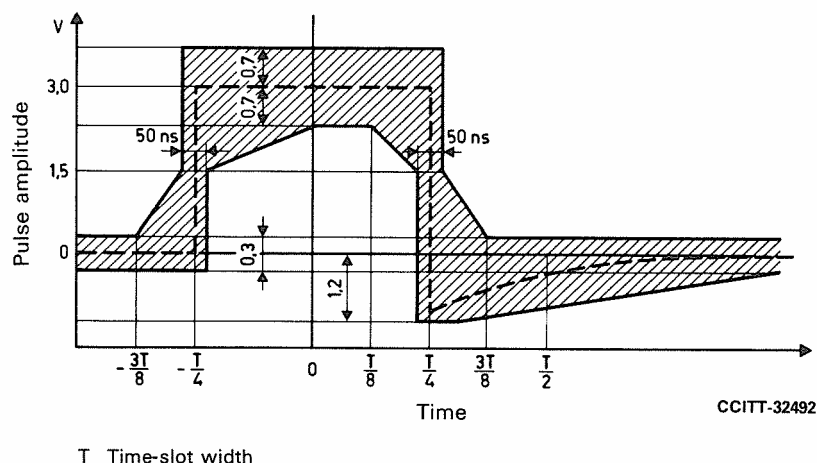
FIGURE 10/G.703
