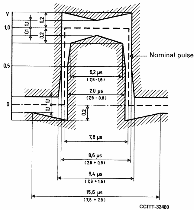
FIGURE 9/G.703
