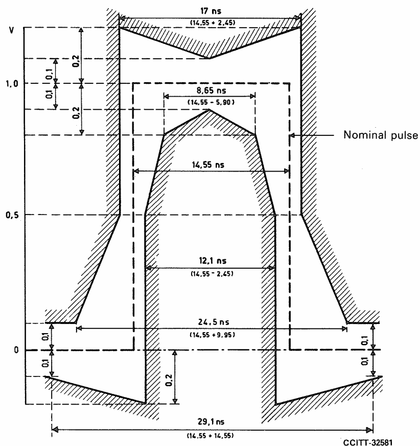
FIGURE 17/G.703
