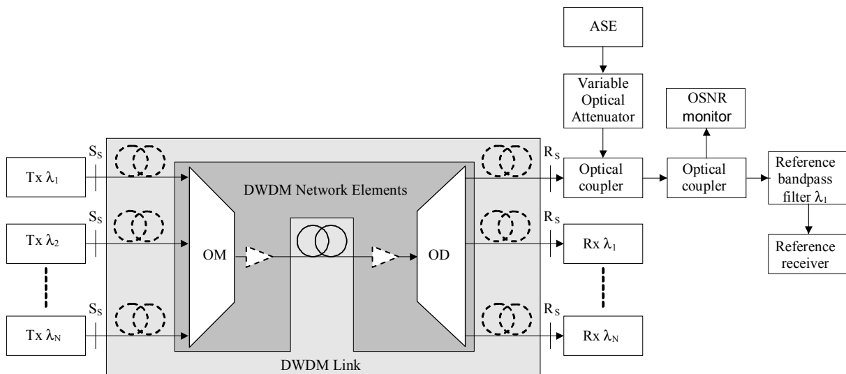
Figure I.3 – Configuration for measurement 3 (at R_S )
