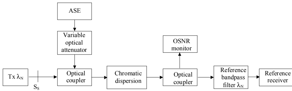
Figure I.2 – Configuration for measurement 2 (at S_S )
