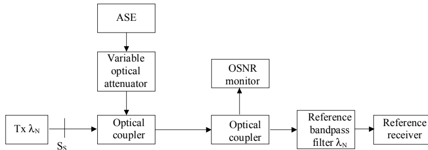
Figure I.1 – Configuration for measurement 1 (at S_S )
