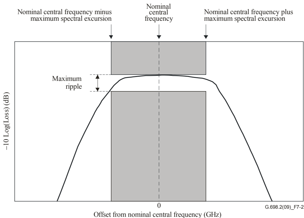
Figure 7-2 – Illustration of maximum ripple
