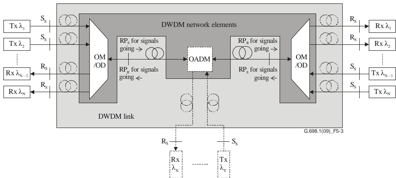
Figure 5-3 – Linear "black link" approach for bidirectional applications
