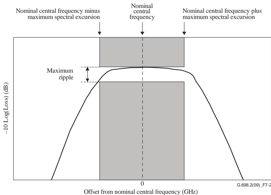
Figure 7-2 – Illustration of a maximum ripple
