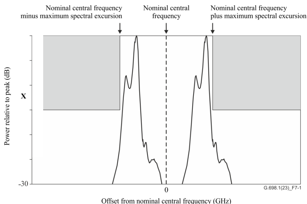
Figure 7-1 – Illustration of the maximum spectral excursion
