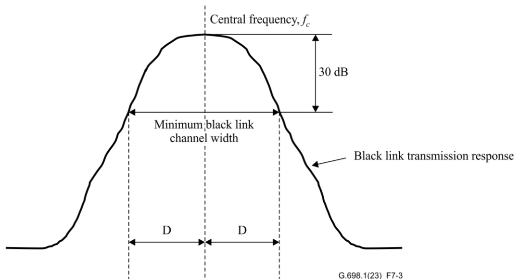
Figure 7-3 – Black link channel width
