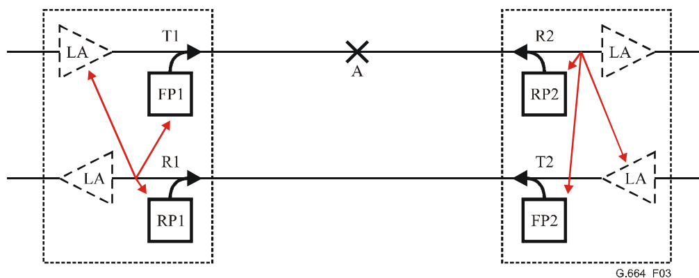
Figure 3 – Possible actions in the case of loss of continuity within a cable
