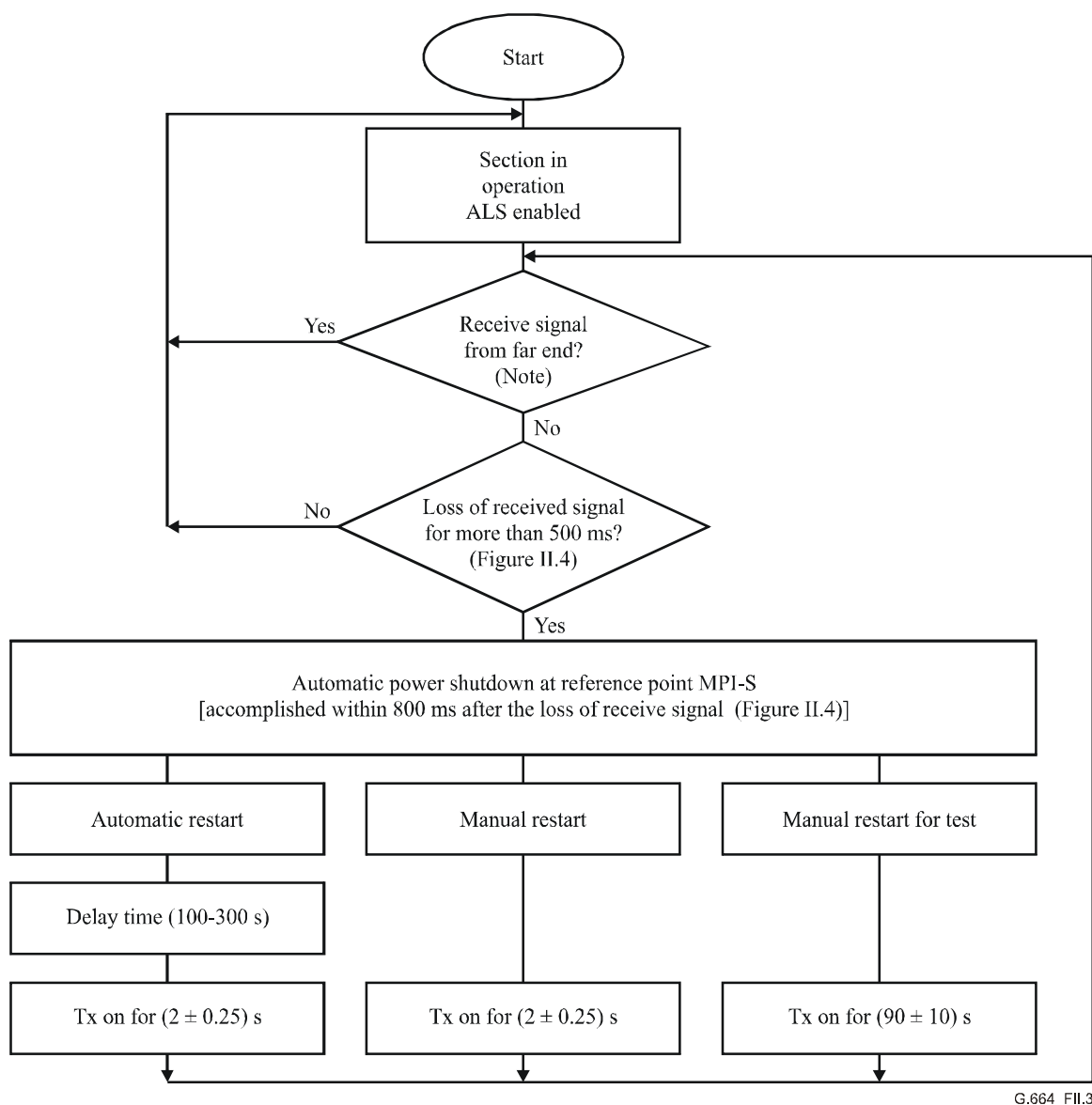
Figure II.3 – Automatic laser shut-down and restart concept including optional test procedure
