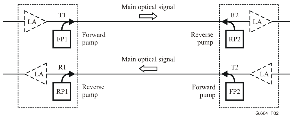
Figure 2 – Configuration with forward and reverse pump lasers in a section within multi-span transmission system employing distributed Raman amplification
