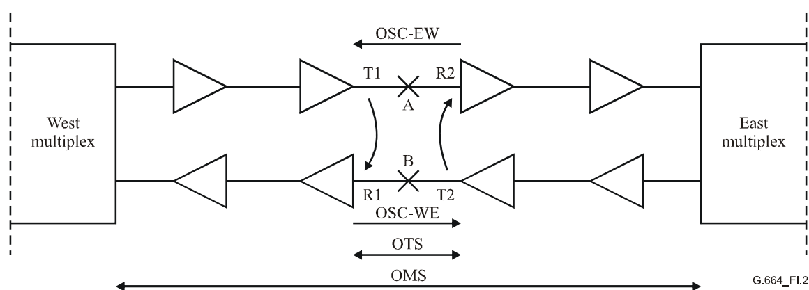
Figure I.2/G.664 – Description of APR capability in the case of loss of continuity within a cable in a configuration with counter-propagating OSC
