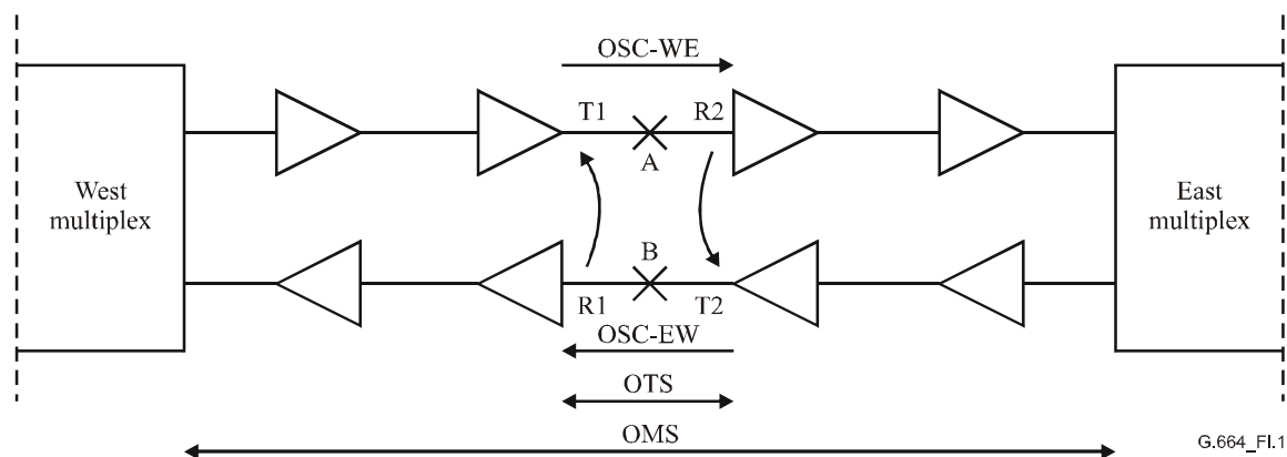
Figure I.1/G.664 – Description of APR capability in the case of loss of continuity within a cable in a configuration with co-propagating OSC
