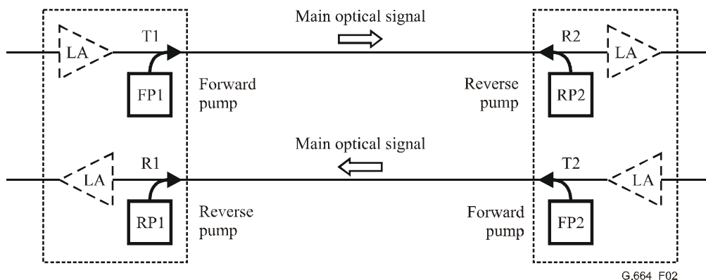
Figure 2/G.664 – Configuration with forward and reverse pump lasers in a section within multi-span transmission system employing distributed Raman amplification
