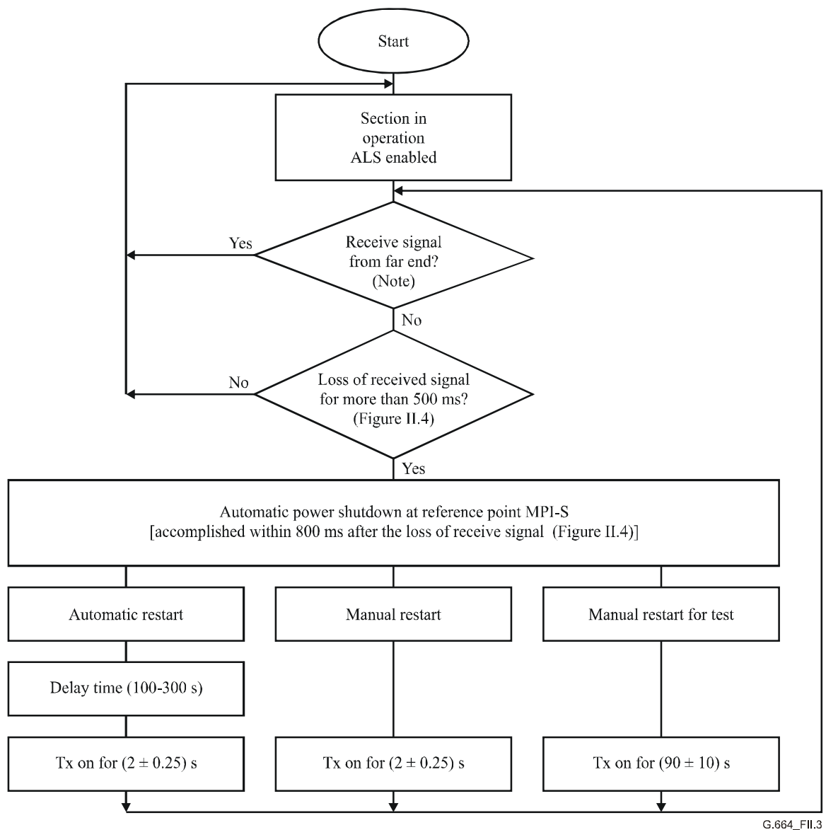
Figure II.3/G.664 – Automatic laser shutdown and restart concept including optional test procedure
