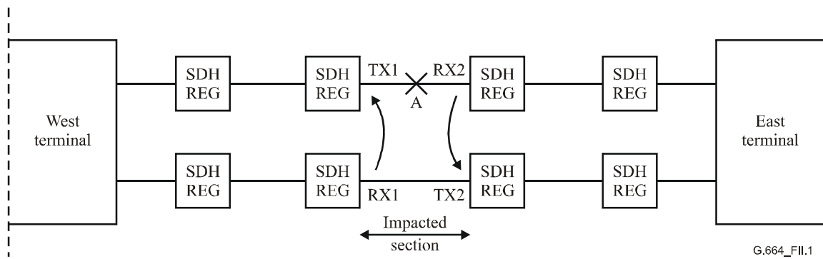
Figure II.1/G.664 – Clarification of ALS operation in the case of loss of continuity within a cable in a chain of SDH regenerators
