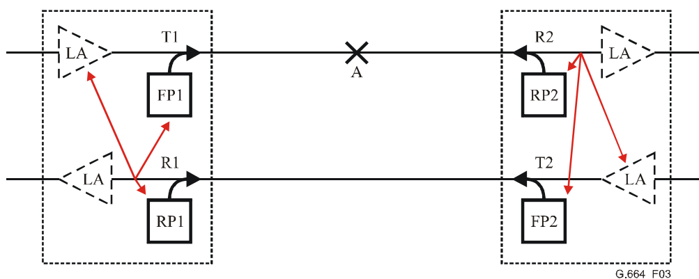
Figure 3/G.664 – Possible actions in the case of loss of continuity within a cable
