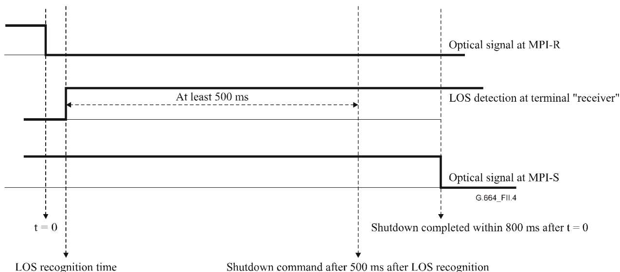
Figure II.4/G.664 – Clarification of shutdown timing requirements
