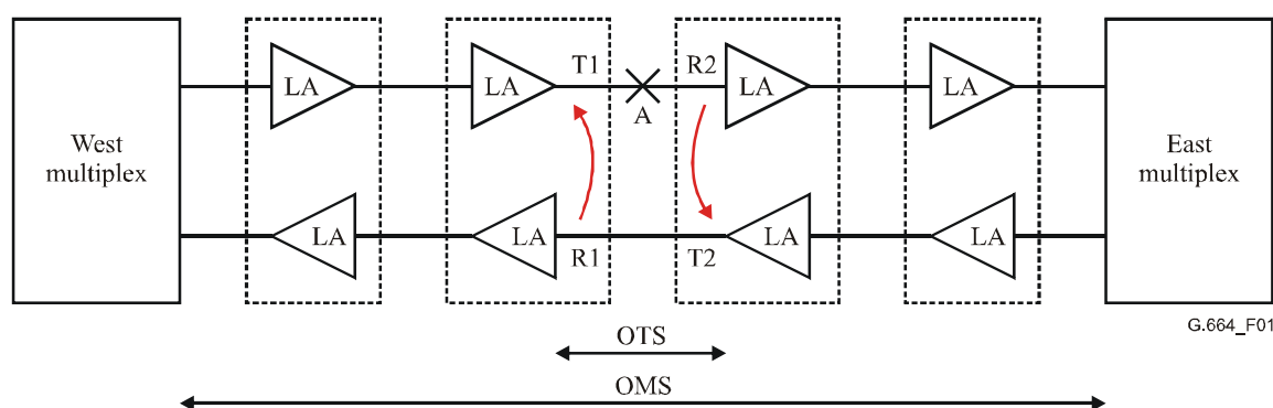
Figure 1/G.664 – Description of APR capability in the case of loss of continuity of a cable
