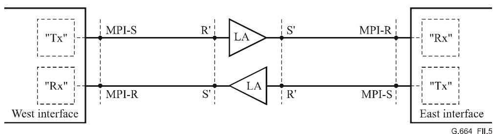
Figure II.5/G.664 – Reference configuration for description of ALS capability in the case that line amplifiers are present
