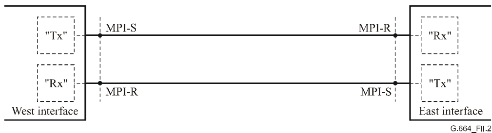
Figure II.2/G.664 – Reference configuration for description of ALS capability
