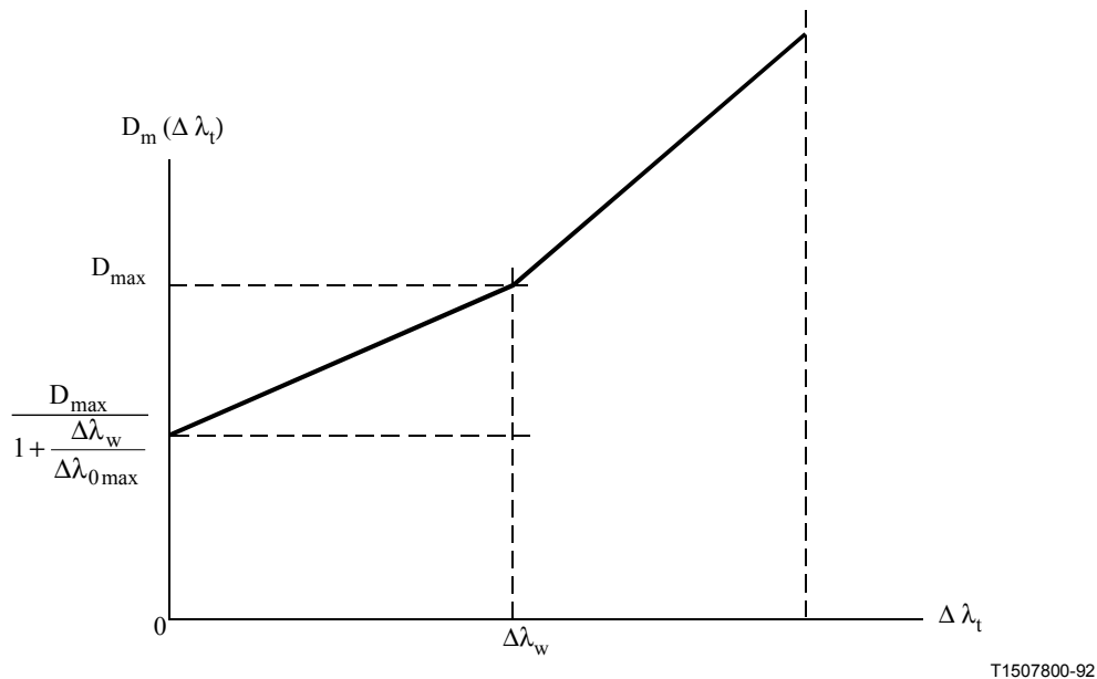
Figure 1/G.653 – Maximum absolute value of the dispersion coefficient
