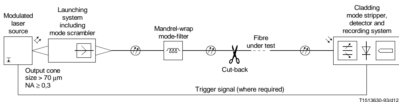
FIGURE B.11/G.651 Typical arrangement of test set-up
