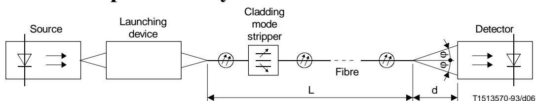
FIGURE B.5/G.651
