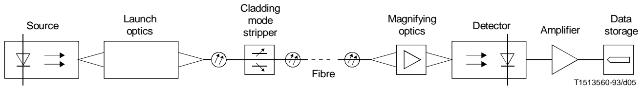
FIGURE B.4/G.651
