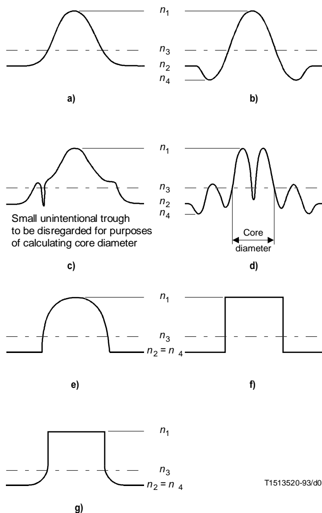
FIGURE A.1/G.651 Some refractive index profiles
