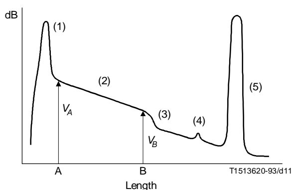
FIGURE B.10/G.651
