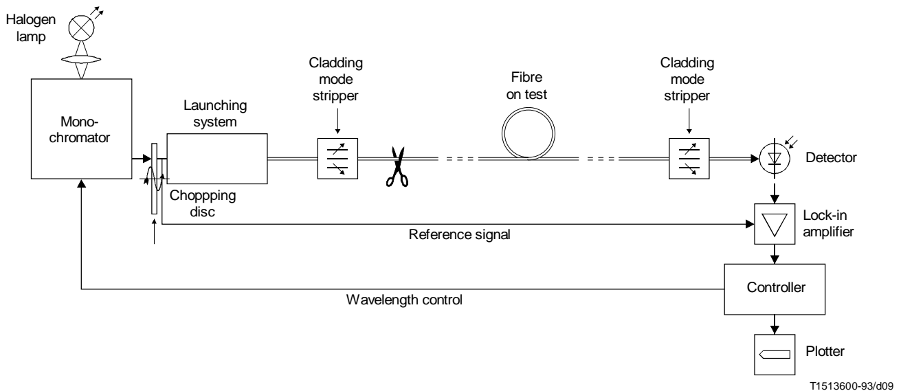
FIGURE B.8/G.651
