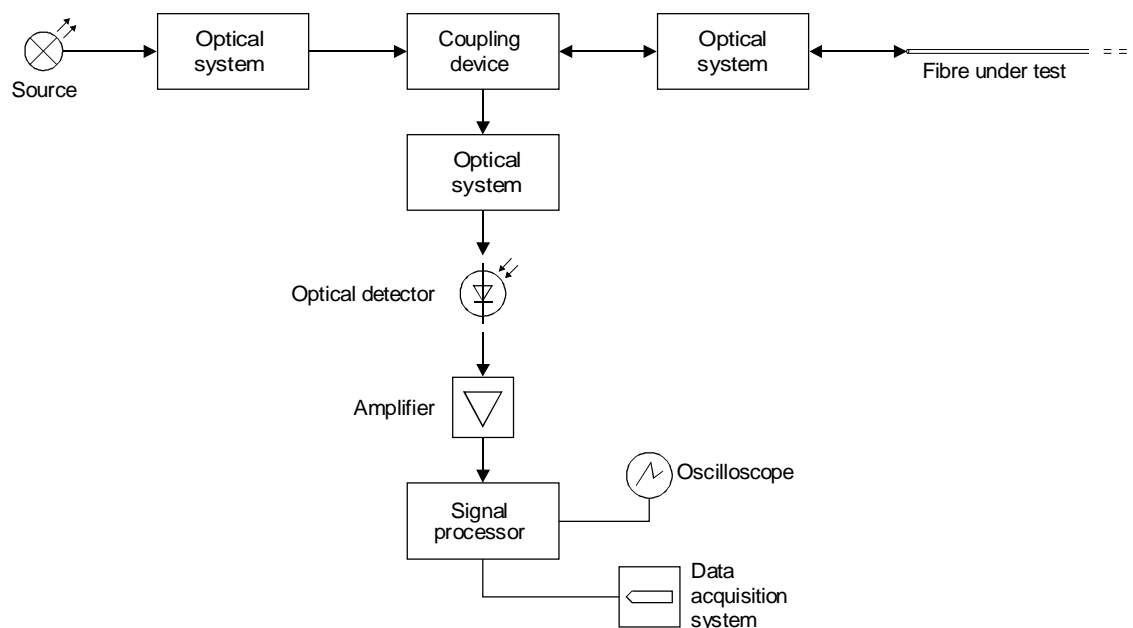
a) Scheme of apparatus
