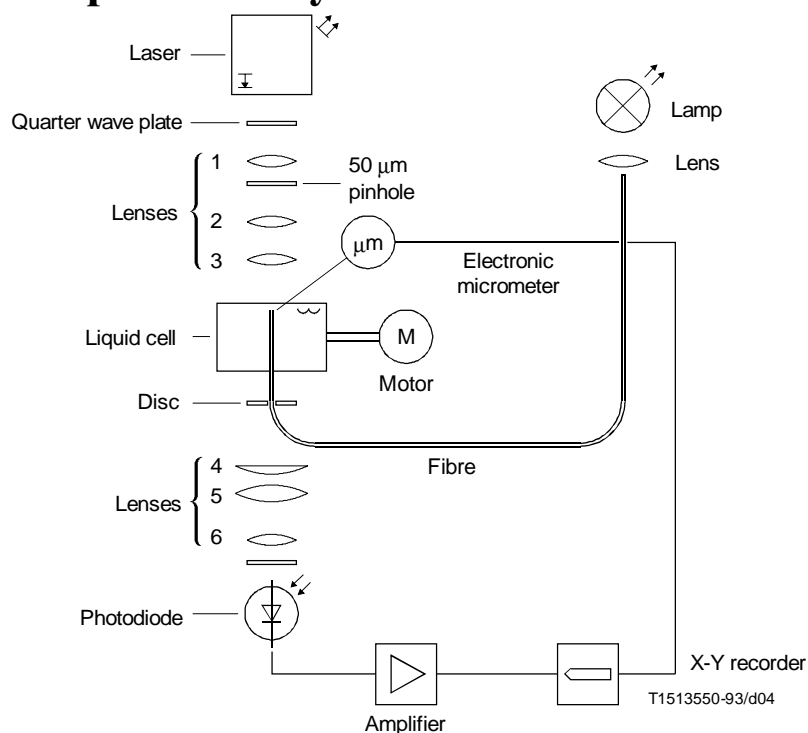
FIGURE B.3/G.651
