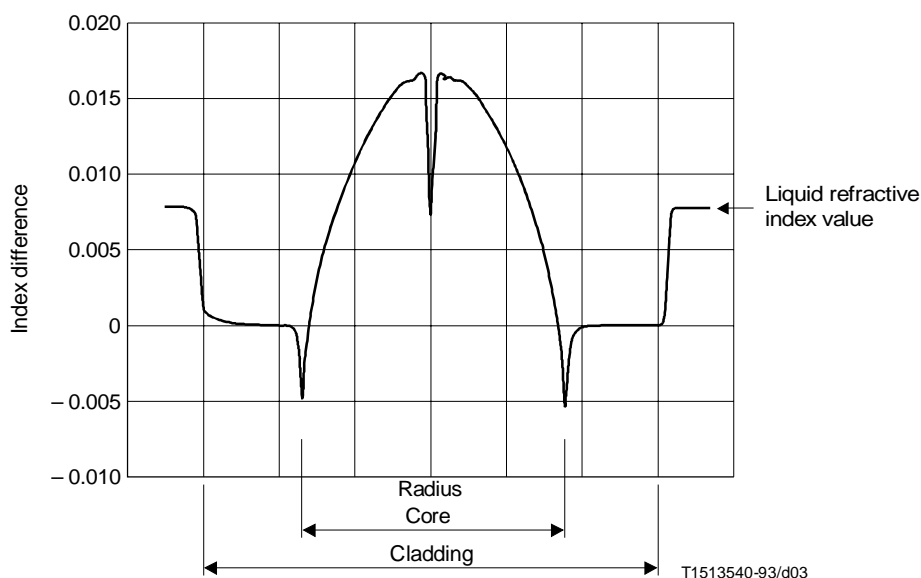
FIGURE B.2/G.651
