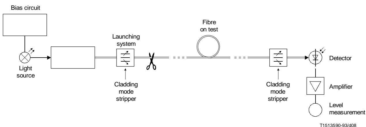
FIGURE B.7/G.651
