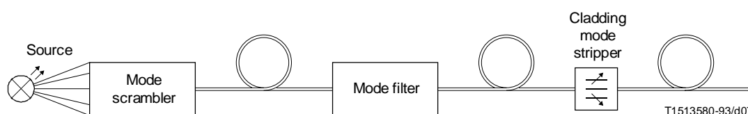
FIGURE B.6/G.651
