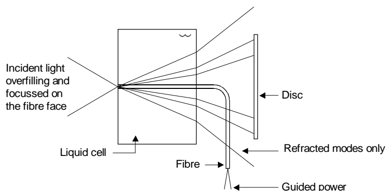
a) Refracted near-field technique – Schematic diagram
