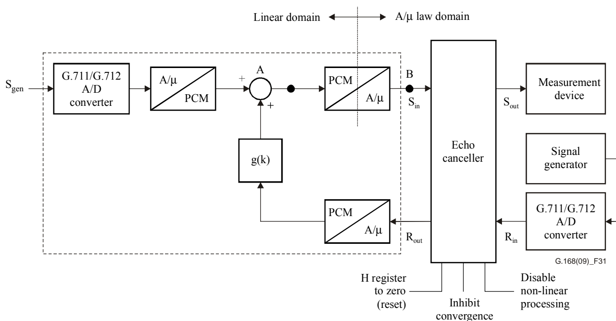
Figure 32 – Test configuration for S_{in} PCM offset test
