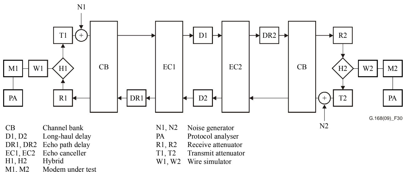
Figure 31 – Test No. 14 configuration
