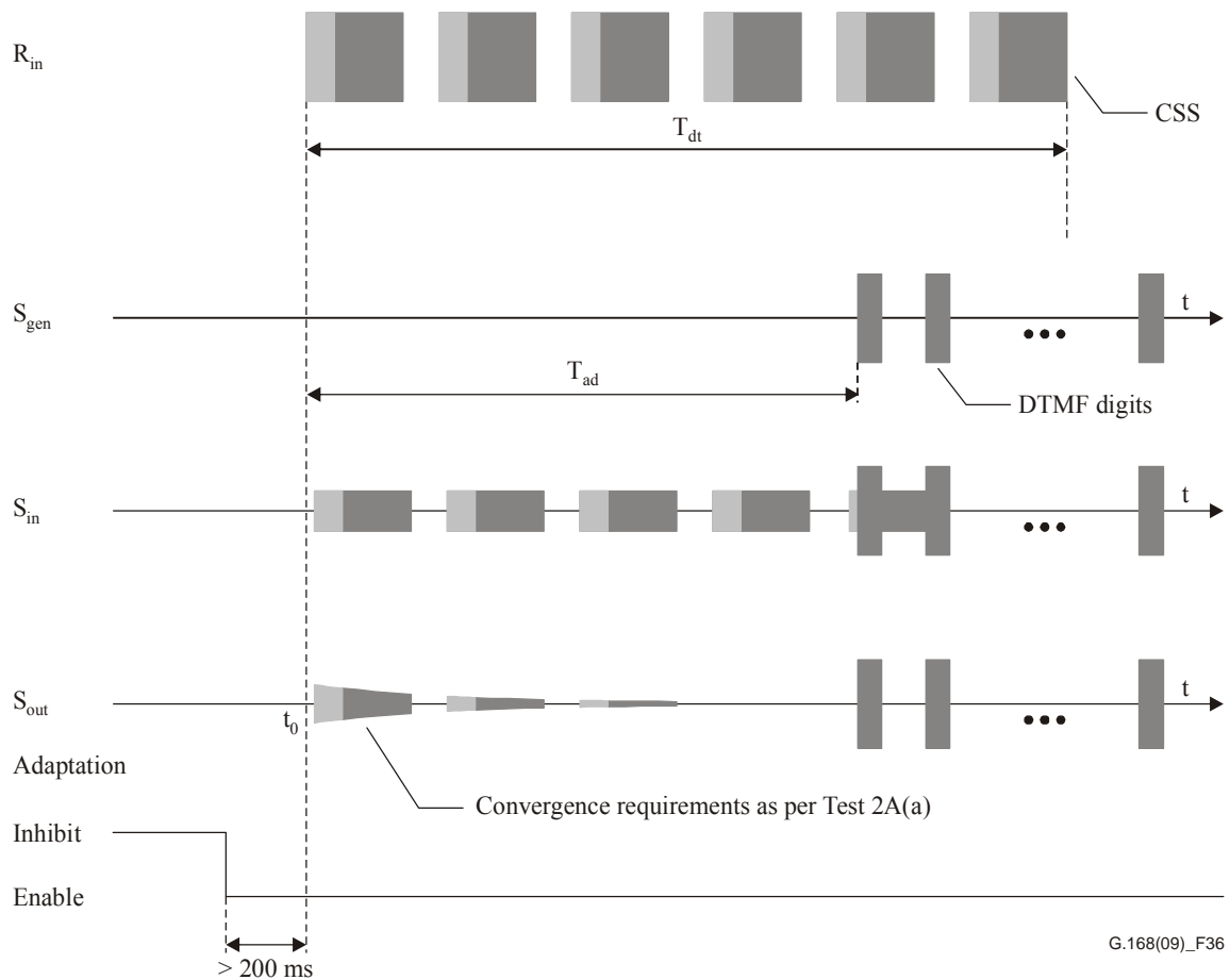
Figure 37 – Illustration of requirements for DTMF transparency in the presence of CSS
