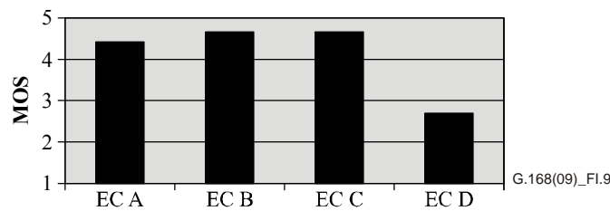
Figure I.9 – Results from talking and listening tests , MOS, disturbance caused by audible switching, digital echo path, ERL 6 dB, background noise –55 dBm0, NLP enabled
