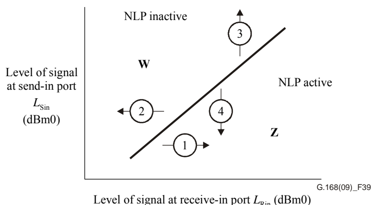
Figure 40 – NLP operating regions
