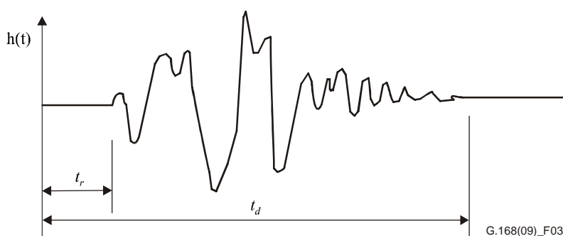
Figure 3 – Example of an impulse response of an echo path
