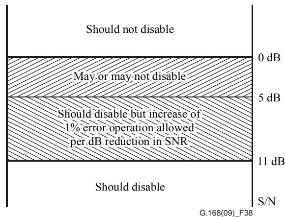
Figure 39 – Guardband and noise tolerance requirements
