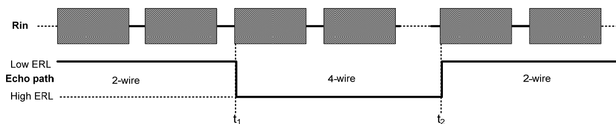
Figure 21b – Test No. 5B signal and timing relationships for low-high-low ERL transitions
