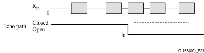
Figure 21a – Test No. 5A signal and time relationships
