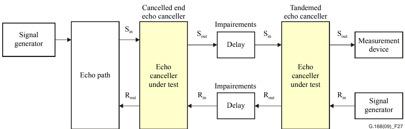
Figure 28 – Test No. 11 configuration
