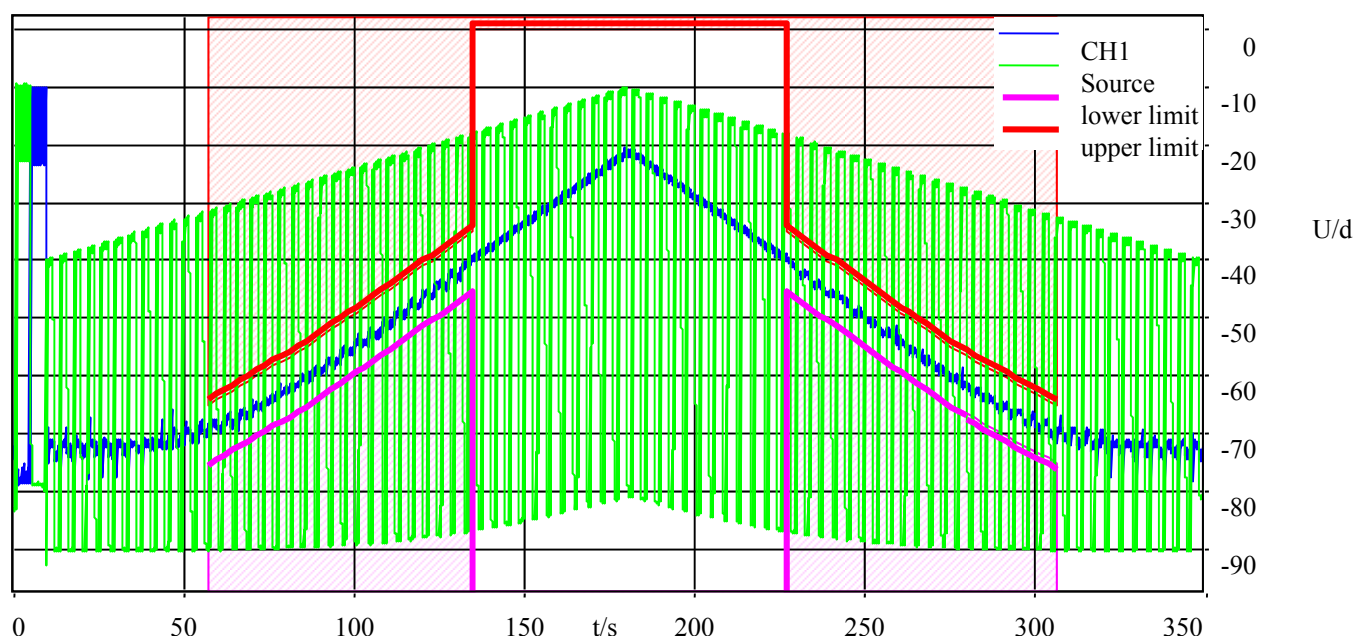
Figure 23b – Dynamic comfort noise level matching at 15 dB ERL
