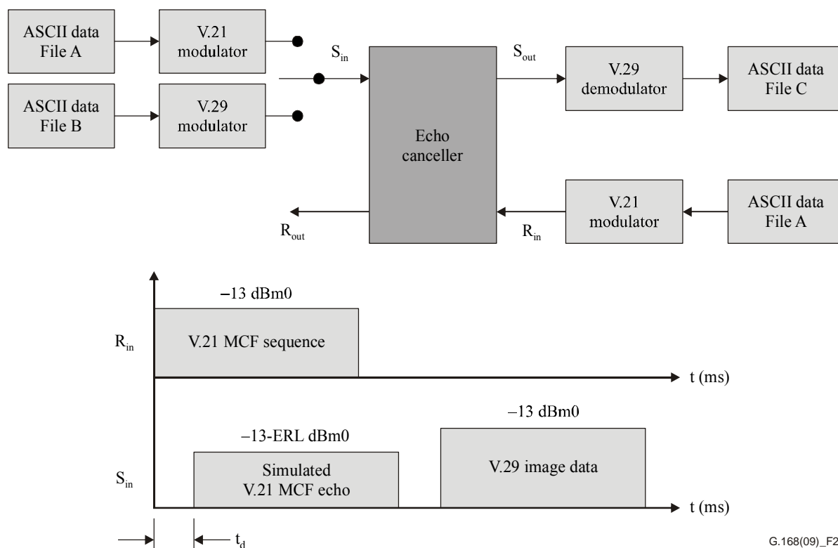
Figure 27 – Cancellation operation during page transmission and page breaks
