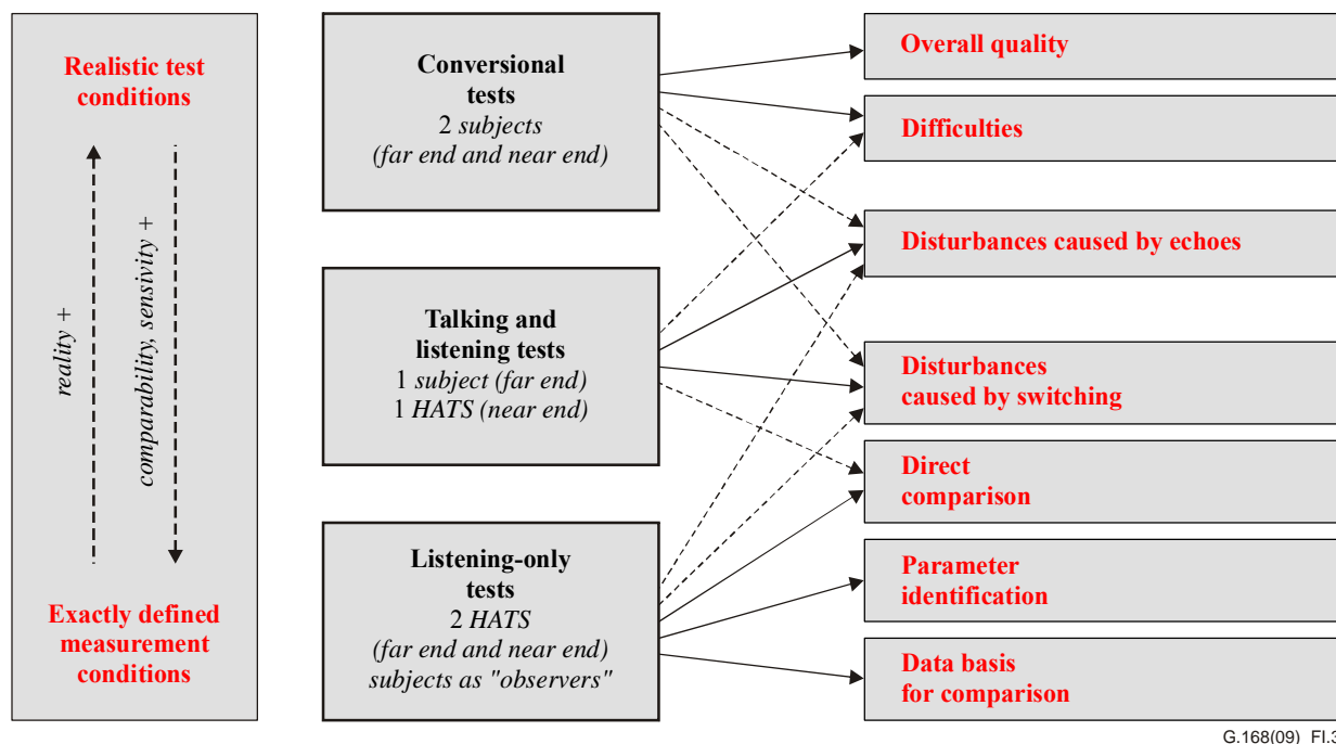
Figure I.3 – Structure of subjective test procedures for speech echo cancellers and a selection of parameters
