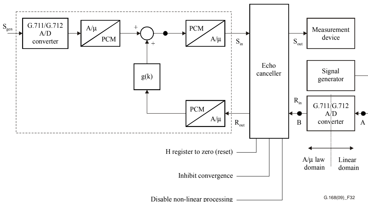
Figure 33 – Test configuration for R_{in} PCM offset test
