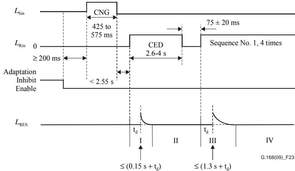
Figure 24 – Test No. 10A signal and time relationships
