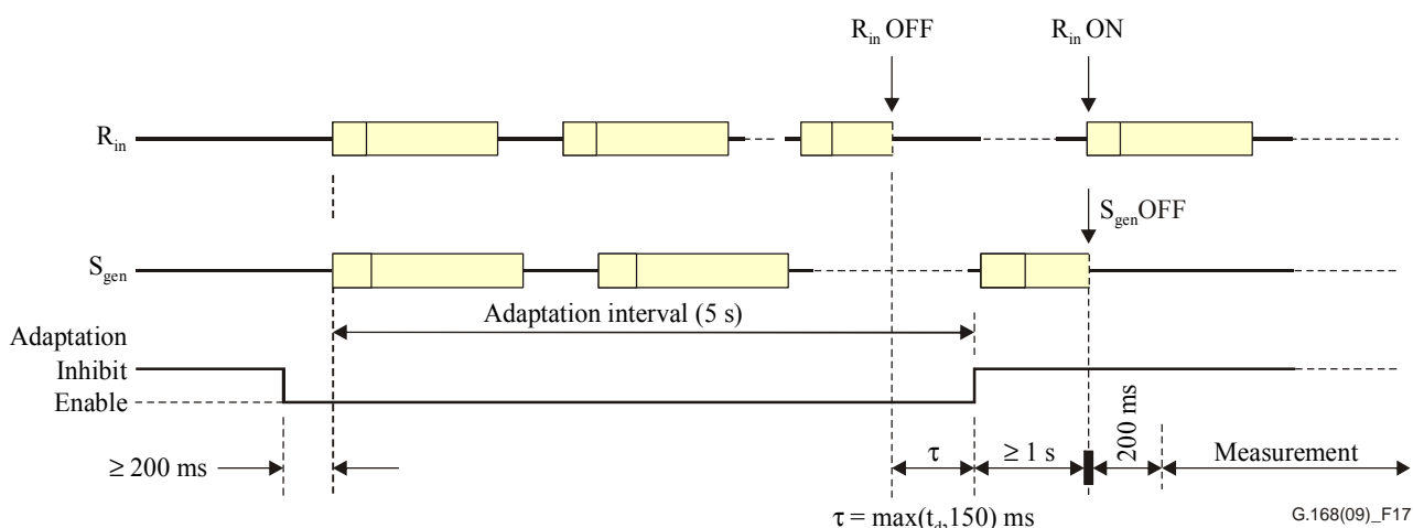
Figure 17 – Test No. 3A signal and time relationships
