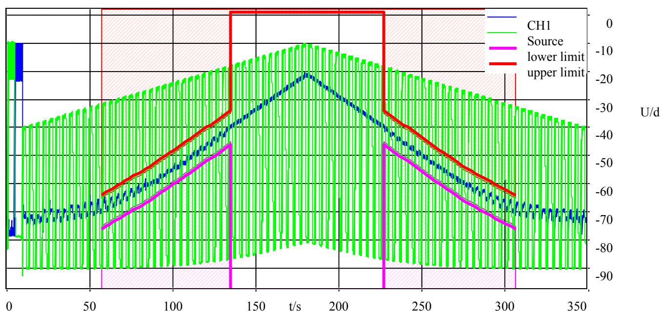
Figure 23c – Dynamic comfort noise level matching at 6 dB ERL
