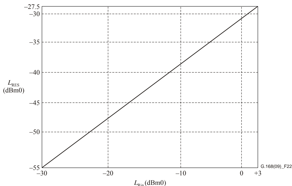
Figure 22 – Performance requirements for Test No. 7
