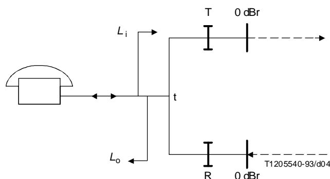
FIGURE C.1/G.121 Relation between relative levels and R- and T-pads
