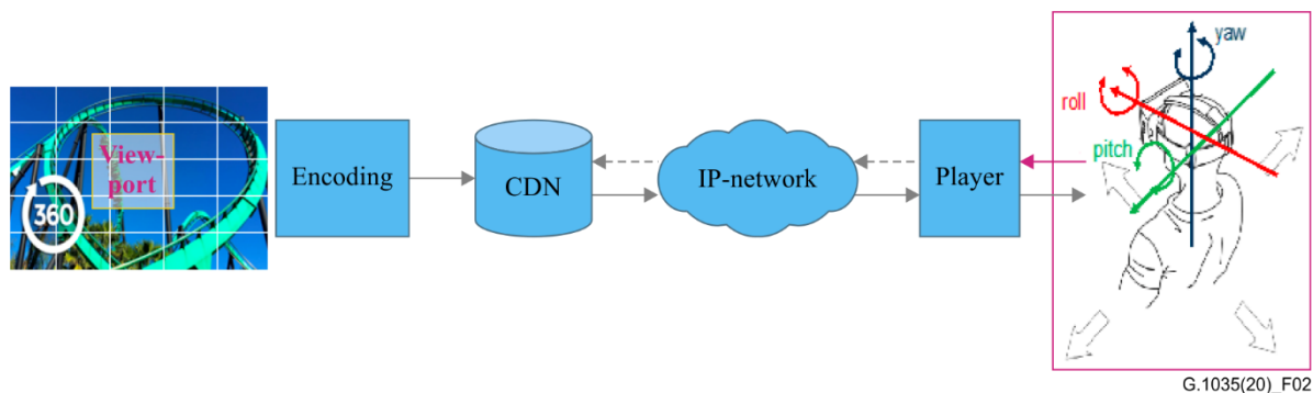
Figure 2 – Tile-based adaptive streaming – behavior dependent
