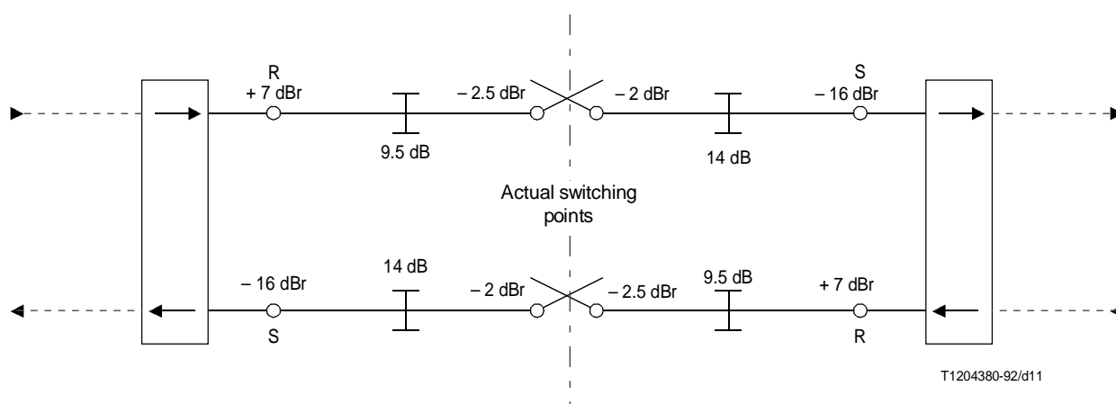
FIGURE A.4-6/G.100 Example showing a (simplified) representation of a transit connection in an international exchange, actual arrangement
