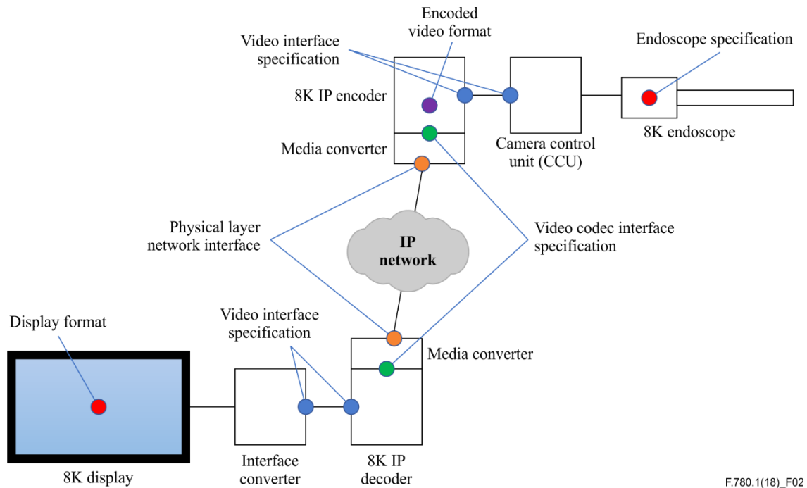
Figure 2 – Typical remote UHD endoscope system using an IP network
