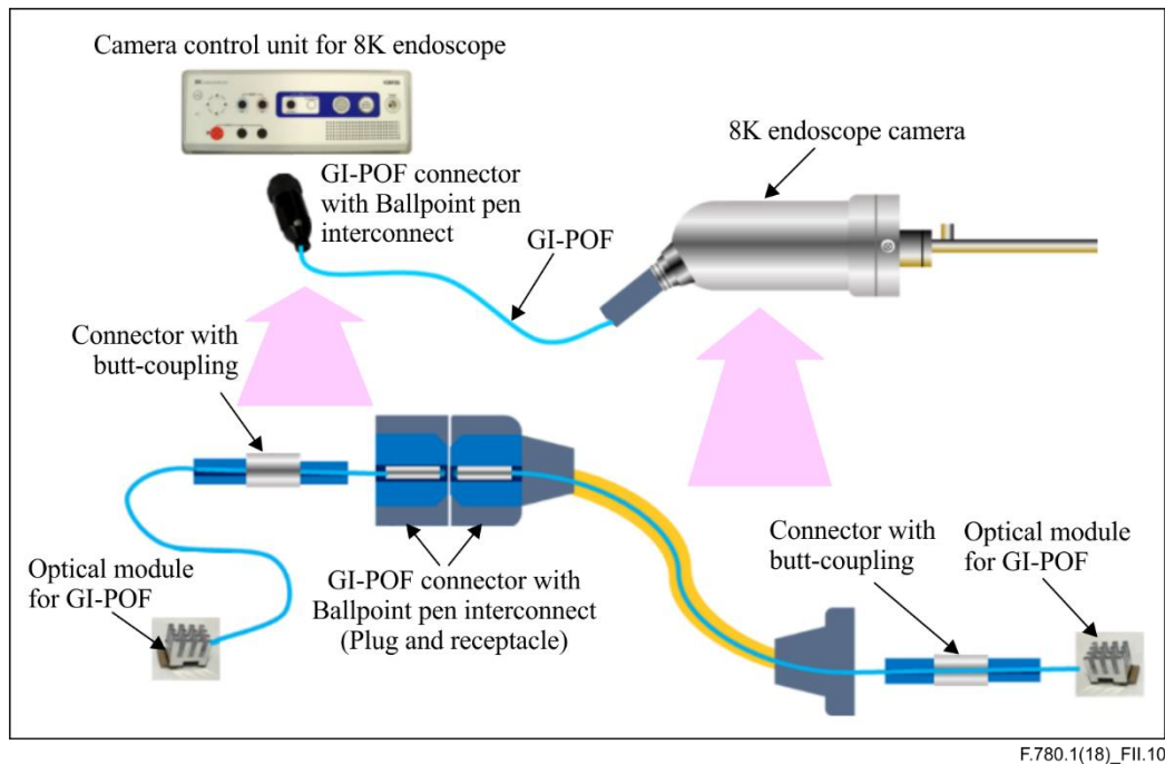
Figure II.10 – Graded index-plastic optical fibre (GI-POF) interface for 8K UHD video transmission
