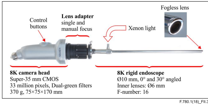
Figure II.3 – An example of a mass production model of the 8K UHD endoscope
