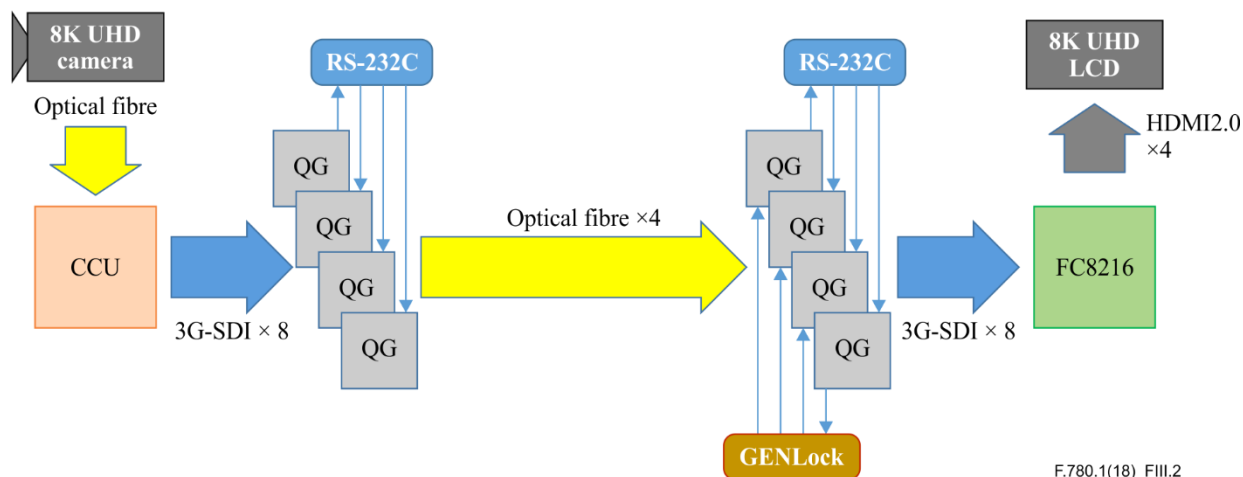
Figure III.2 – Connection between 8K UHD camera and 8K UHD LCD through the encoding / decoding transmission
