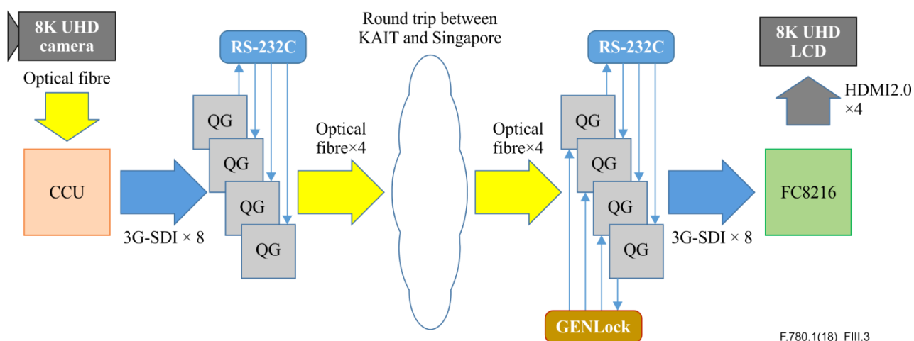
Figure III.3 – Connection between 8K UHD camera and 8K UHD LCD by way of a round trip between Japan (KAIT) and Singapore
