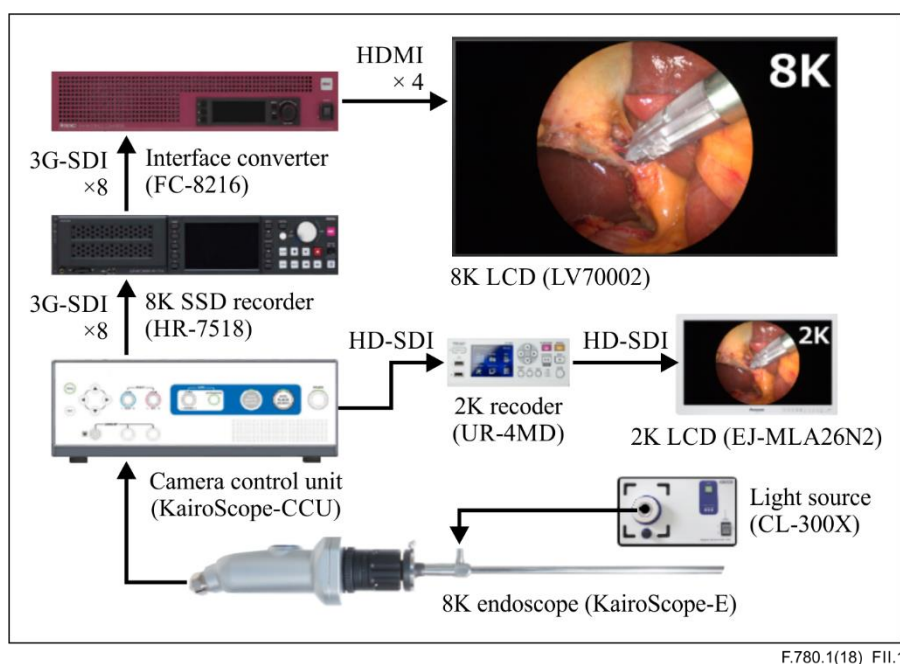
Figure II.1 – System configuration example of an 8K UHD endoscope
