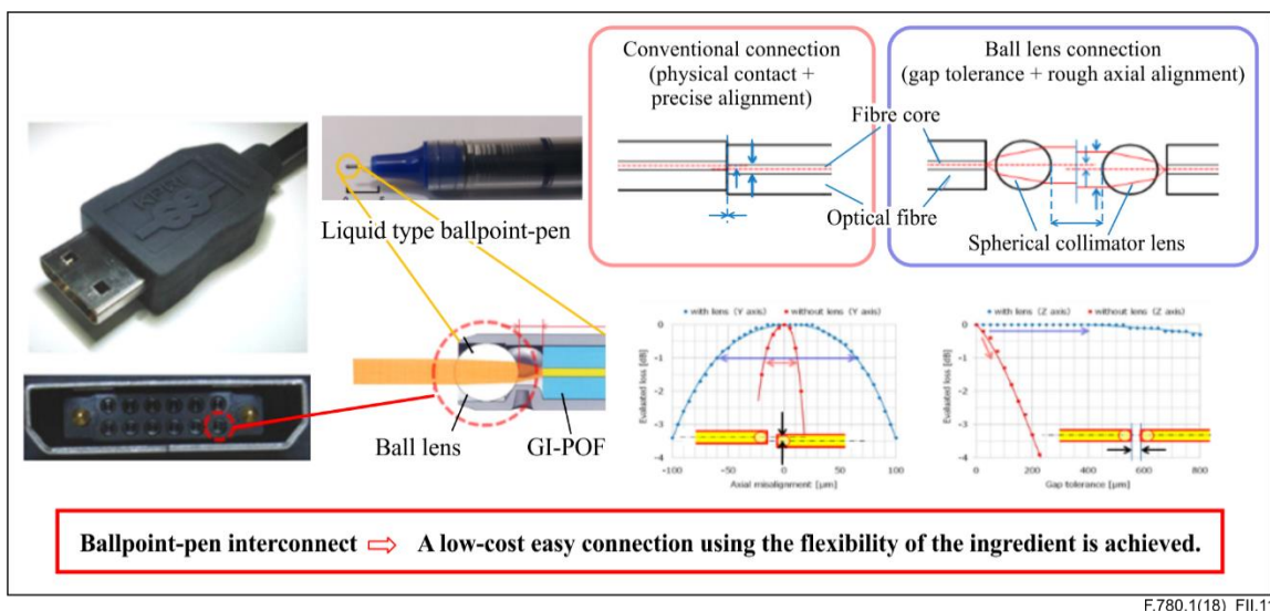
Figure II.11 – Ballpoint-pen interconnection
