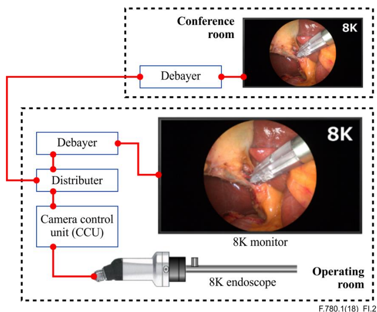
Figure I.2 – 8K endoscope system with teleconference (in-house)
