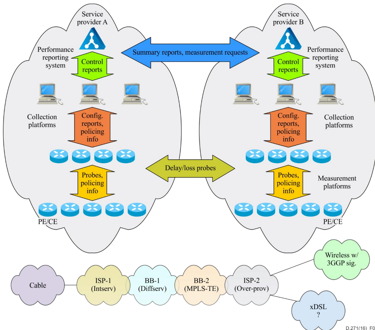
Figure 4 – QoS interworking accounting parameters
