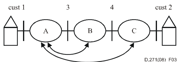
Figure 3 – Three administrations conduct a session through intersession (star organization)
