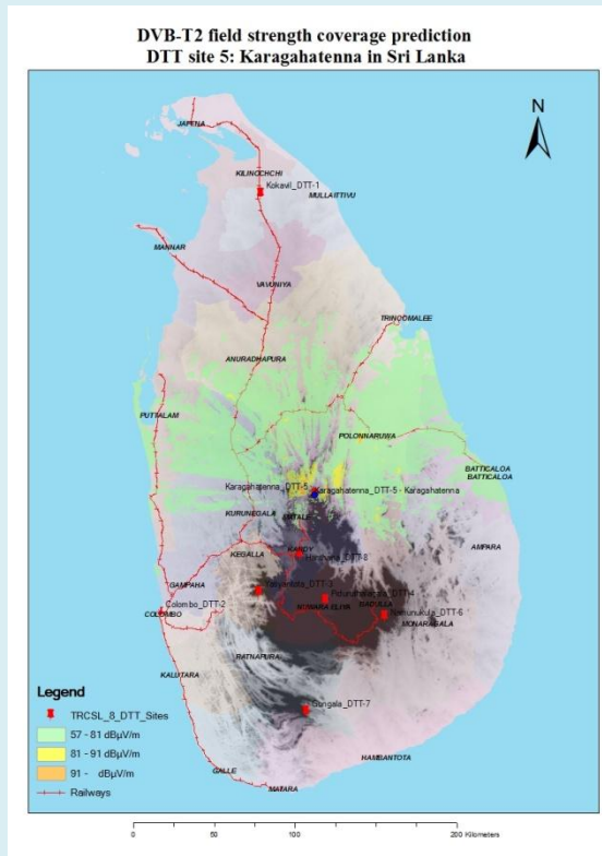
Figure 45: Karagahatenna DTTB Site FS coverage
