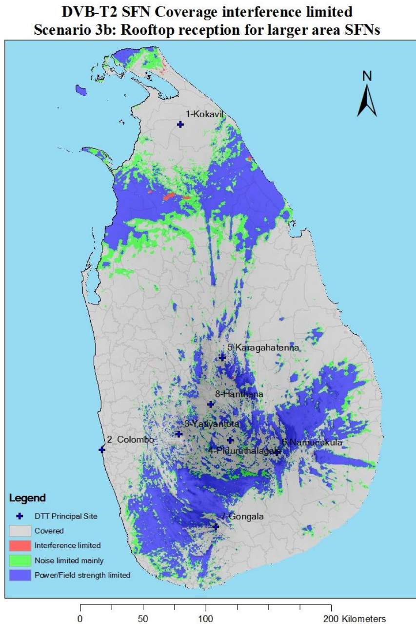
Figure 39: coverage interference limited under Scenario 3b (self interference occurs in power/field strength limited area)
