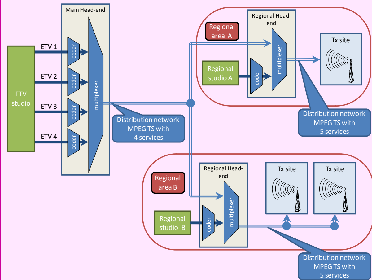
Figure 4.9: Example of network lay out with regional head-ends
