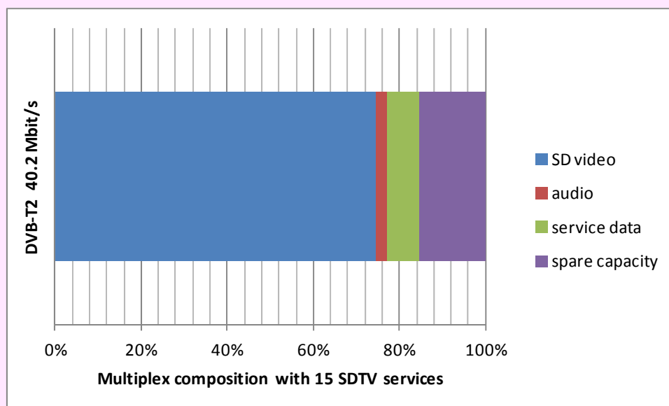
Figure 4.8: Example DVB-T2 multiplex compositions with 15 SDTV services
