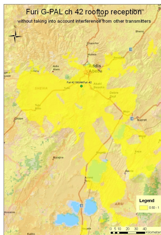
Figure 2.4: Coverage of B-PAL (ch 7) and G-PAL (ch 42) with rooftop reception
