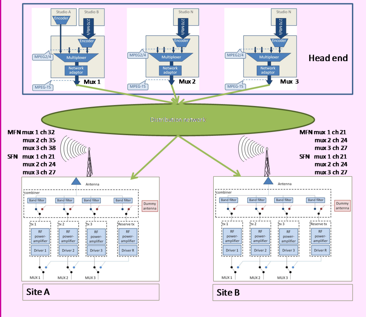
Figure 7-2: Example of a DTTB network consisting of a head end with three multiplexers and two sites
