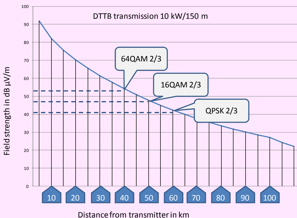
Figure A6-2: Example of digital TV coverage area with rooftop reception
