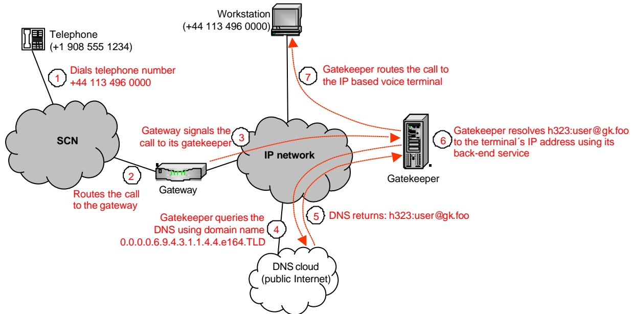
Figure 3 – Sample call flow from IP based network to switched circuit network
