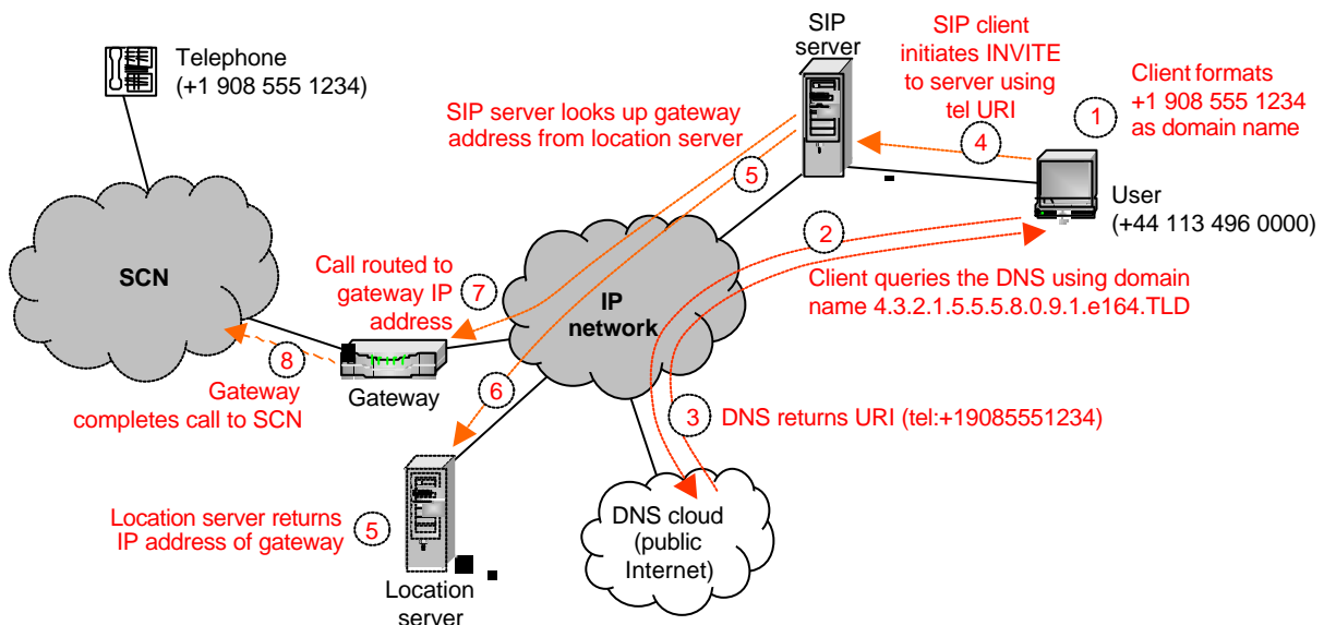
Figure A.2 – Typical call flows: IP to PSTN
