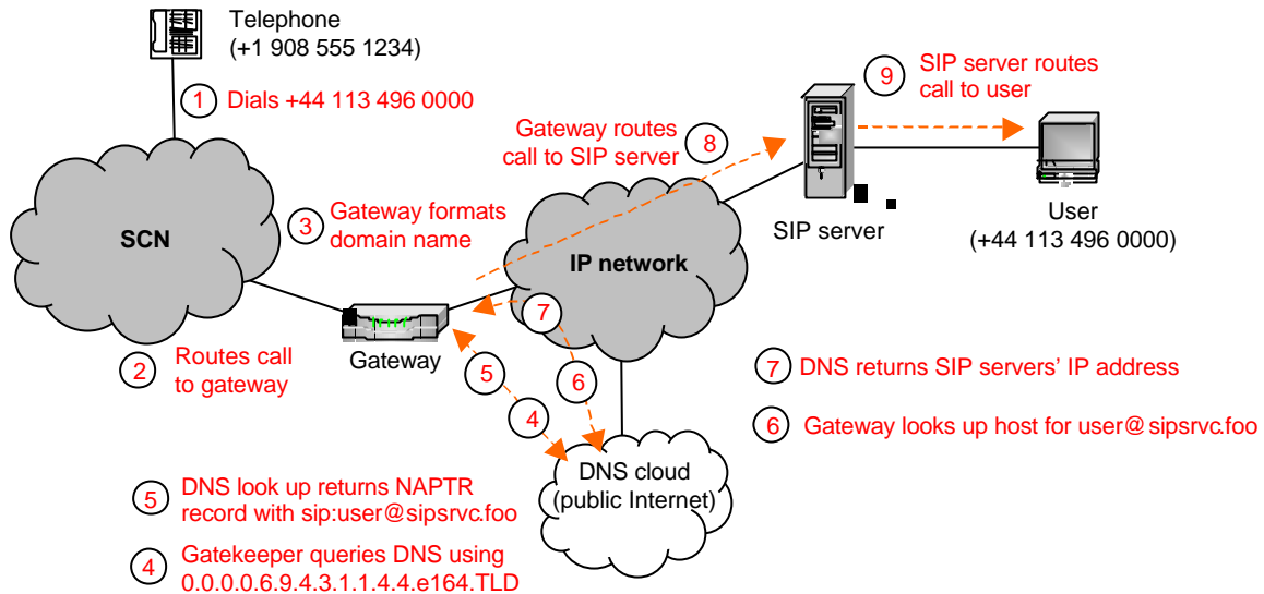
Figure A.1 – Typical call flows: PSTN to IP
