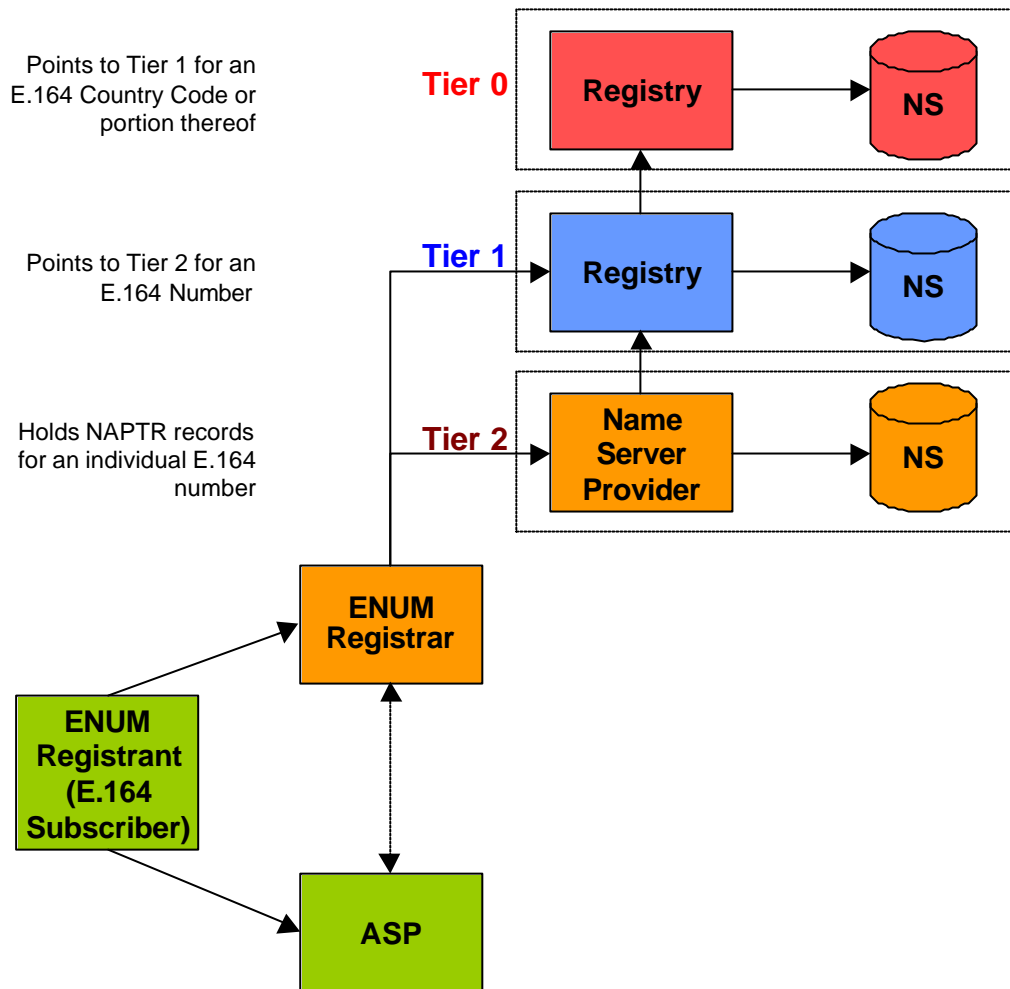
Figure 4 – Inserting E.164 numbers in DNS
