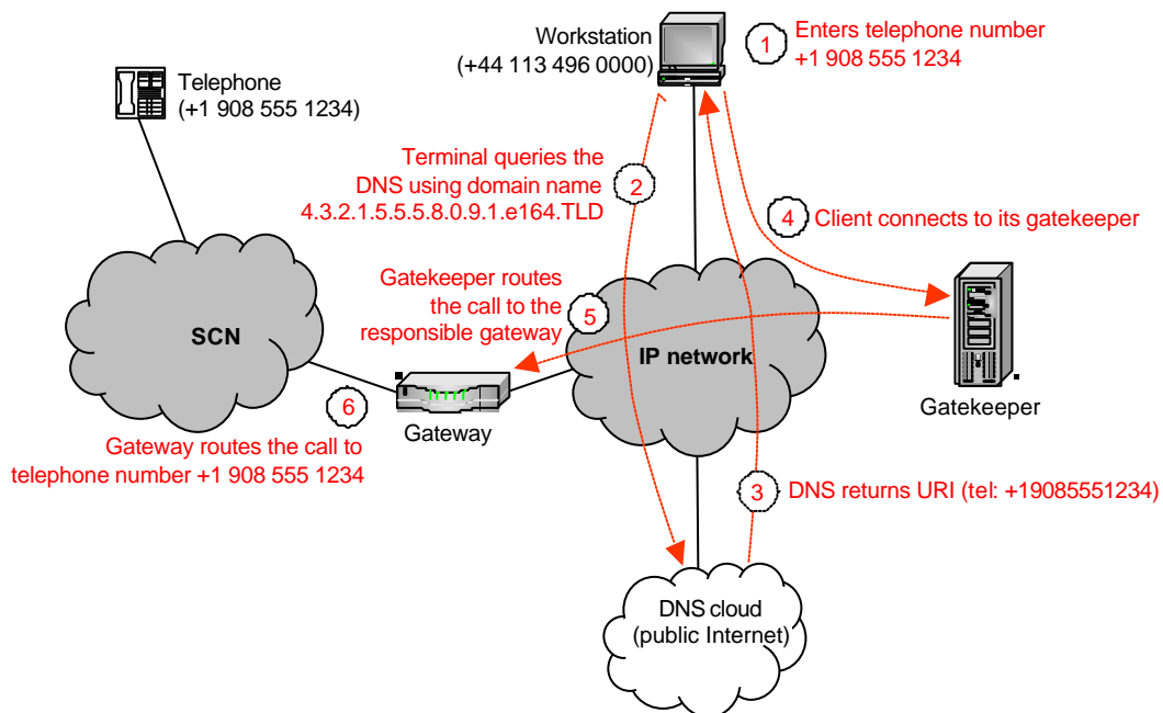
Figure 2 – Sample call flow from switched circuit network to IP based network
