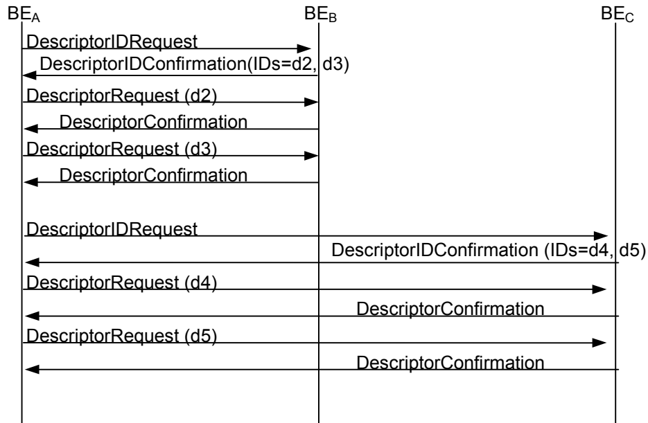
Figure G.8/H.225.0 - Example of Descriptor Exchange
