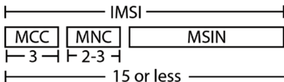
Figure 3.3. MCC, MNC, MSIN, and IMSI
