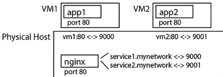
Figure 3.8. Microservice Architecture
