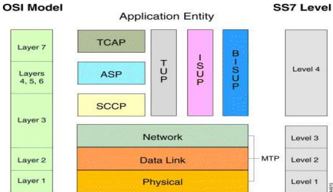
Figure A.1 The SS7 Protocol stack
