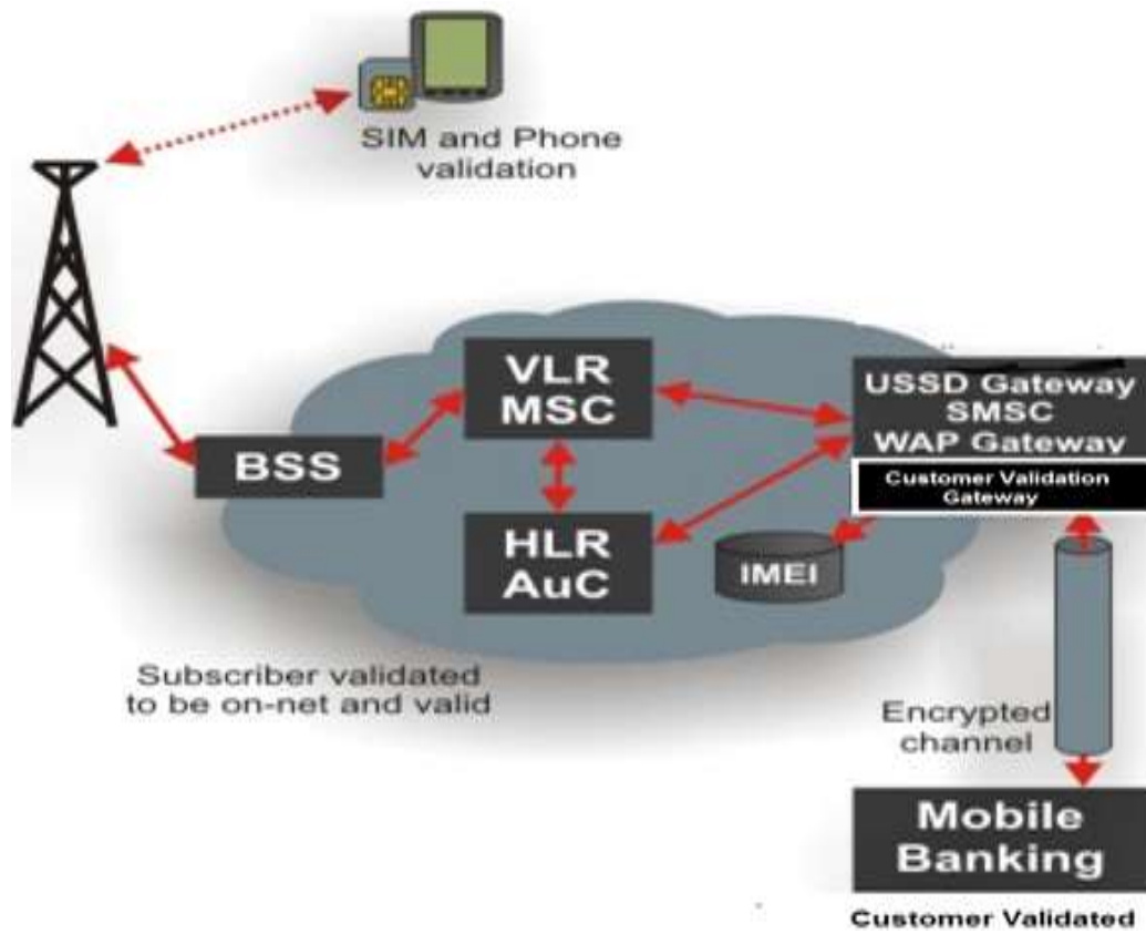
Figure 12 – An IMSI validation gateway
