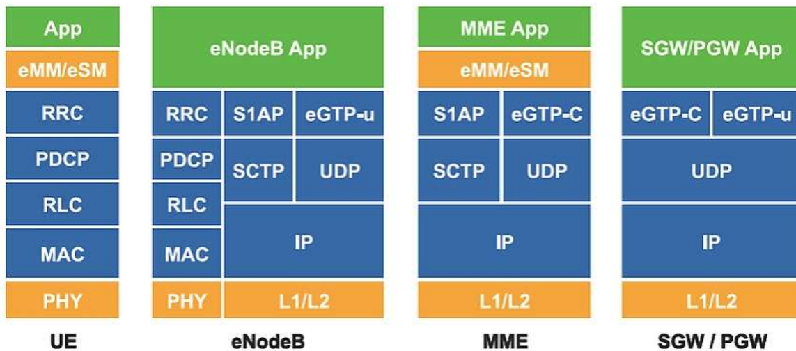
Figure A.2 - LTE (Diameter) protocol stack
