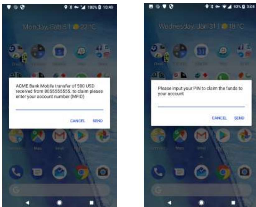
Figure 8 – Using USSD to socially engineer the user
