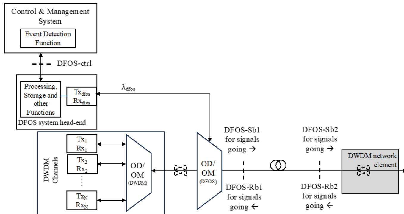
Figure 6-1 – Reference diagram of back-scattering type sensing. Out-of-band sensing wavelength, bi-directional DWDM transmission
