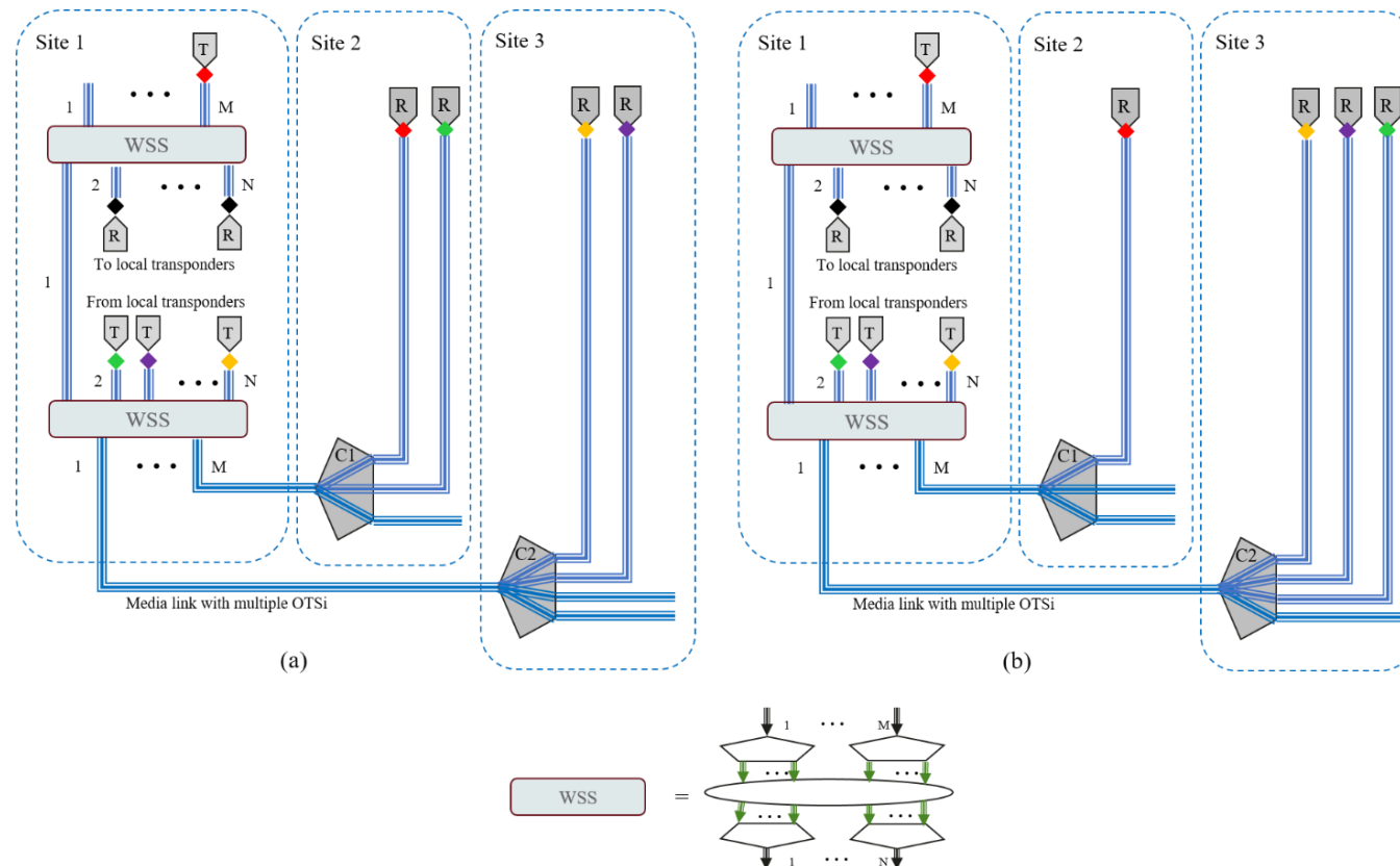
Figure III.5 - Optical one-hop connection and resource sharing features of metro aggregation ring network based on R-(LADD&WADD) in Appendix II.4.
