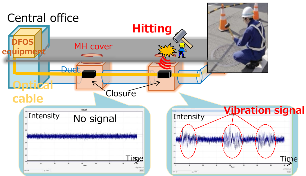
Cable route identification with DFOS
