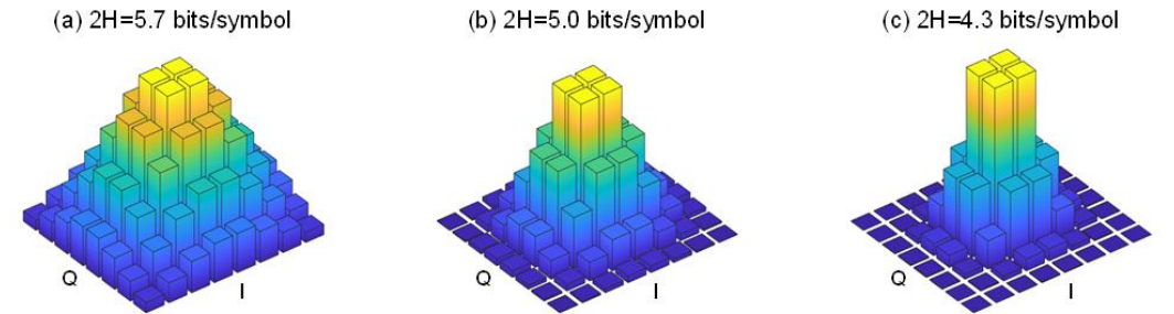
Figure 7-42 – Exemplary constellation distribution diagrams of PCS-64-QAM with entropies of (a) 5.7 bits, (b) 5.0 bits, and (c) 4.3 bits per complex symbol ([b-Liu2])
