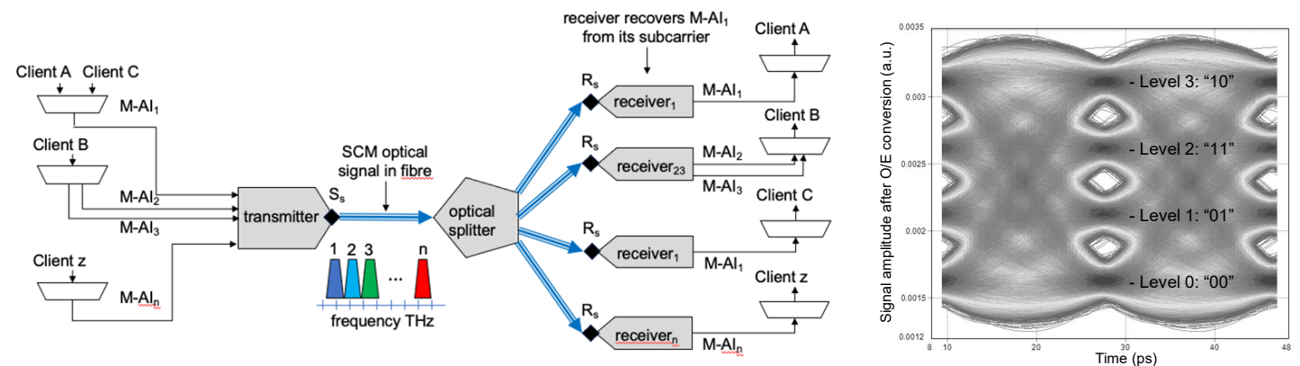
Figure 7-10 – An exemplary PAM4 eye diagram generated by an EML at 112 Gb/s
