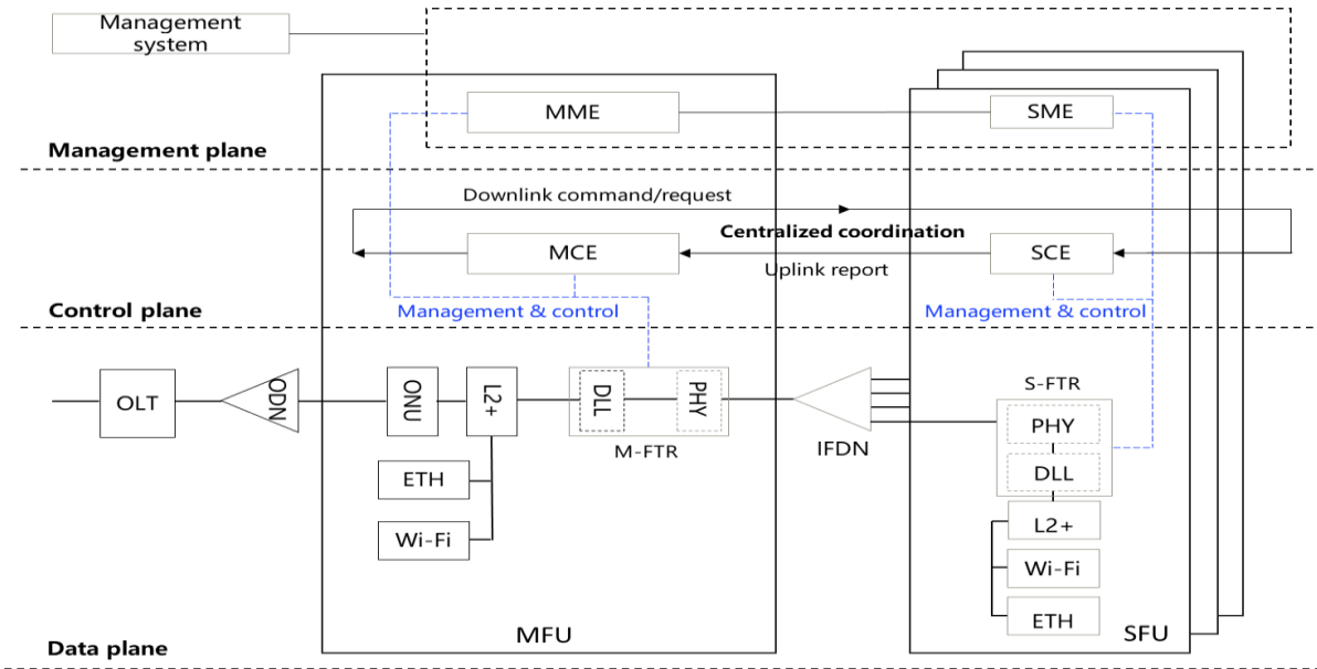
Functional framework of G.fin system
