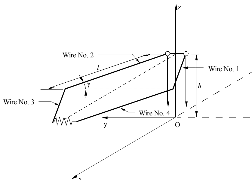
Horizontal rhombic antenna
