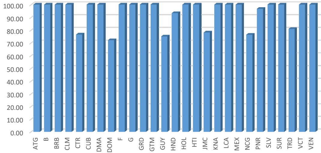
Final UHF iteration - Percentage of assignable channels (4dB margin), ignoring self-interference and interference to the wanted requirement
