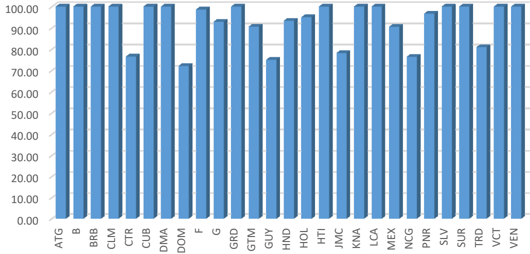
Iteration 40 - Percentage of assignable channels (4dB margin), ignoring self-interference and interference to the wanted requirement
