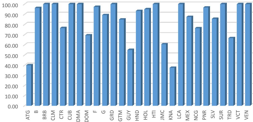
Iteration 39 - Percentage of assignable channels (4dB margin), ignoring self-interference and interference to the wanted requirement
