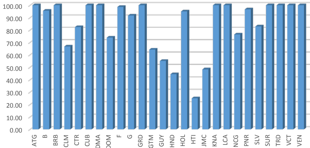
Iteration 38 - Percentage of assignable channels (4dB margin), ignoring self-interference and interference to the wanted requirement
